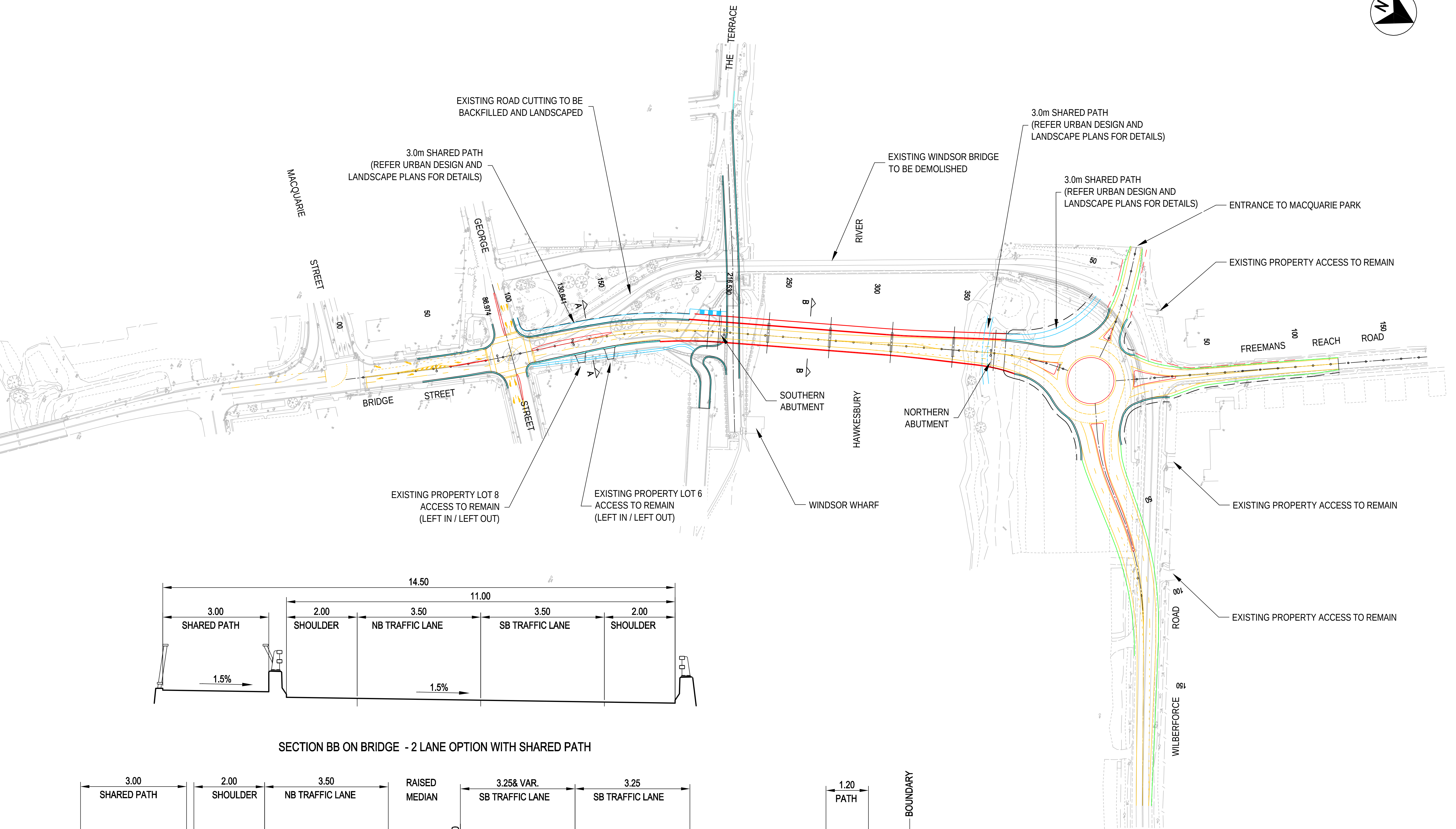
MR182 - BRIDGE ST WINDSOR WINDSOR BRIDGE REPLACEMENT -OPTION 5 GENERAL ARRANGEMENT PLAN SCALE 1:1000 (A1)
