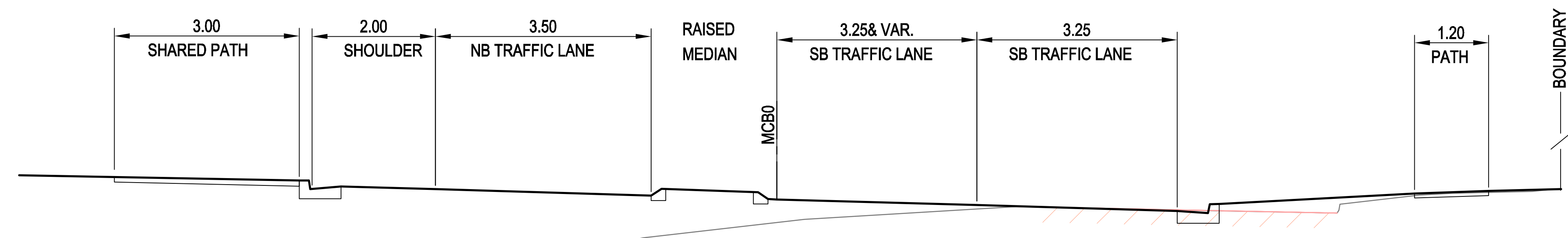
SECTION BB ON BRIDGE - 2 LANE OPTION WITH SHARED PATH
