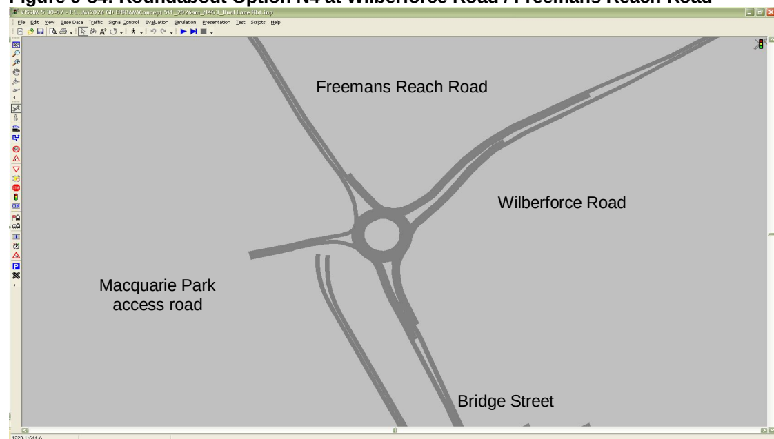
Figure 9-34: Roundabout Option N4 at Wilberforce Road / Freemans Reach Road
