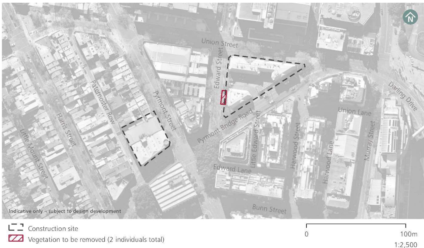
Figure 10. Site plan – Pyrmont Station construction sites
