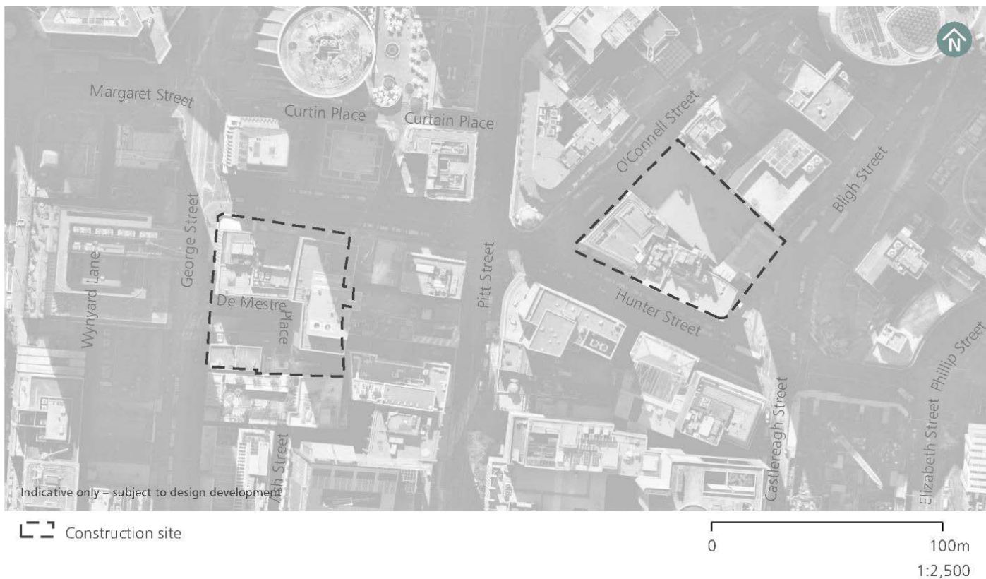
Figure 11. Site plan - Hunter Street Station (Sydney CBD) sites
