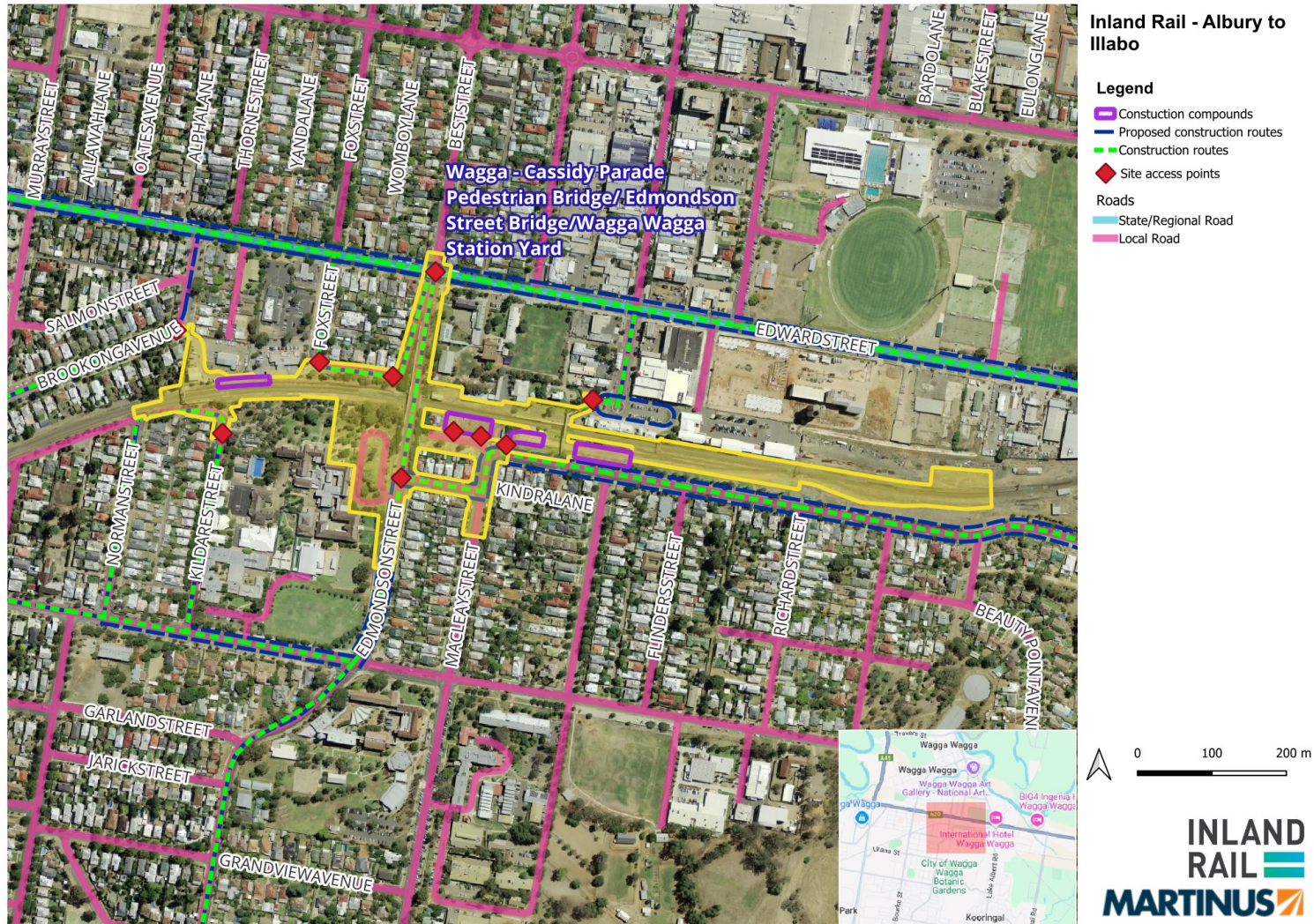
FIGURE 31 WAGGA WAGGA AND SURROUNDS CONSTRUCTION ROUTES
