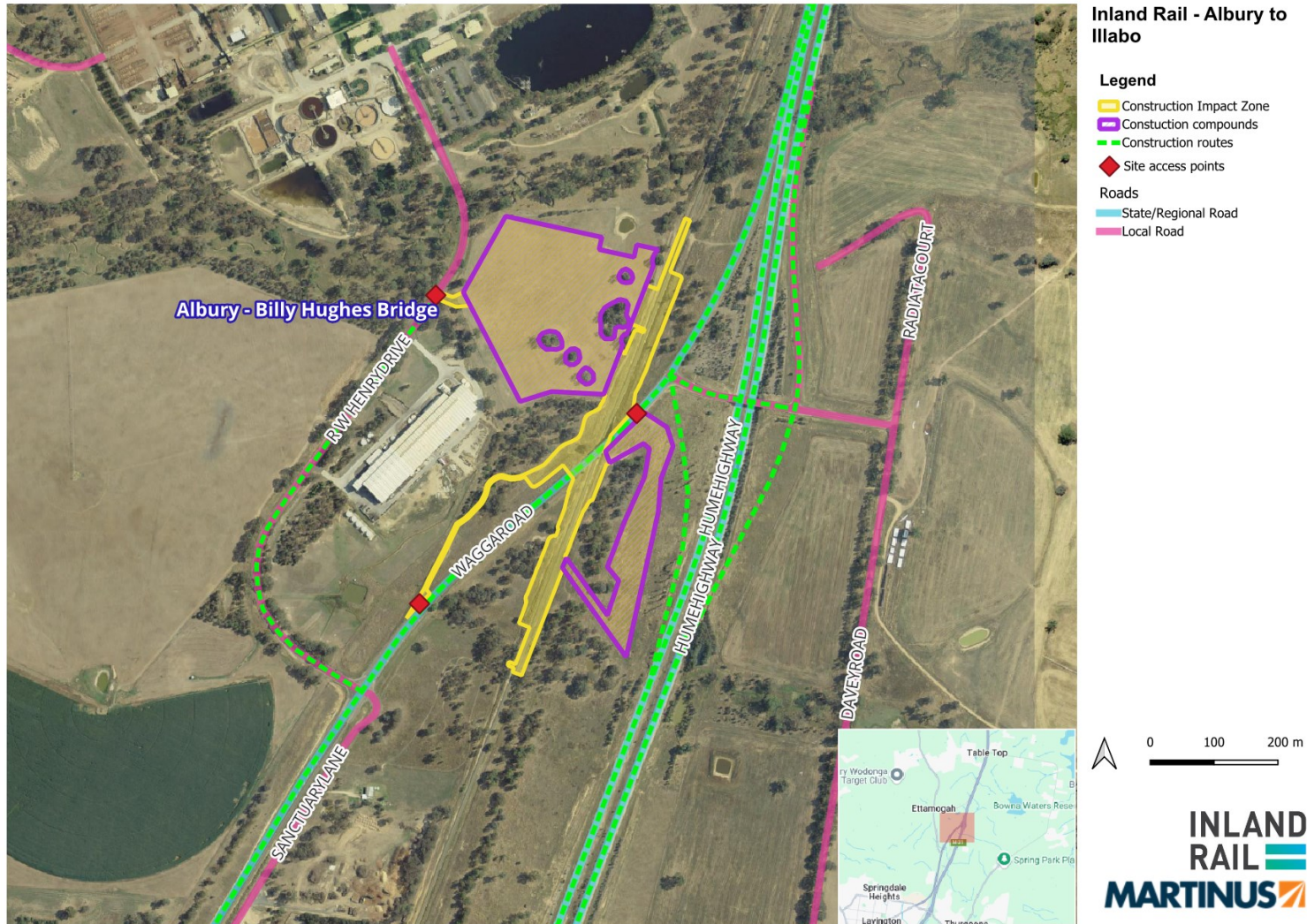
FIGURE 23 BILLY HUGHES BRIDGE CONSTRUCTION ROUTES
