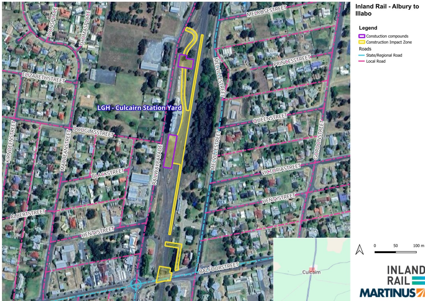
FIGURE 5 STATE, REGIONAL AND LOCAL ROADS CULCAIRN STATION YARD
