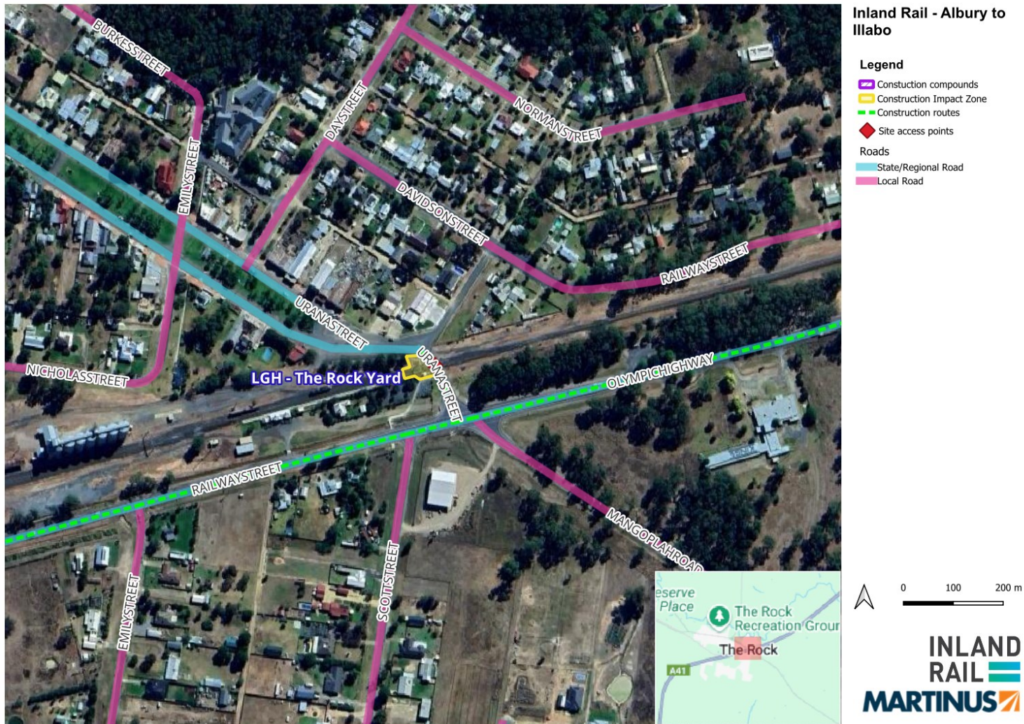
FIGURE 28 THE ROCK CONSTRUCTION ROUTES
