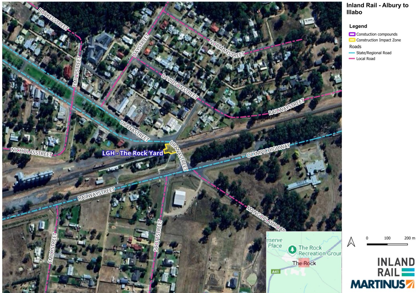
FIGURE 8 STATE, REGIONAL AND LOCAL ROADS THE ROCK
