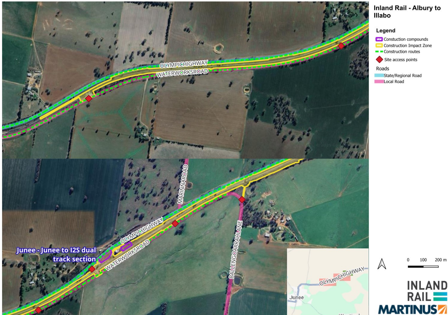
FIGURE 37 JUNE TO ILLABO CLEARANCES CONSTRUCTION ROUTES
