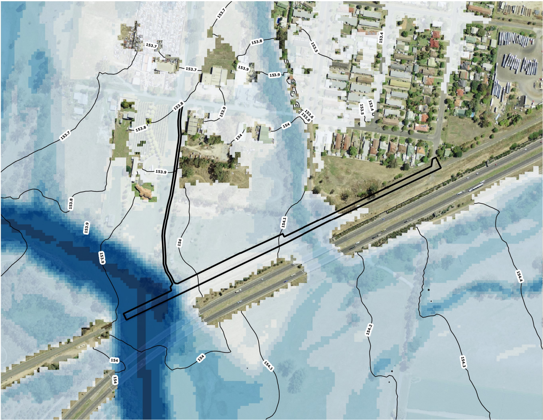
Figure A23 : 2% AEP Peak Flood Depth and Levels (Design Condition)
