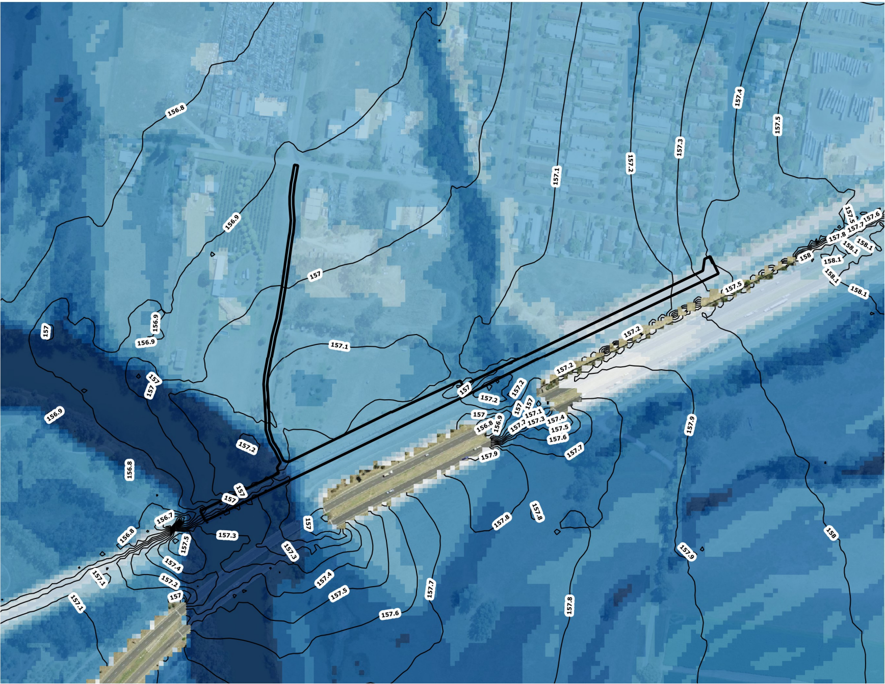
Figure A7 : PMF Peak Flood Depth and Levels (Existing Condition)
