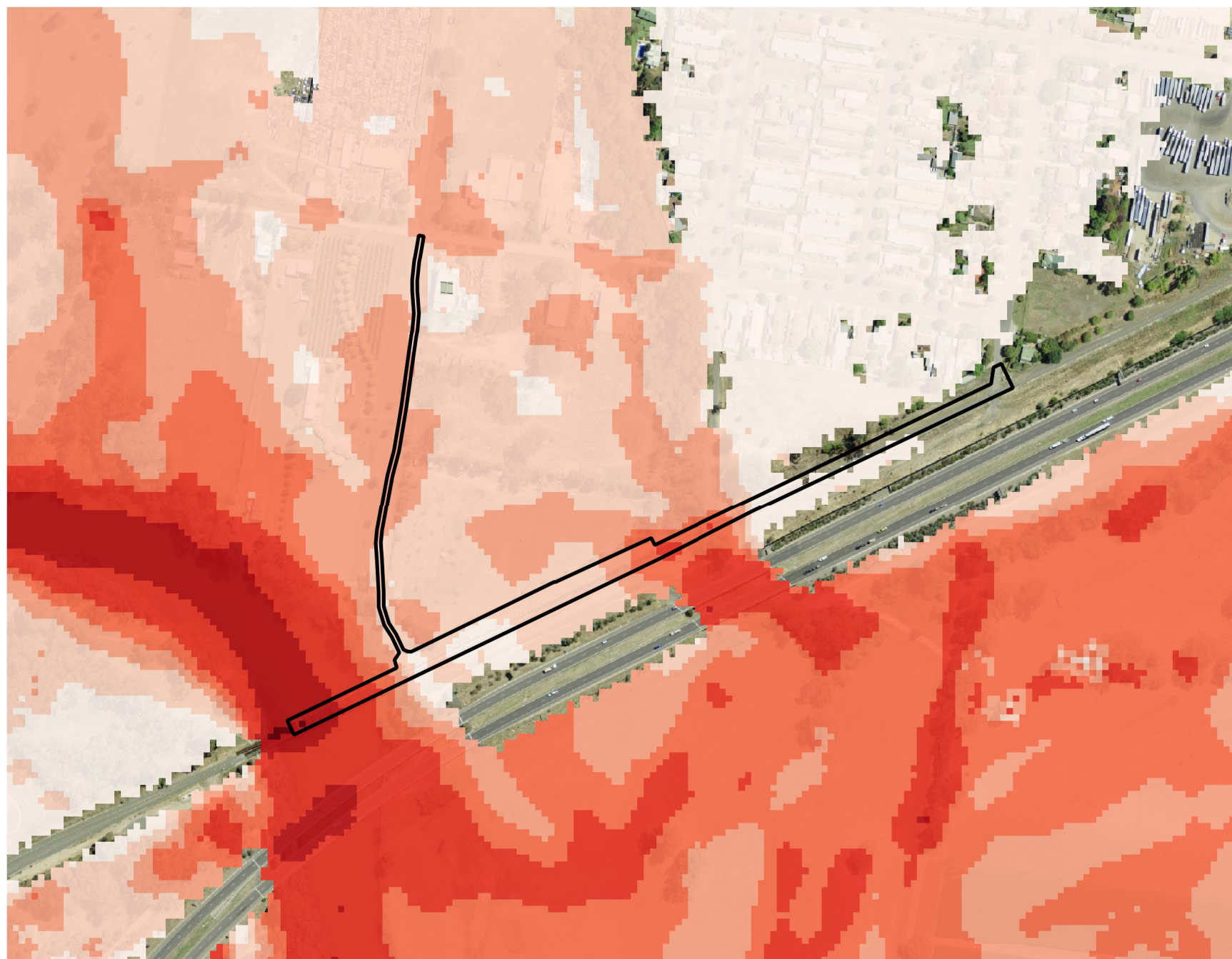
Murray River Bridge - Inland Rail (A2P) - DDR Stage Figure A65 : 1% AEP Peak Flood Velocity (Blockage Assessment)
