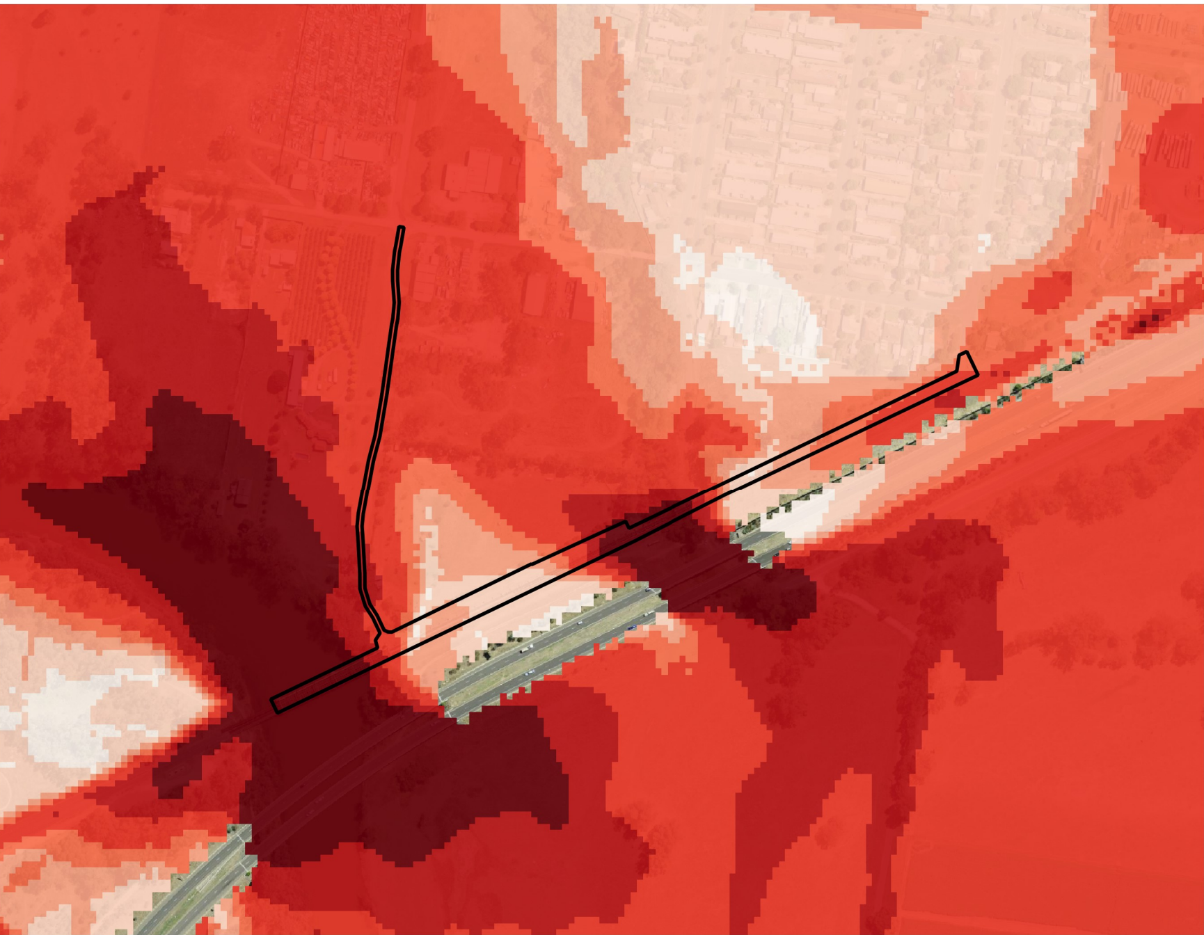
Murray River Bridge - Inland Rail (A2P) - DDR Stage Figure A14 : PMF Peak Flood Velocity (Existing Condition)
