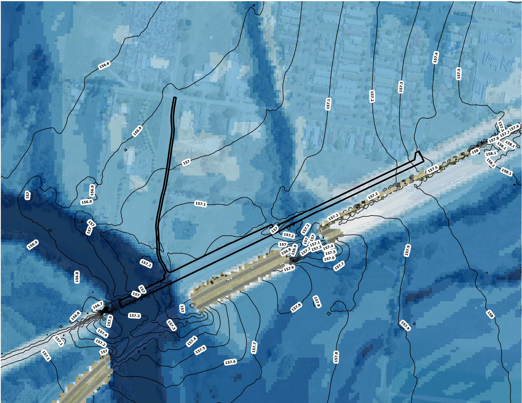
Figure A28 : PMF Peak Flood Depth and Levels (Design Condition)
