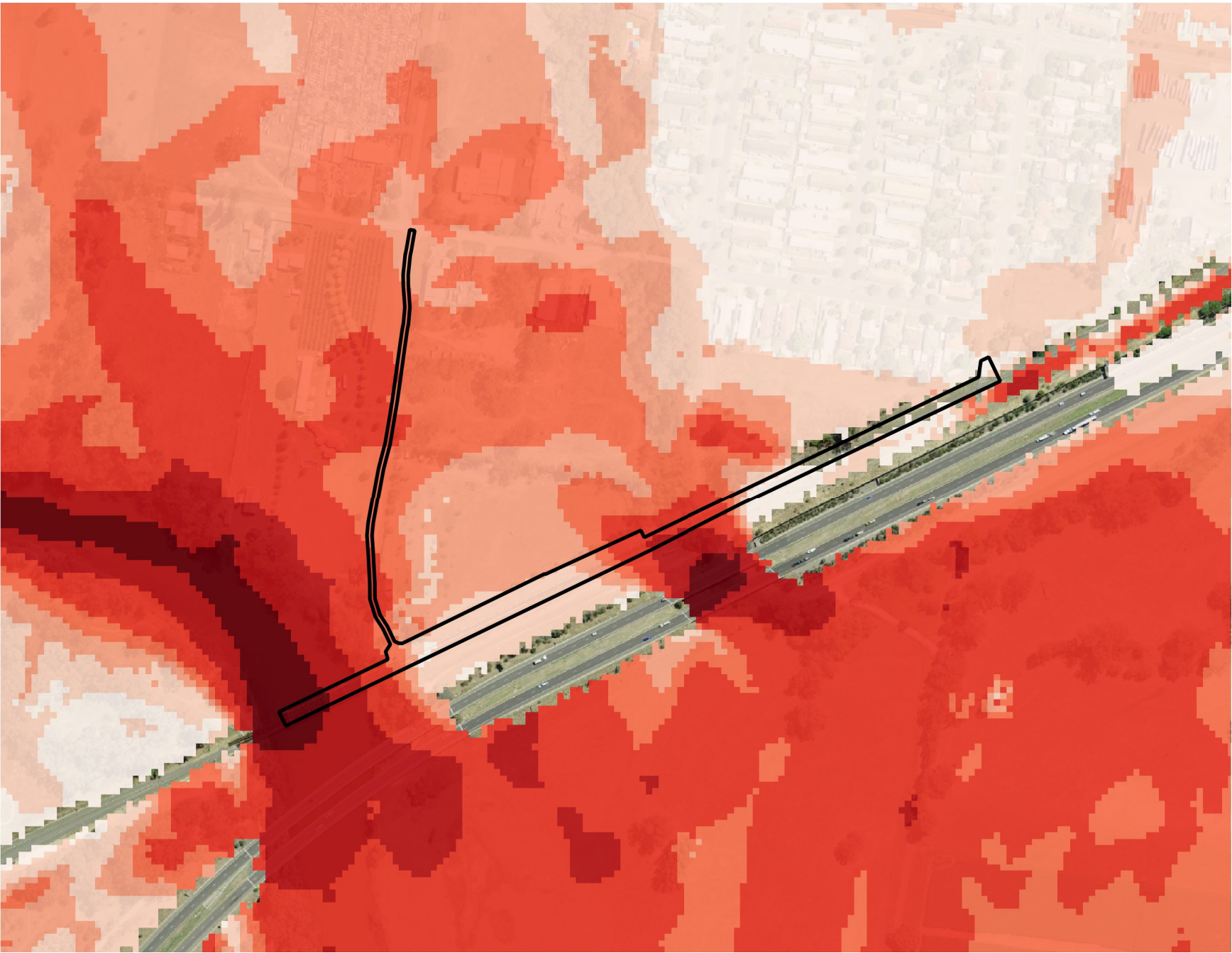
Figure A12 : 0.2% AEP (Climate Change Scenario 2) Peak Flood Velocity (Existing Condition)
