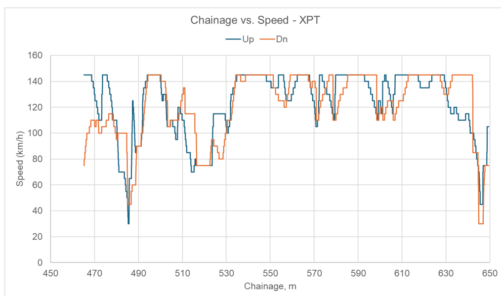
Figure 1 Chainage vs. speed – XPT trains
