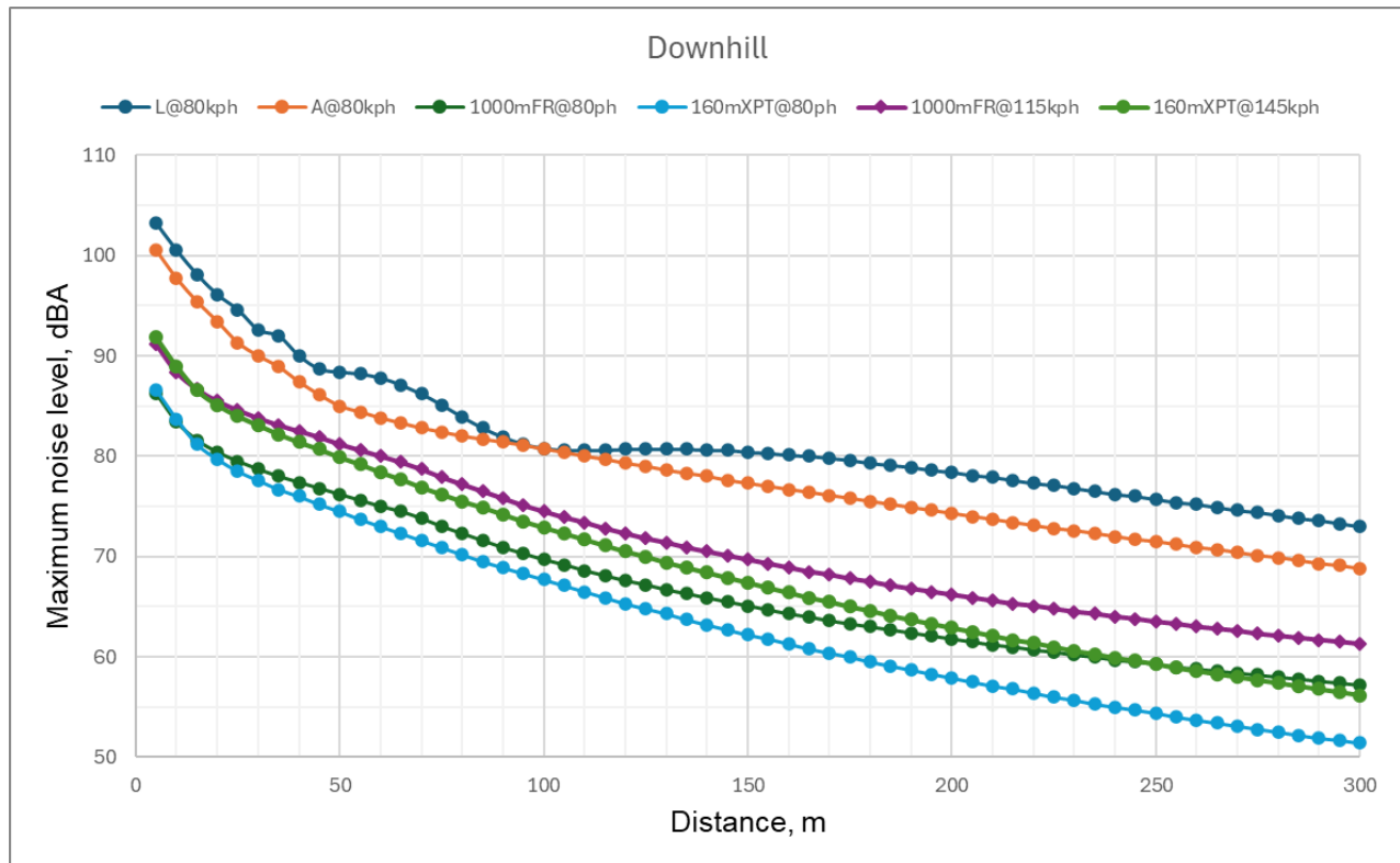
Figure 6 N2K propagation with distance, locomotives (downhill) and wagons
