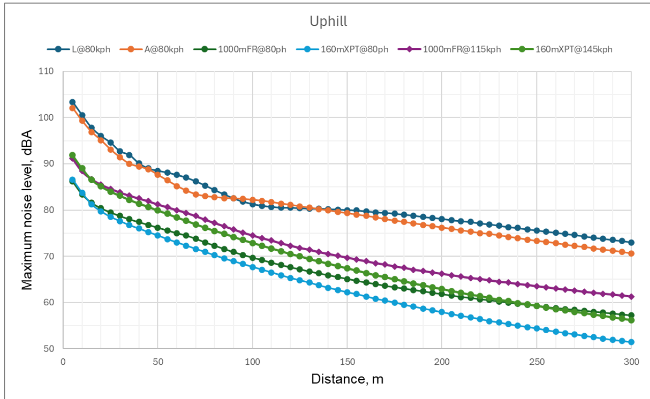
Figure 5 N2K propagation with distance, locomotives (uphill) and wagons
