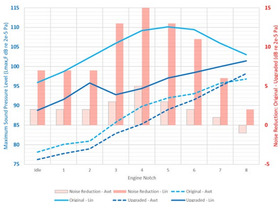
Figure 3 C Class noise emissions were reduced by 12-15dB at 15m from the track centreline in the loudest engine notches
