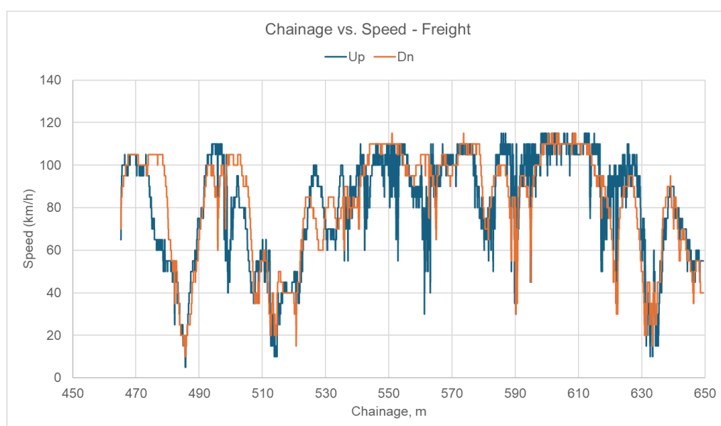
Figure 2 Chainage vs. speed – Freight trains
