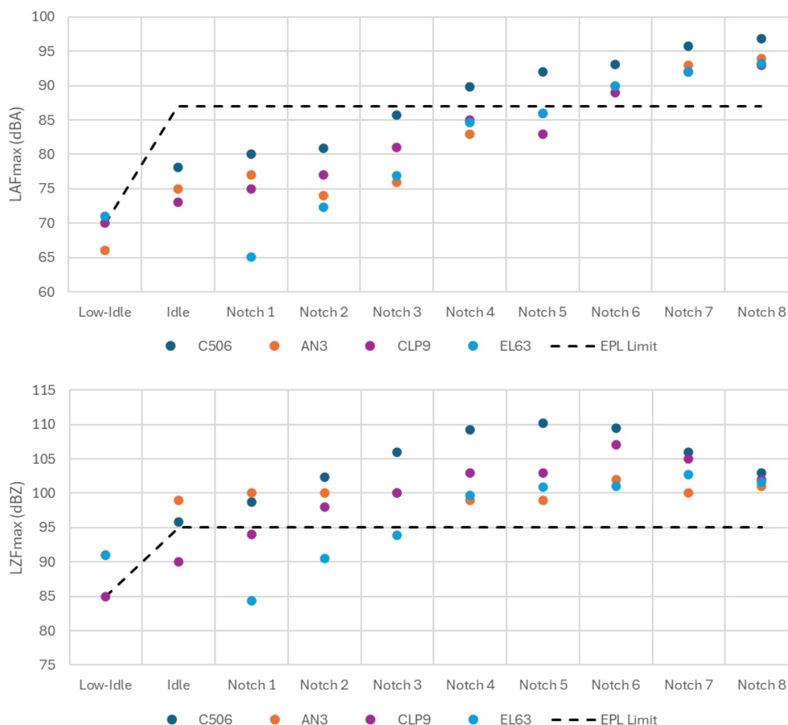
Figure 2 Stationary noise test results at 15m from the track centreline for target locomotive classes – A-weighted (top) and Z-weighted (bottom)
