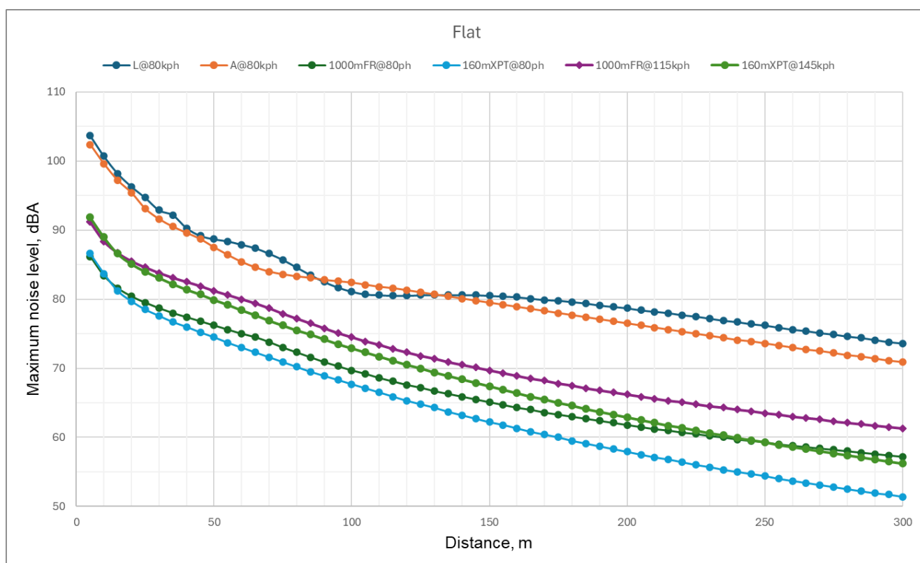
Figure 7 N2K propagation with distance, locomotives (flat) and wagons
