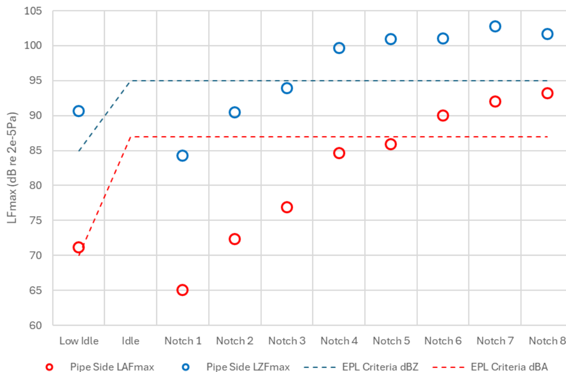
Figure 3 Noise test results for EL63 (pipe side – 15m from the track centreline at mid-locomotive position)
