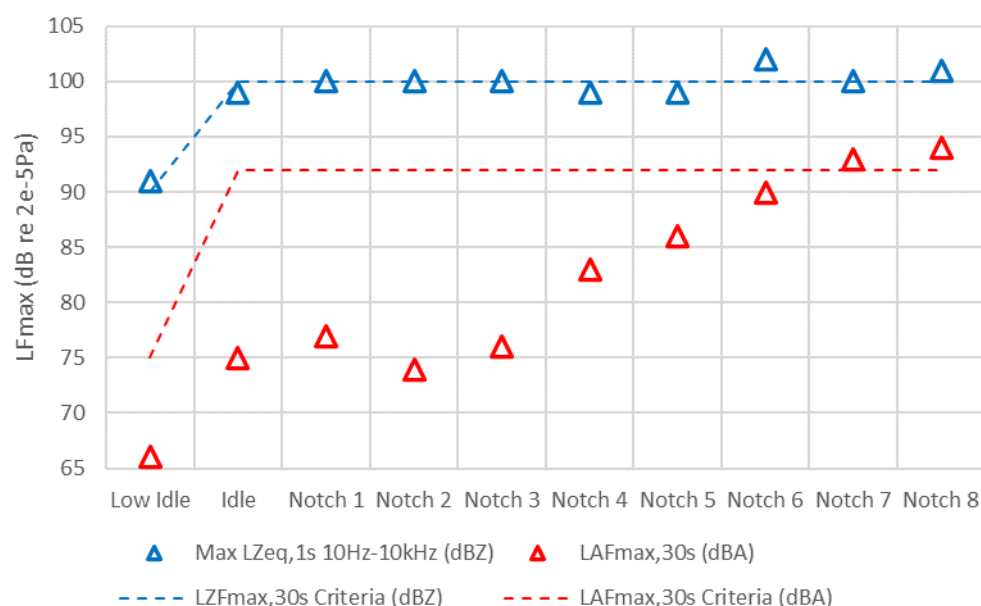
Figure 3 Noise test results for AN3 (pipe side – 15m from the track centreline at mid-locomotive position)
