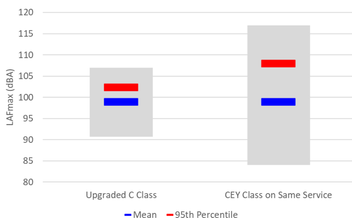
Figure 4 Revenue service LAFmax noise levels at approx. 20m from the track centreline for upgraded C and CEY Class locomotives
