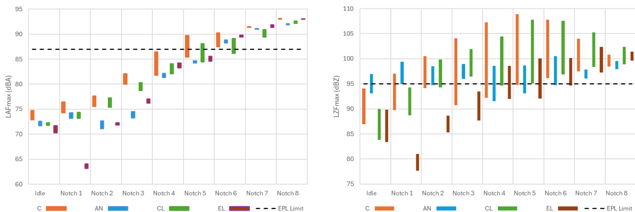
Figure 5 Predicted locomotive change in overall stationary type test noise levels at 15m from the track centreline due to upgrade under the LNCP – A-weighted (left) and unweighted (right). The upper end of the range is the noise level before upgrade, the lower end is after upgrade.
