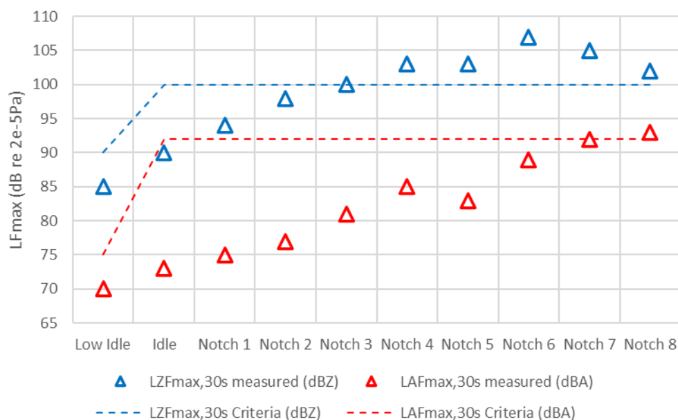
Figure 3 Noise test results for CLP09 (pipe side – 15m from the track centreline at mid-locomotive position)
