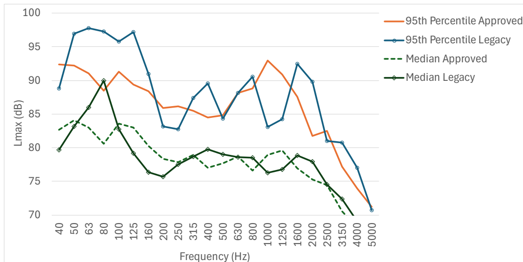
Figure 8 Indicative locomotive Noise Spectra
