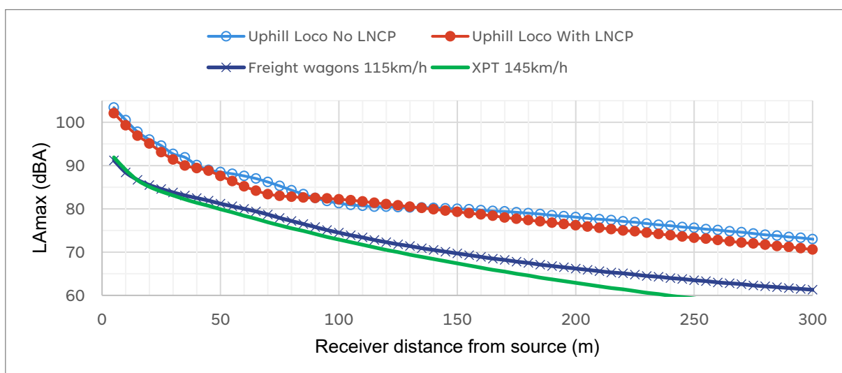
Figure 9 Example of noise propagation over distance for locomotive with and without LNCP
