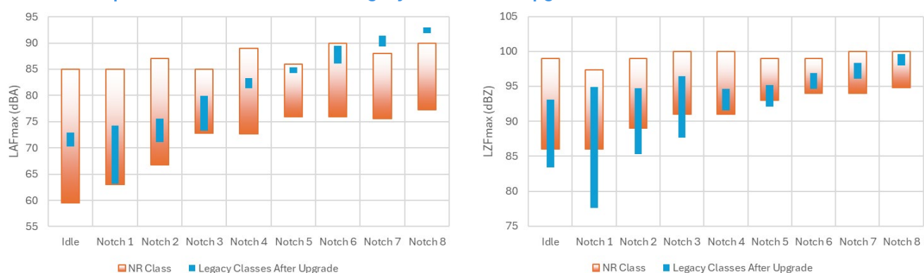
Figure 6 Comparison of the stationary noise levels measured on NR Class at 15m from the track centreline with the predicted noise levels of the Legacy Classes after upgrade
