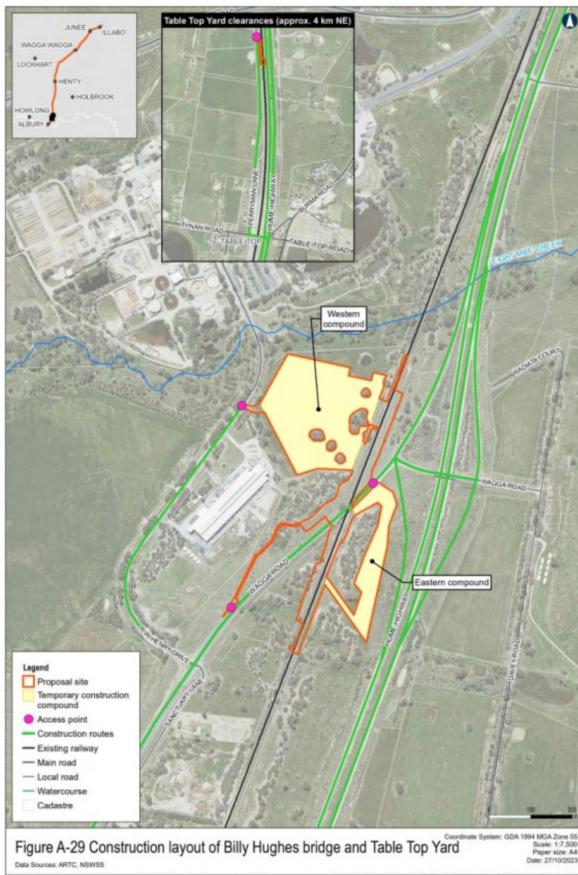
Billy Hughes bridge and Table Top Yard
