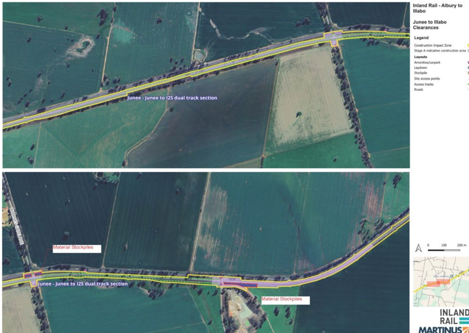
Junee to Illabo Clearances (2 of 4)
