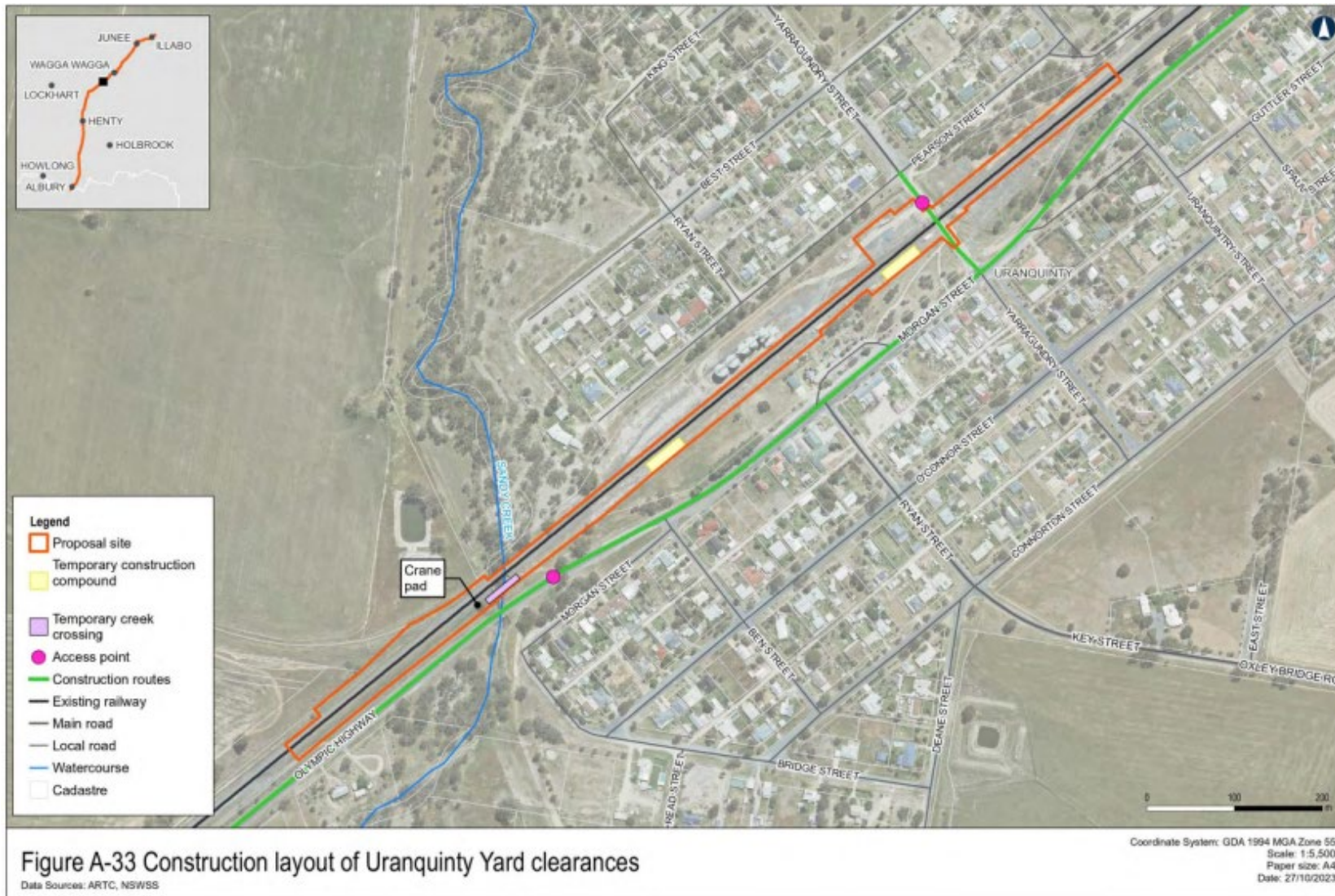
Uranquinty Yard clearances
