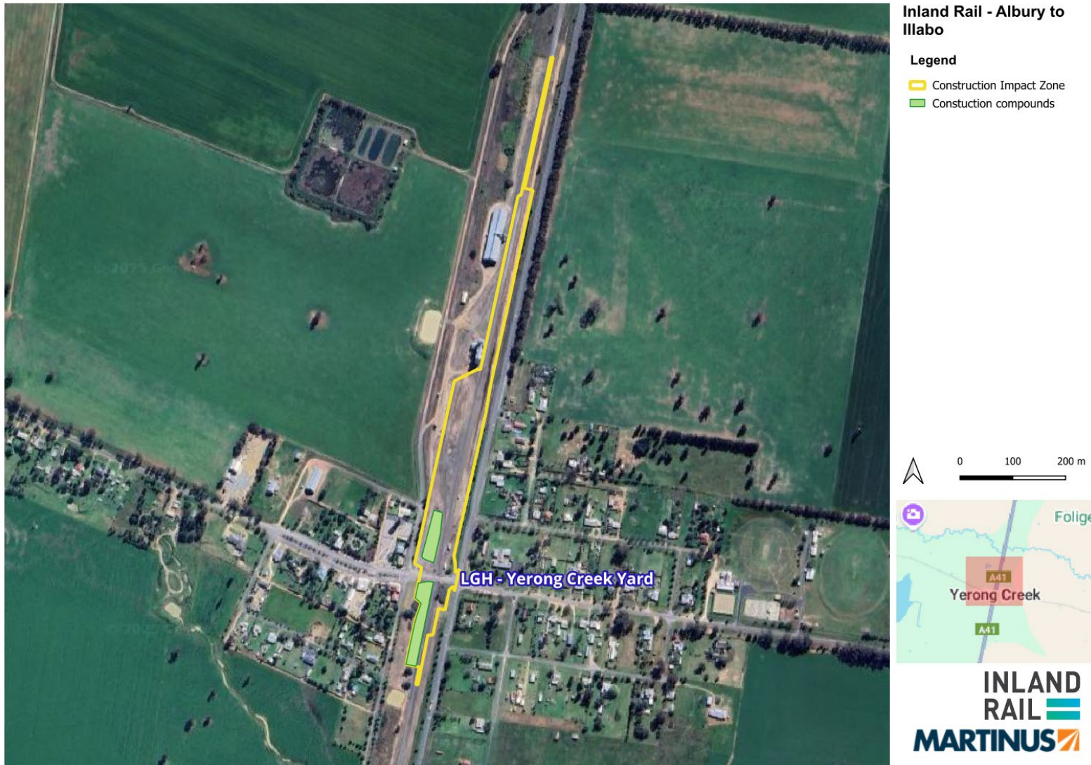
FIGURE 10: YERONG CREEK YARD CLEARANCES ENHANCEMENT SITE
