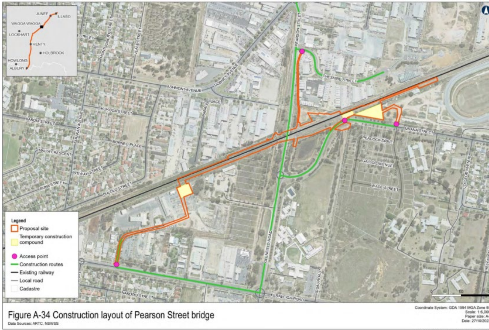
Pearson Street bridge
