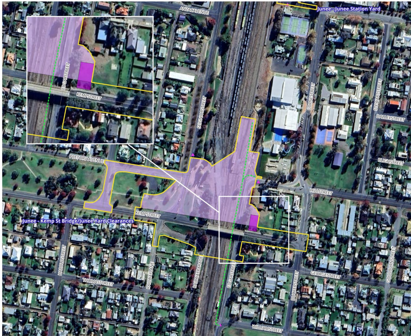
Junee Yard Clearances
