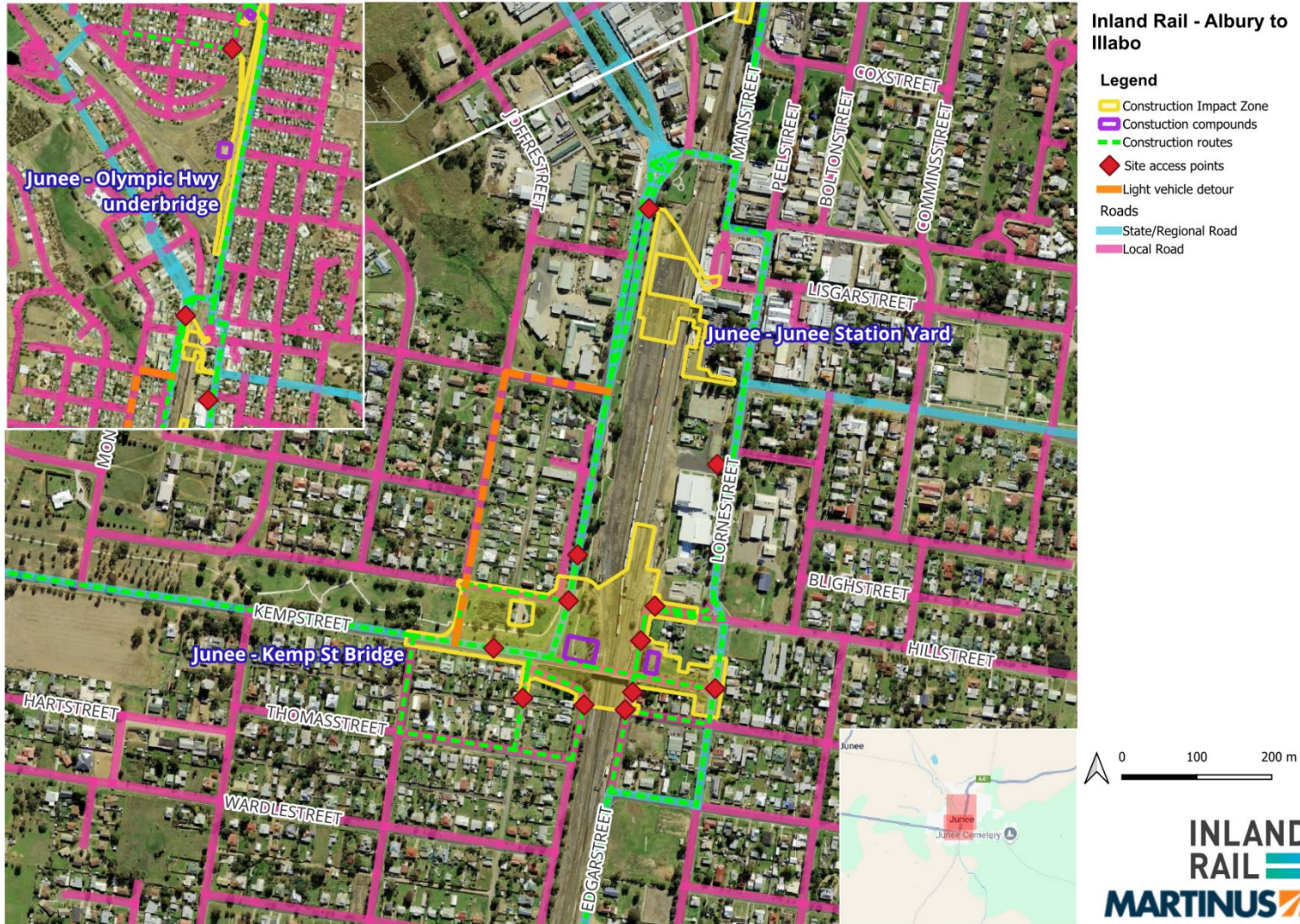
FIGURE 33 JUNEES STATION AND SURROUNDS CONSTRUCTION ROUTES
