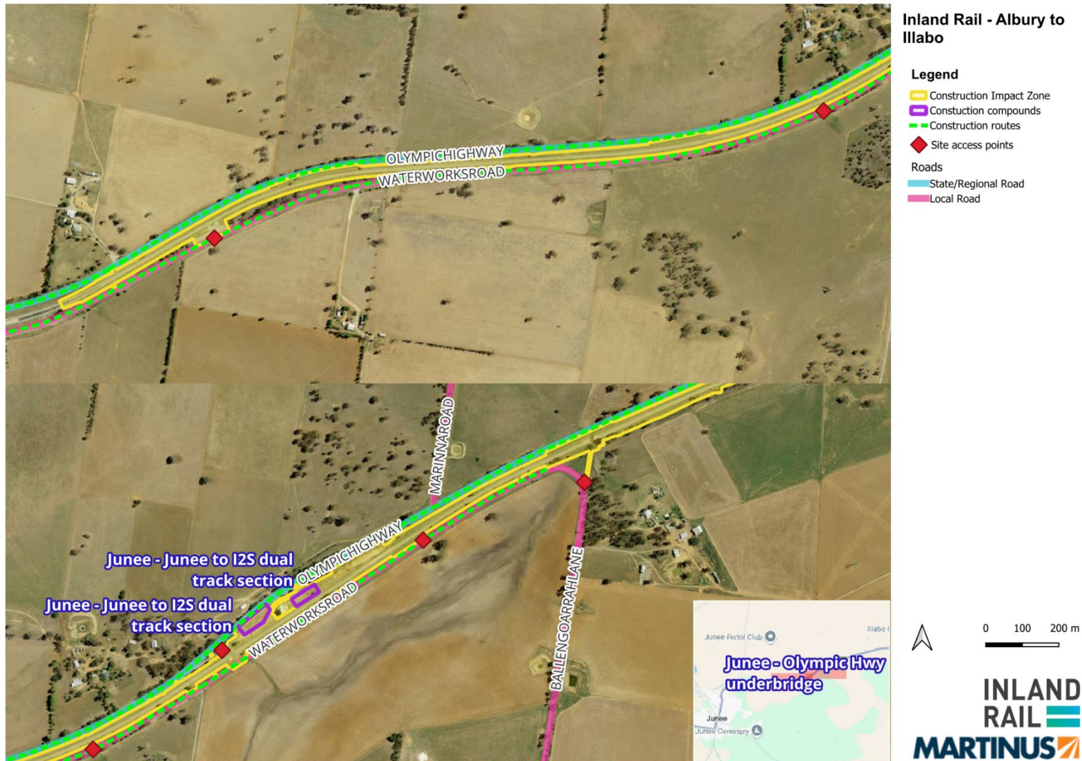
FIGURE 36 JUNEES TO ILLABO CLEARANCES CONSTRUCTION ROUTES
