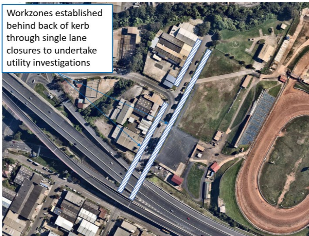
Figure 7-4: Wentworth St work areas
