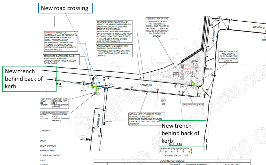
Figure 7-6: Unwin St and Shirley Street trench excavations
