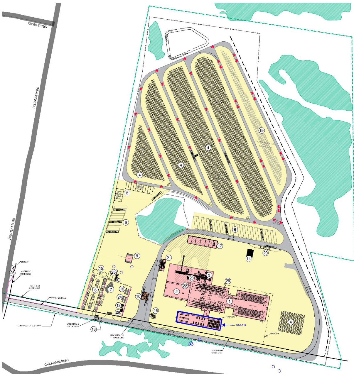
Figure 2-2: Site layout
