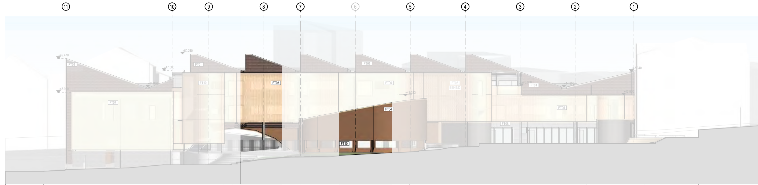
1 ELEVATION Play Area Elevation 1:200 NTS
