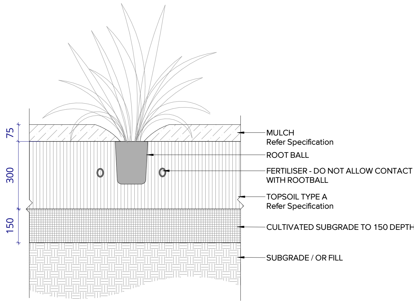
1 DETAILS_MASSPLANTING ON GRADE 1:10
