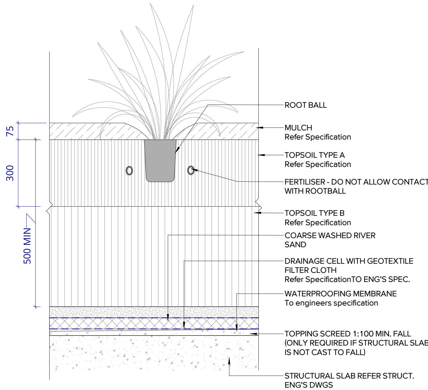
2 DETAILS_MASSPLANTING ON SLAB 1:10
