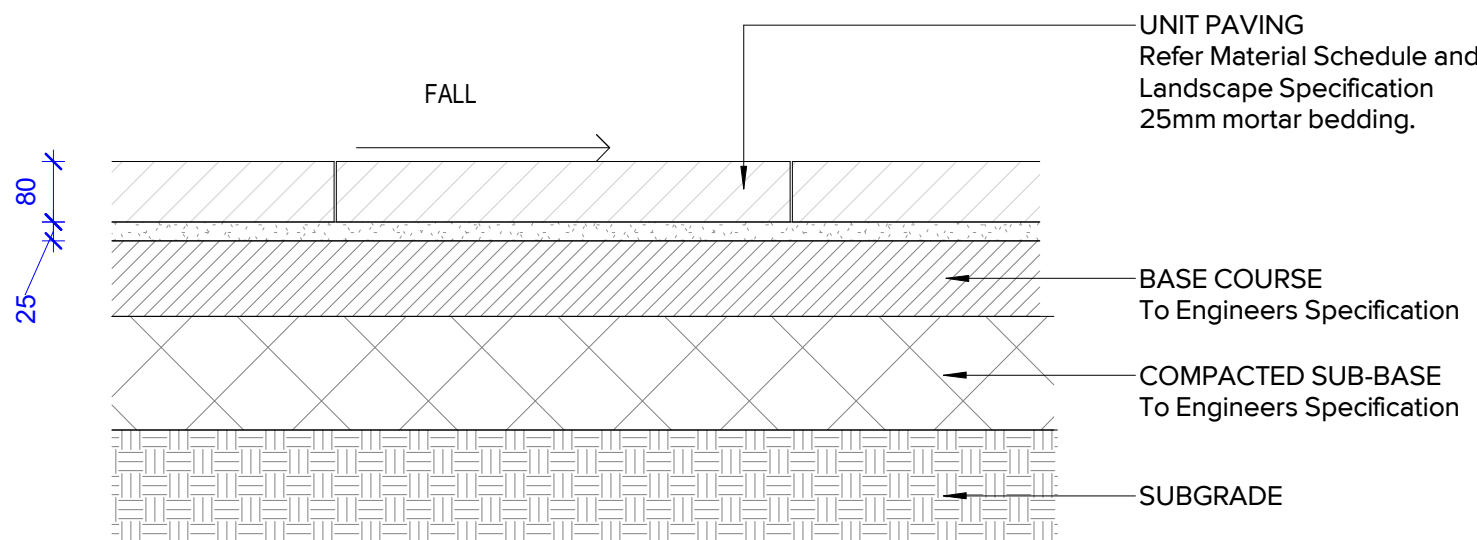
4 TYPICAL UNIT PAVING - SECTION 1:10
