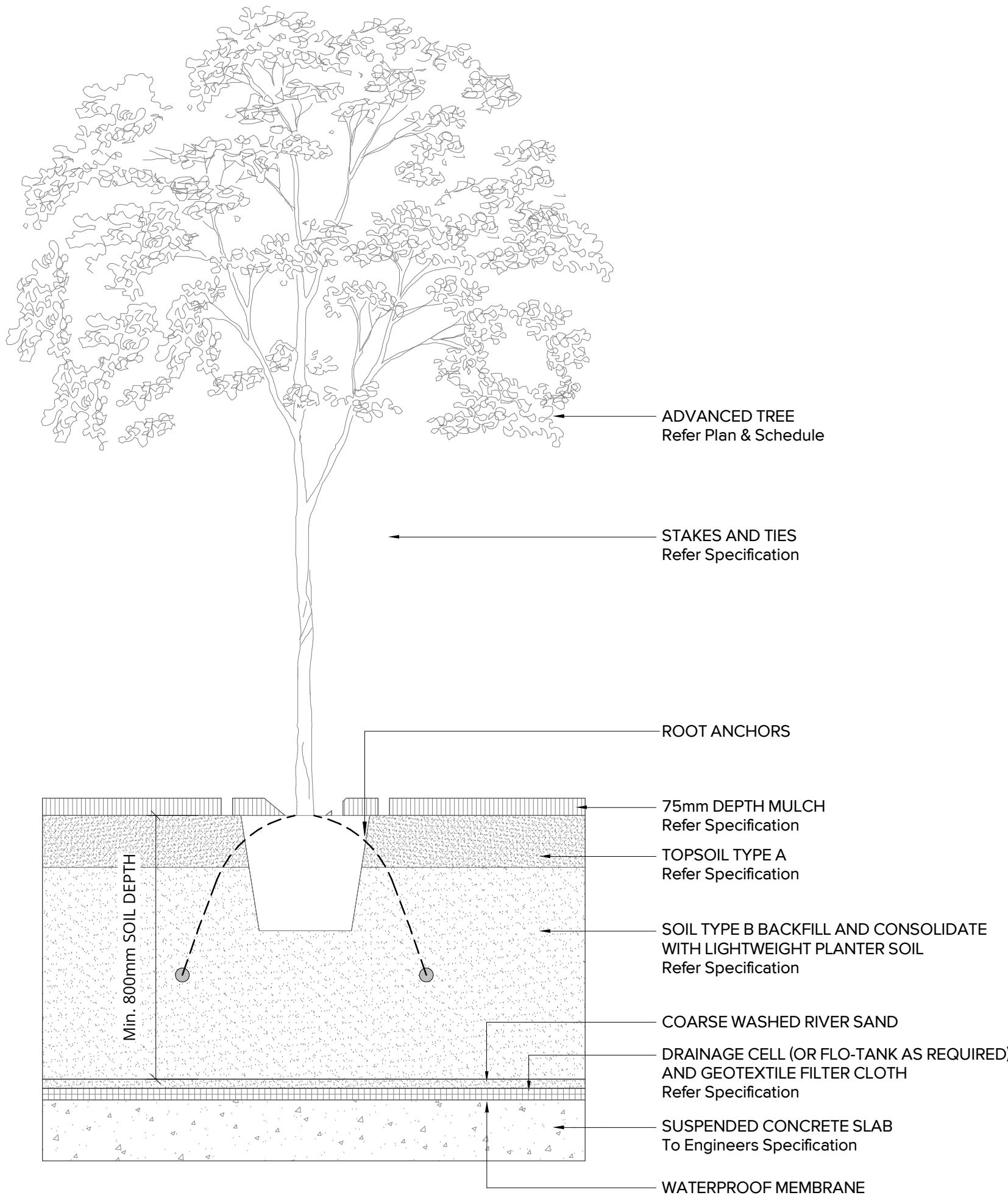
3 DETAILS_TREE ON STRUCTURE 1:20
