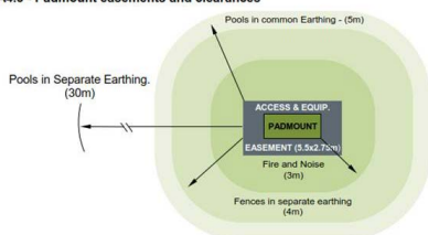
A4.3 - Padmount easements and clearances
