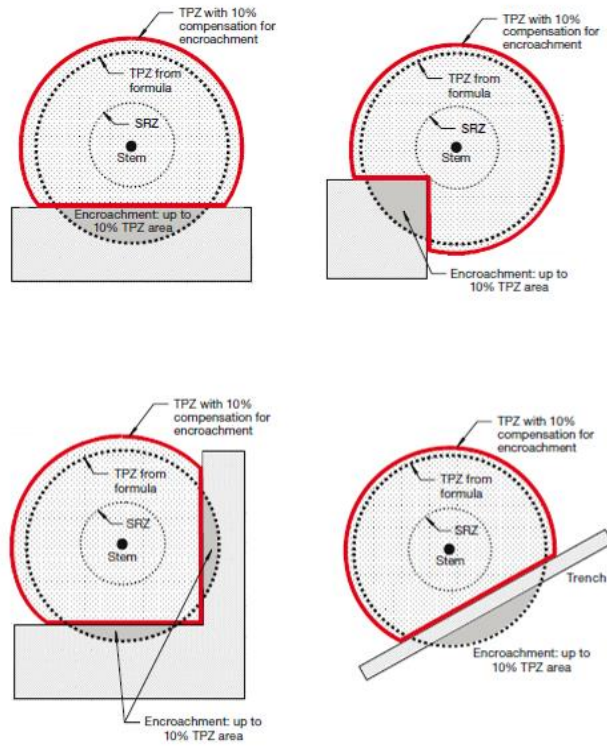
Figure 3 - Minor encroachment on TPZ and 10% compensation for encroachment (Source AS 4970-2009)
