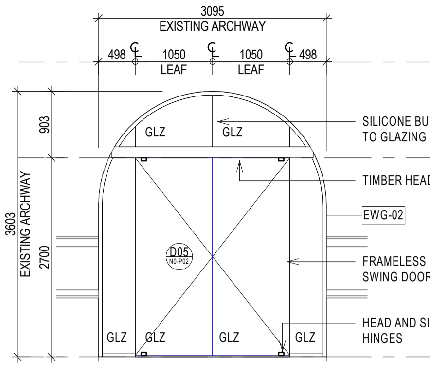
2 RHI NORTH ELEVATION - EWG-N0-P02 1:50
