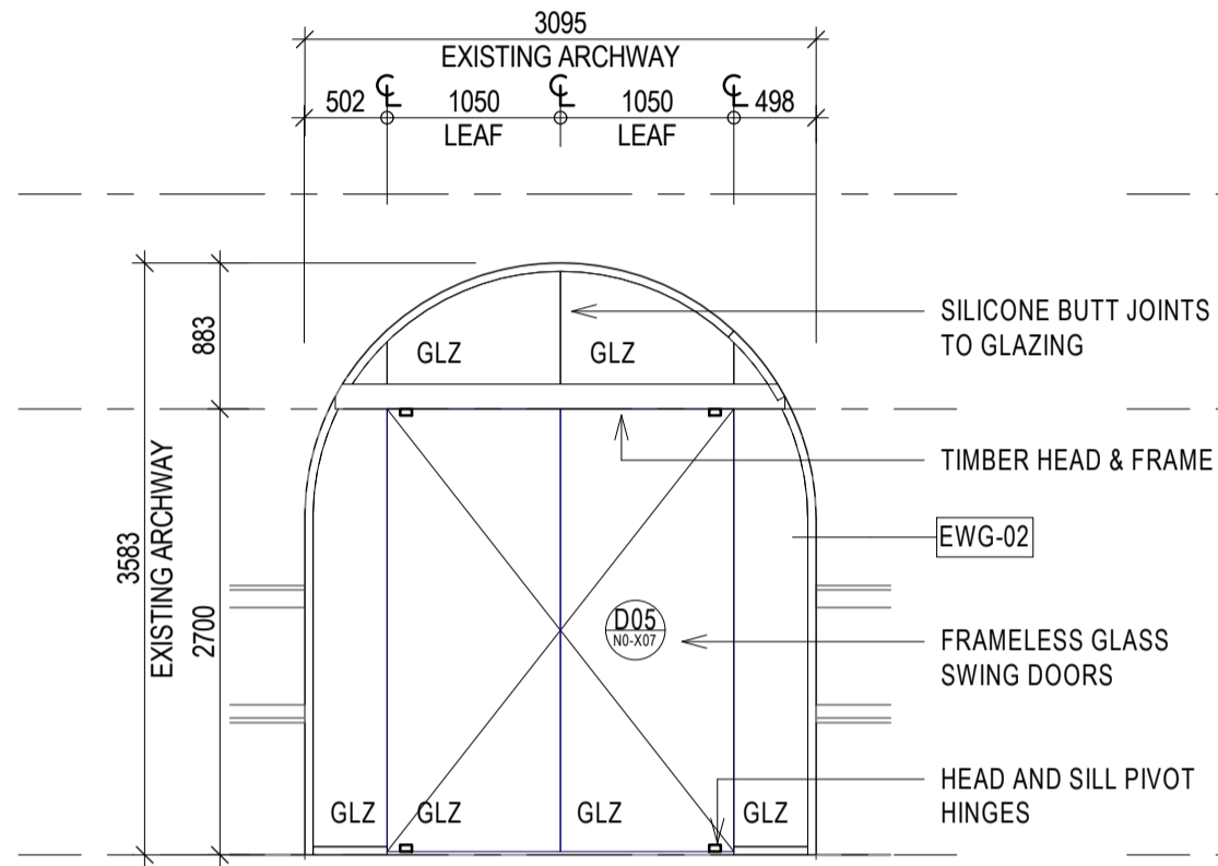
3 RHI NORTH ELEVATION - EWG-N0-X02 1:50
