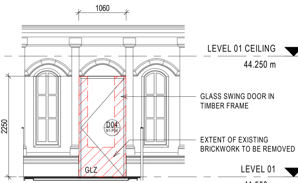
16 RHI SOUTH ELEVATION - EWG-N1-P04 1:50
