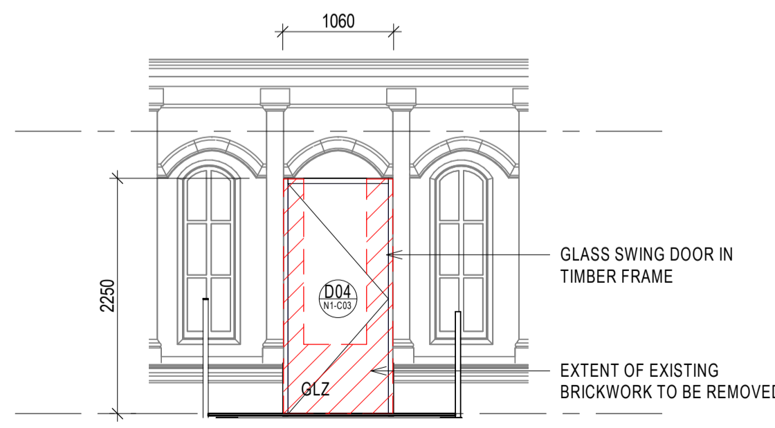
15 RHI SOUTH ELEVATION - EWG-N1-C03 1:50
