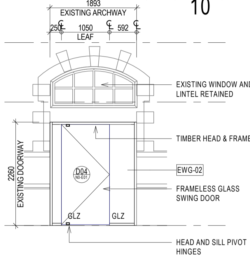
7 RHI EAST ELEVATION - EWG-N0-E01 1:50
