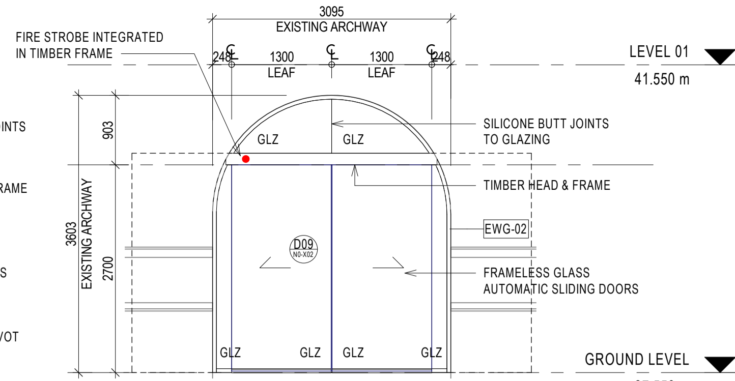
3 RHI NORTH ELEVATION - EWG-N0-X02 1:50
