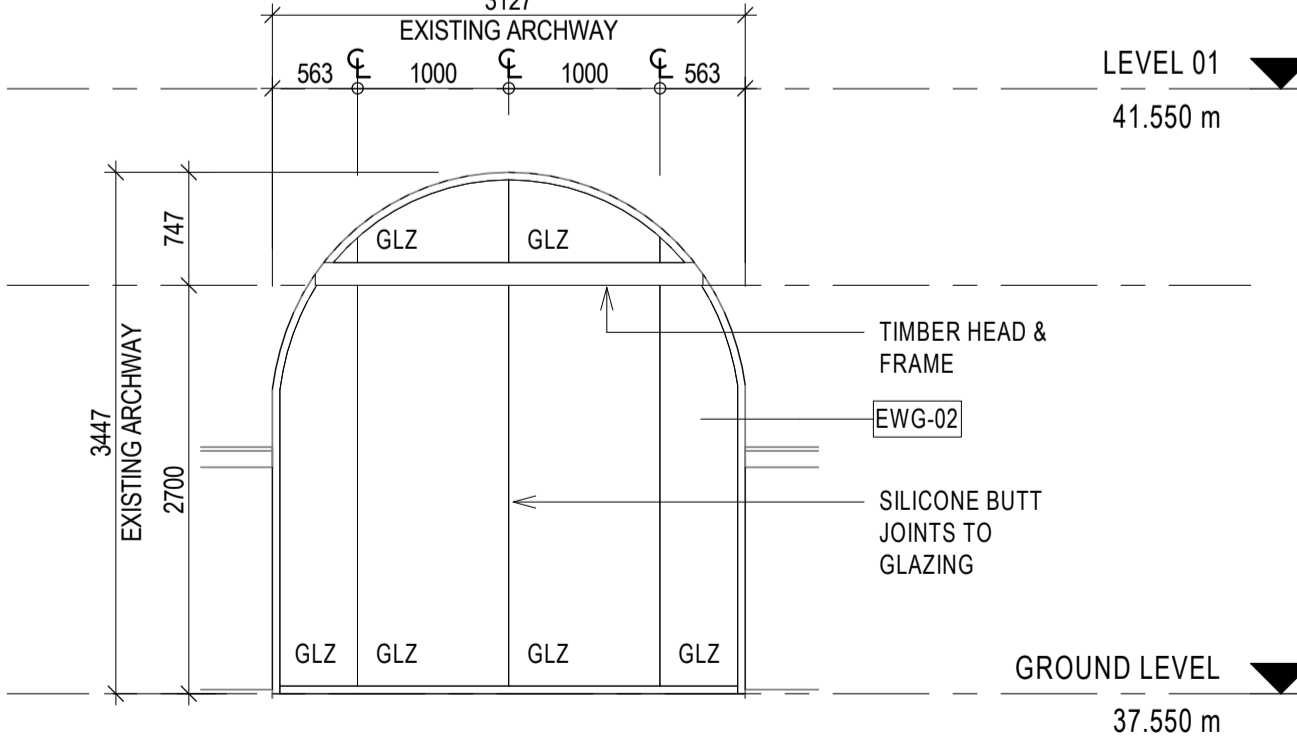
9 RHI EAST ELEVATION - EWG-N0-B02 1:50
