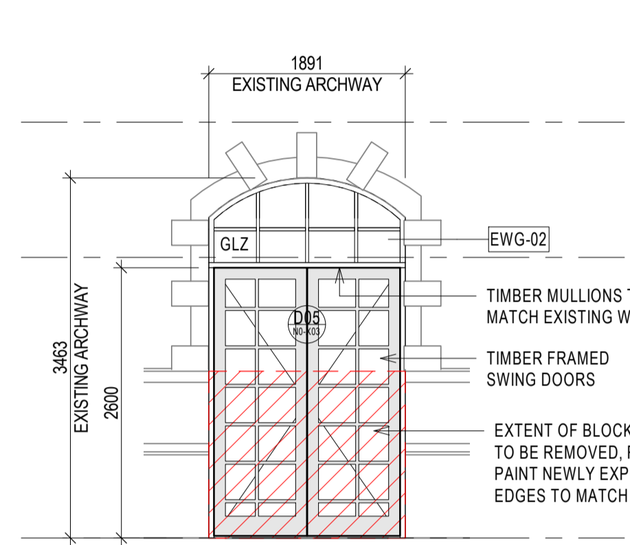
1 RHI NORTH ELEVATION - EWG-N0-G19 1:50
