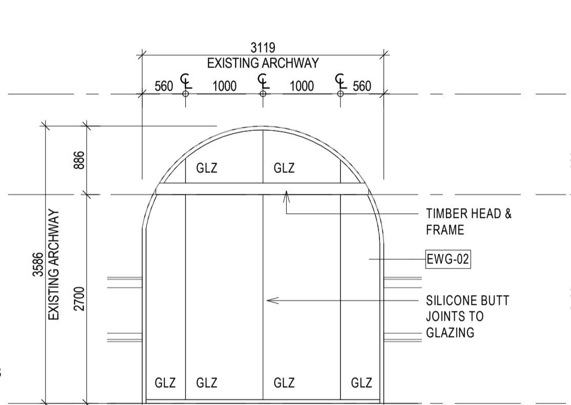
6 RHI EAST ELEVATION - EWG-N0-X07 1:50
