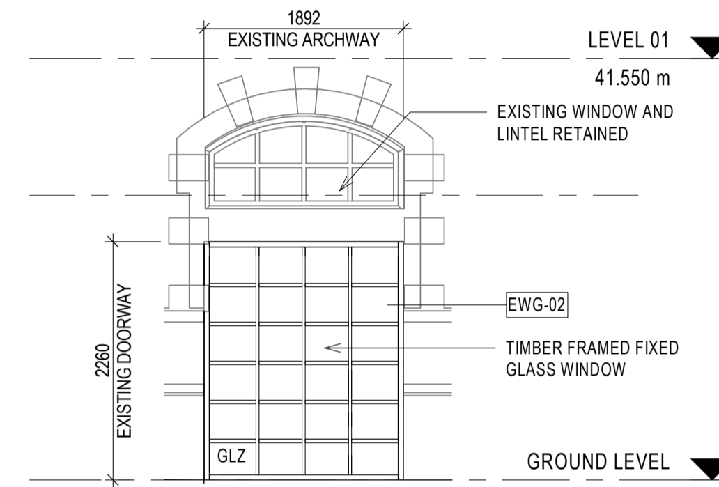
8 RHI EAST ELEVATION - EWG-N0-XXX 1:50
