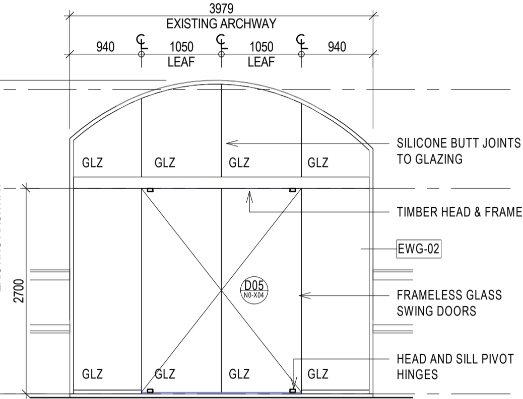
2 RHI NORTH ELEVATION - EWG-N0-P02 1:50
