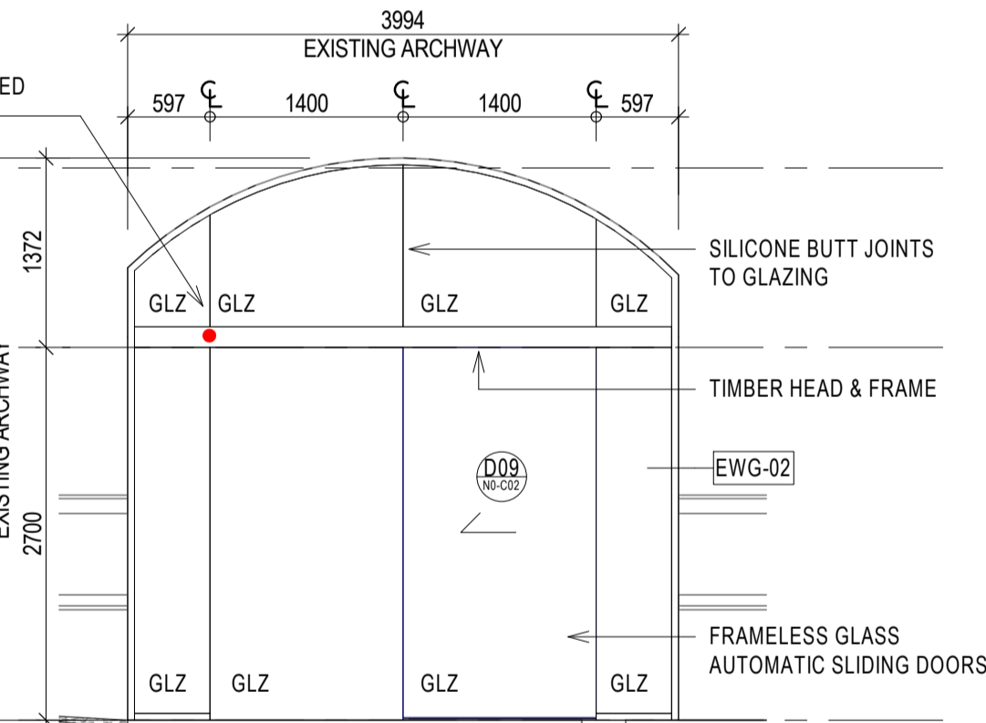
5 RHI EAST ELEVATION - EWG-N0-X04 1:50
