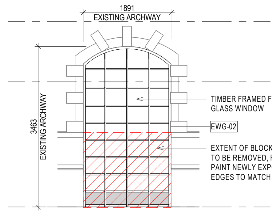
1 RHI NORTH ELEVATION - EWG-N0-G19 1:50
