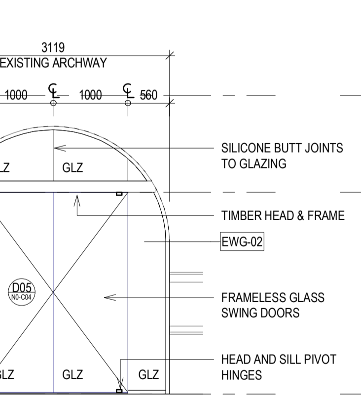
7 RHI EAST ELEVATION - EWG-N0-E01 1:50
