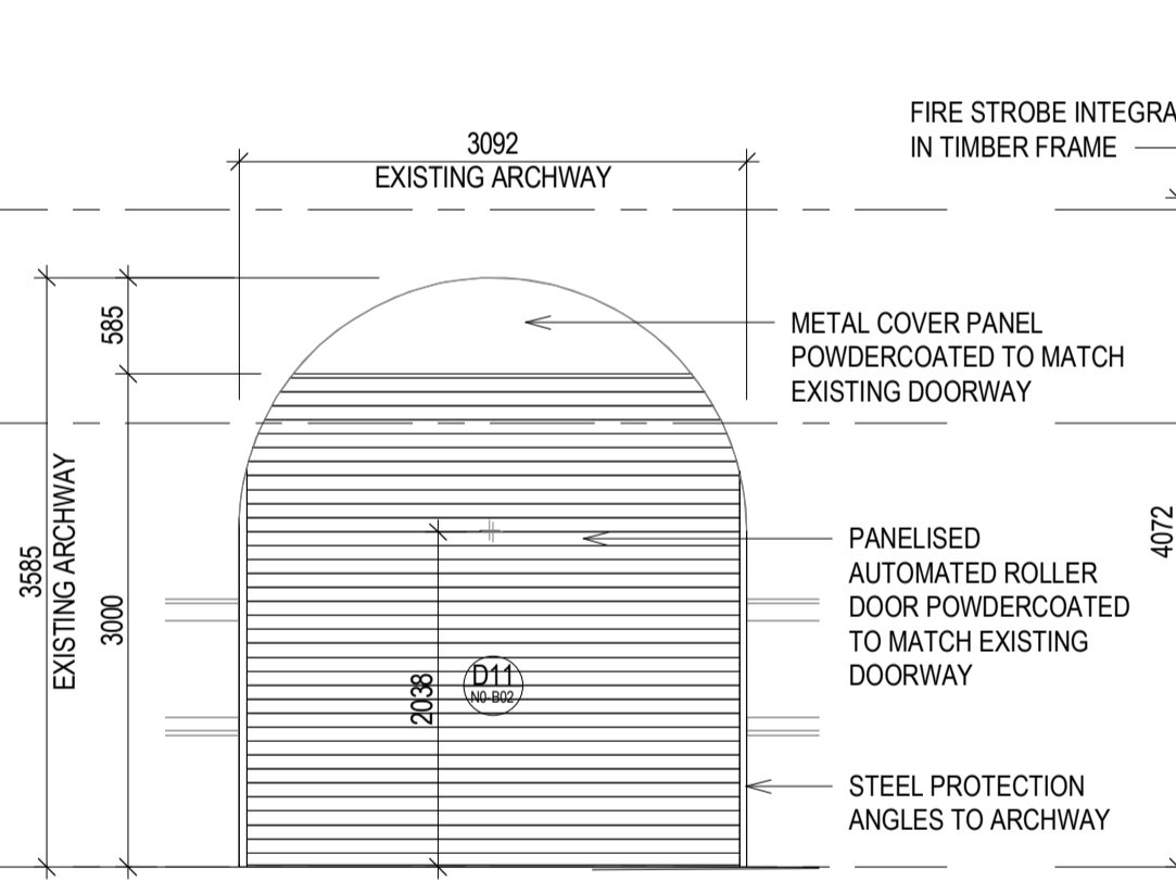
4 RHI NORTH ELEVATION - EWG-N0-X03 1:50
