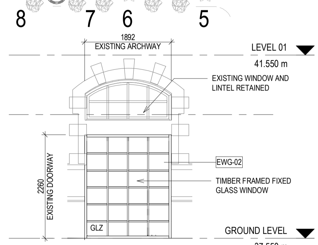
8 RHI EAST ELEVATION - EWG-N0-XXX 1:50
