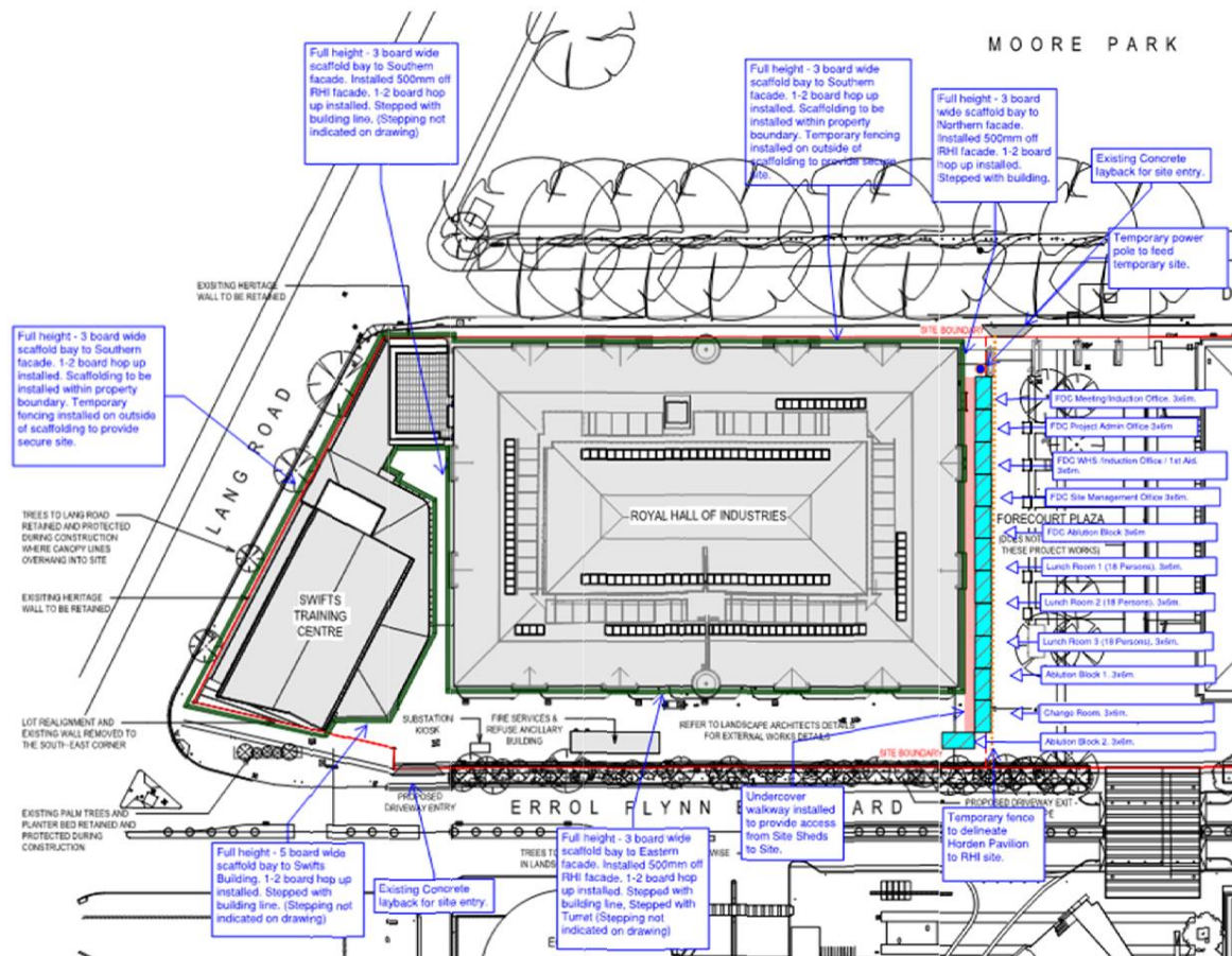
Figure 2: Site Establishment Plan (Provided by FDC)
