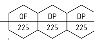
DOWNPIPE & OVERFLOWS FROM ROOF & RAINWATER TANK ABOVE.
