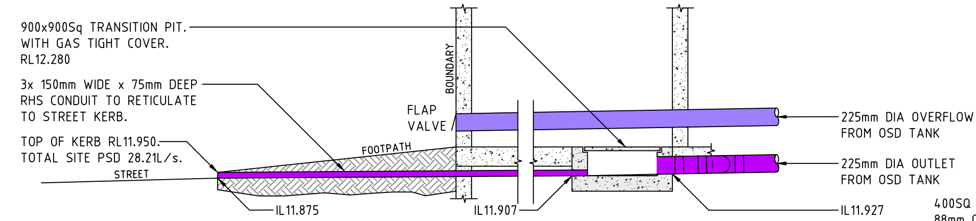
KERB & TRANSITION PIT SECTION SCALE 1:50
