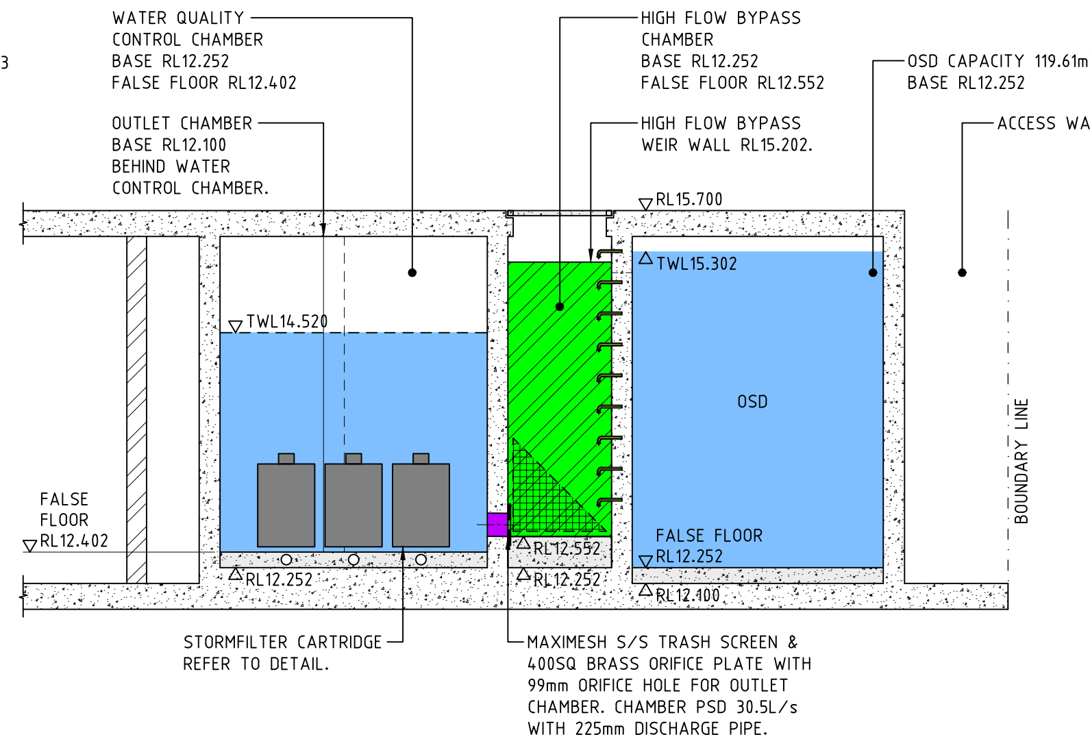
OSD TANK SECTION B-B SCALE 1:50
