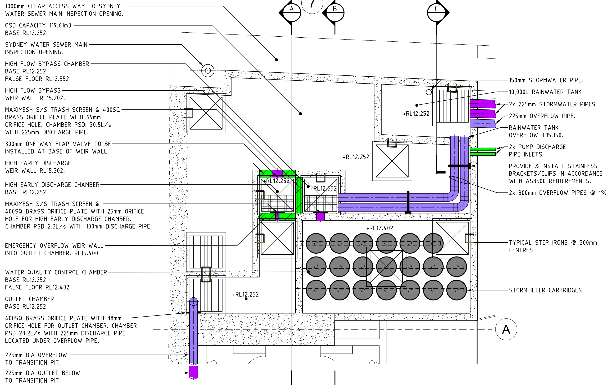
OSD TANK PLAN DETAIL SCALE 1:50
