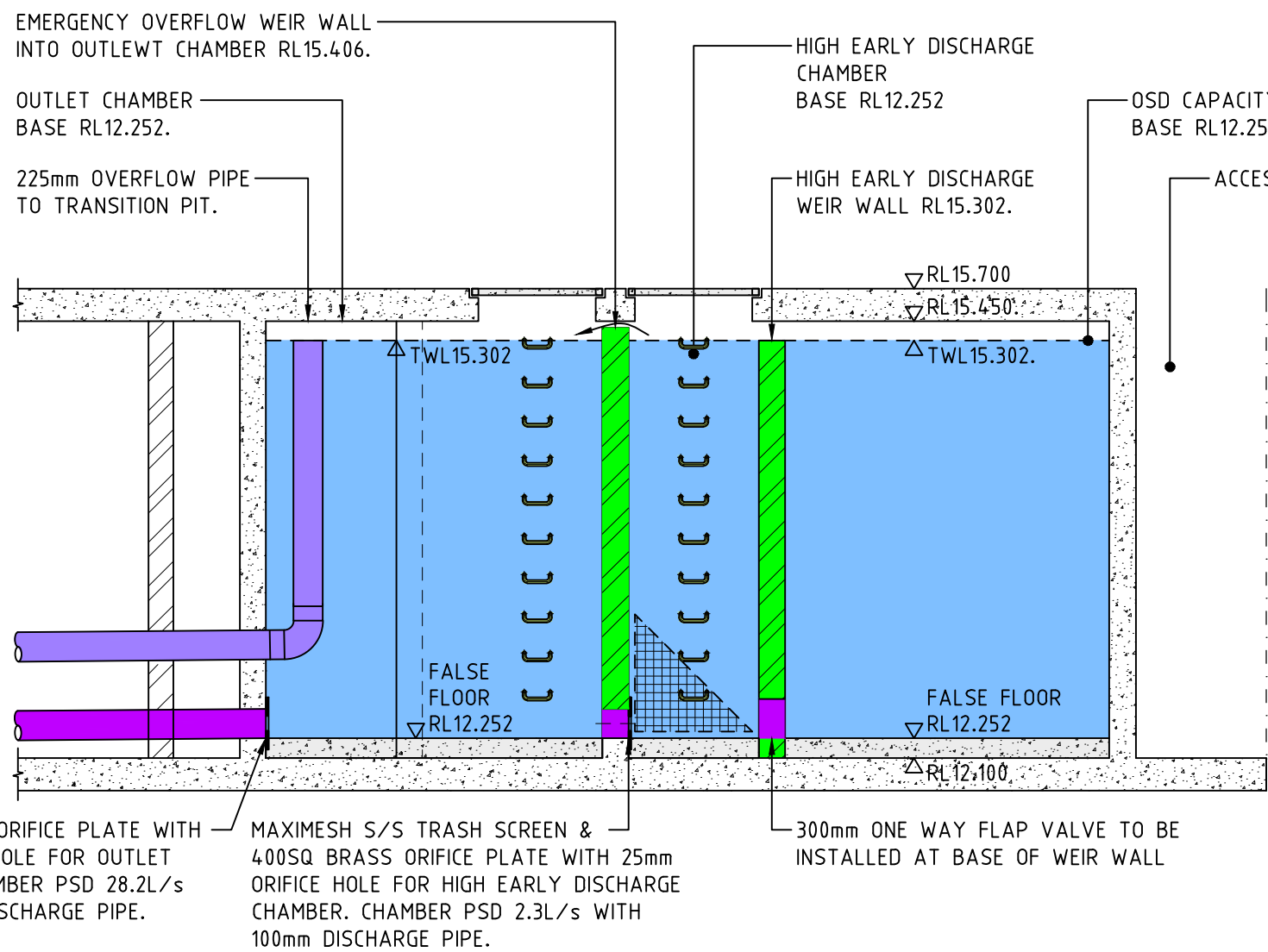
OSD TANK SECTION A-A SCALE 1:50
