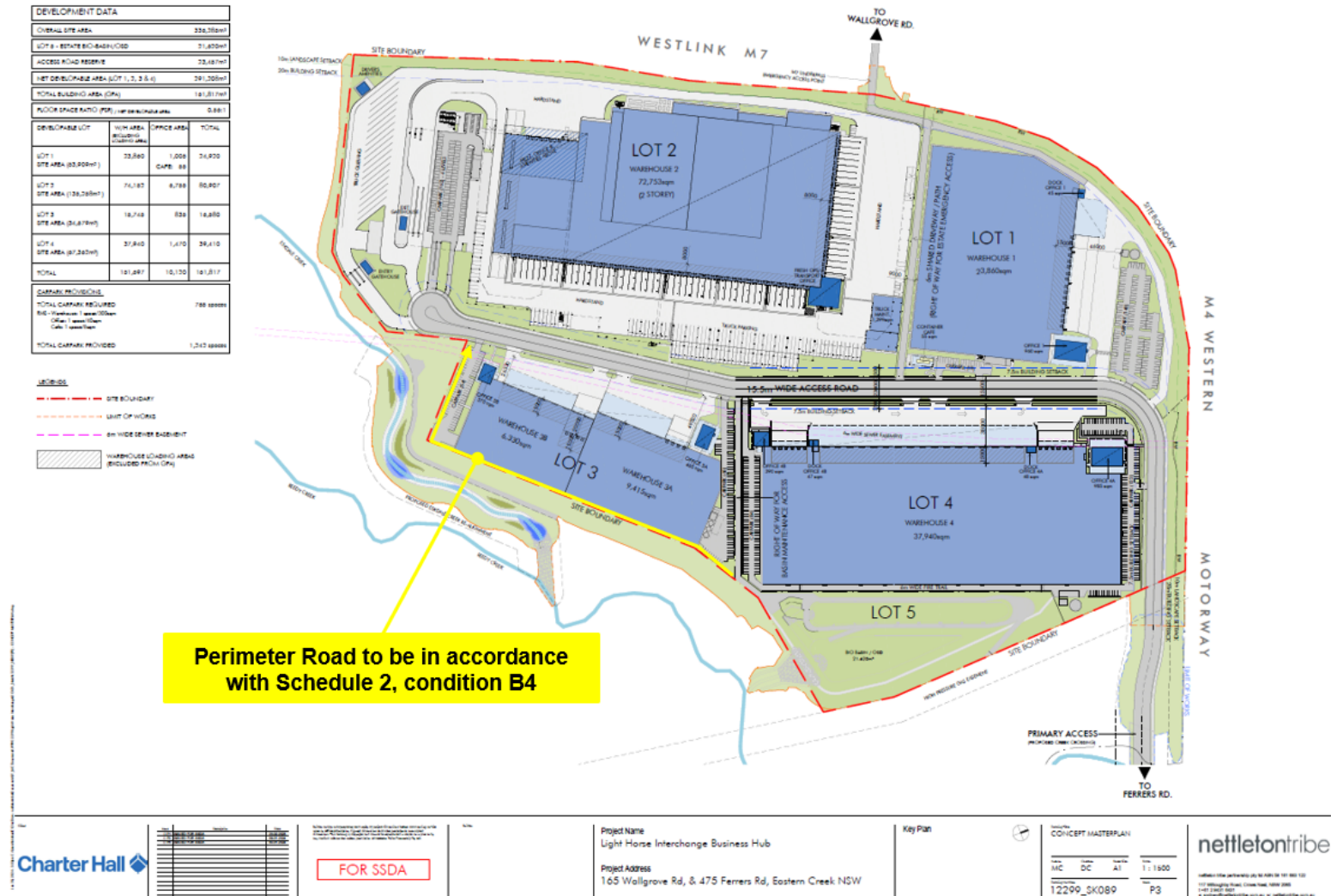
Figure 1: Concept Masterplan
