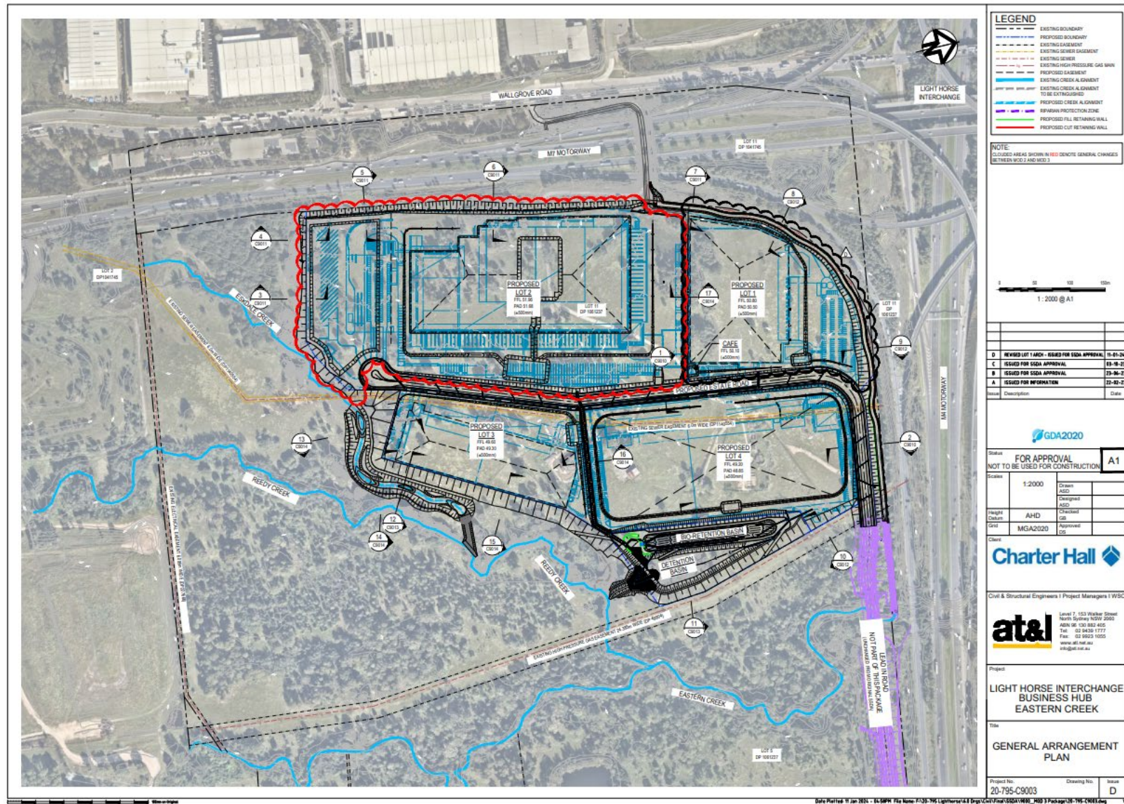
Figure 2: Stage 1 Works - General Arrangement Plan
