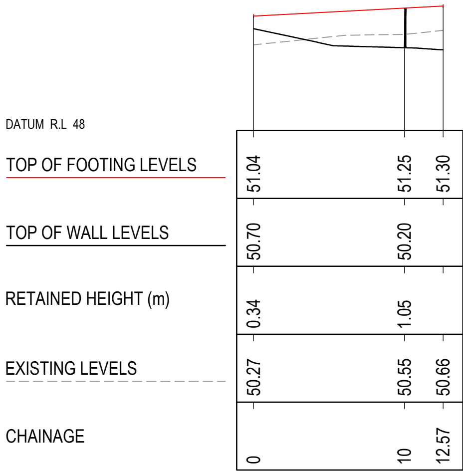
RETAINING WALL ELEVATION - MW06
