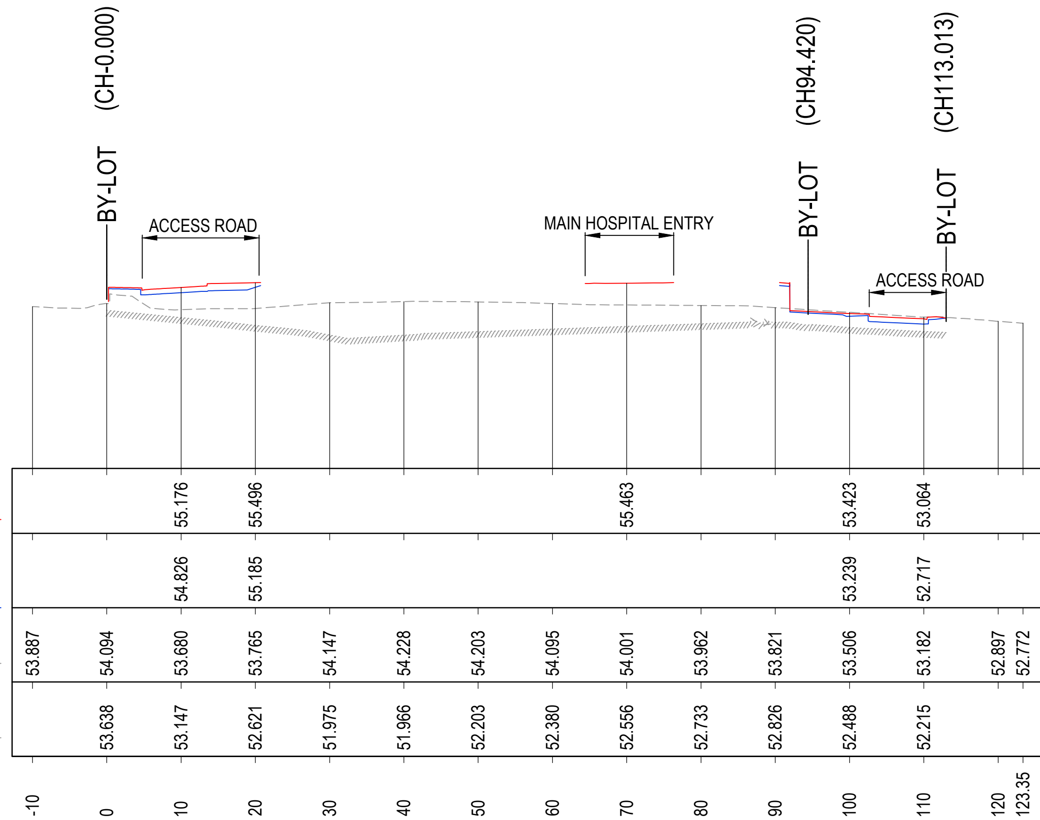
BULK EARTHWORKS SECTION - BE-C A1 Horizontal scale 1:500 A1 Vertical scale 1:250
