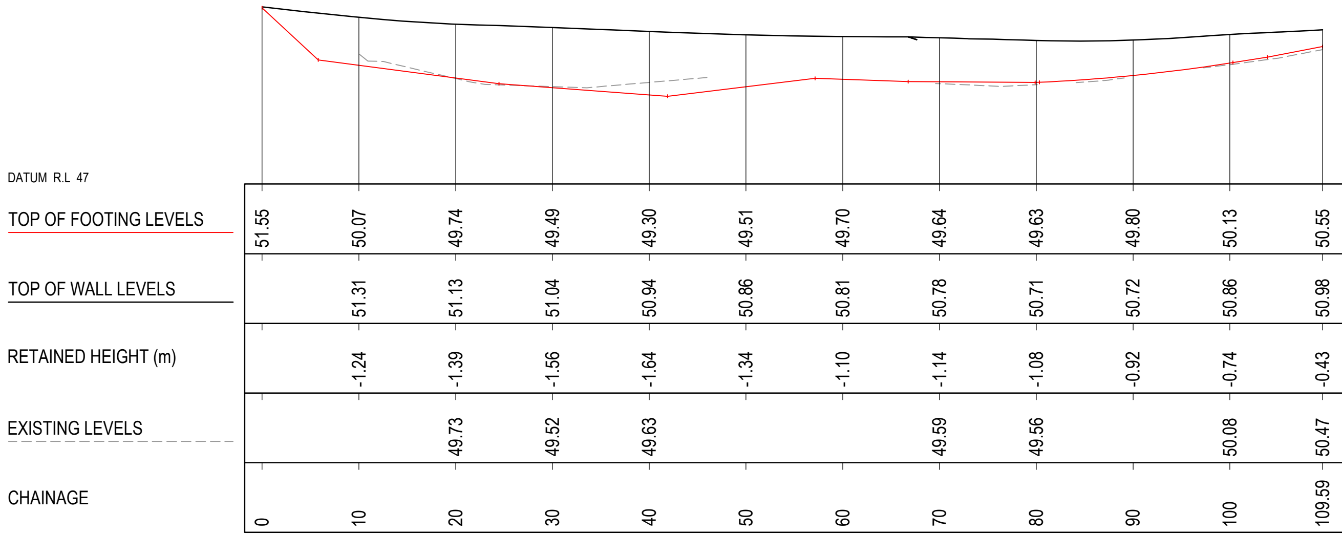
RETAINING WALL ELEVATION - MW02
