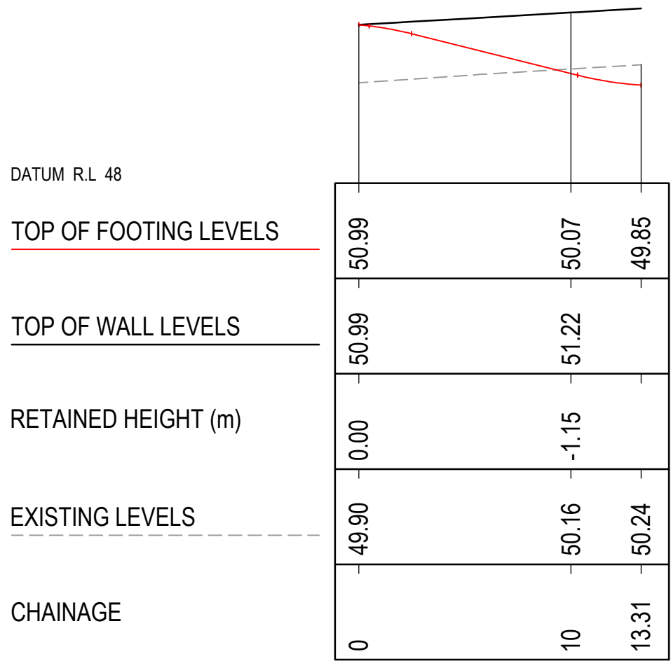
RETAINING WALL ELEVATION - MW05
