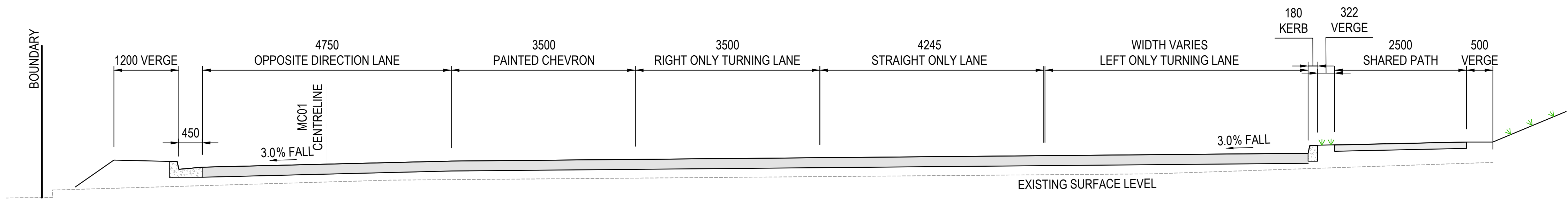
PROPOSED ROAD SECTION 1 SCALE 1:50 265001
