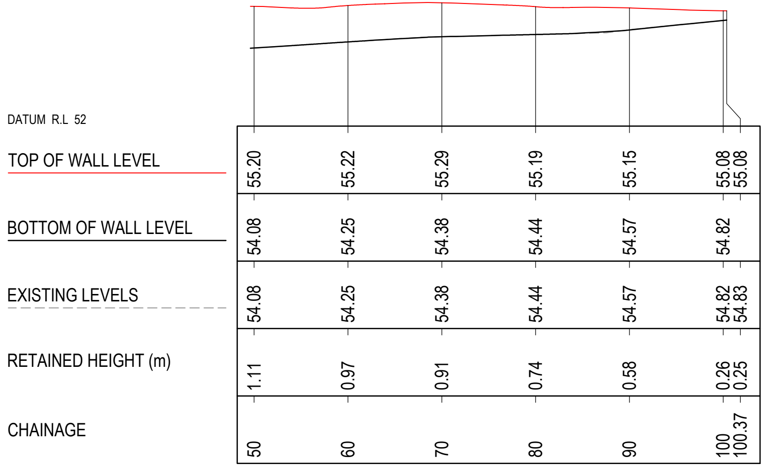
RETAINING WALL ELEVATION - MW01
