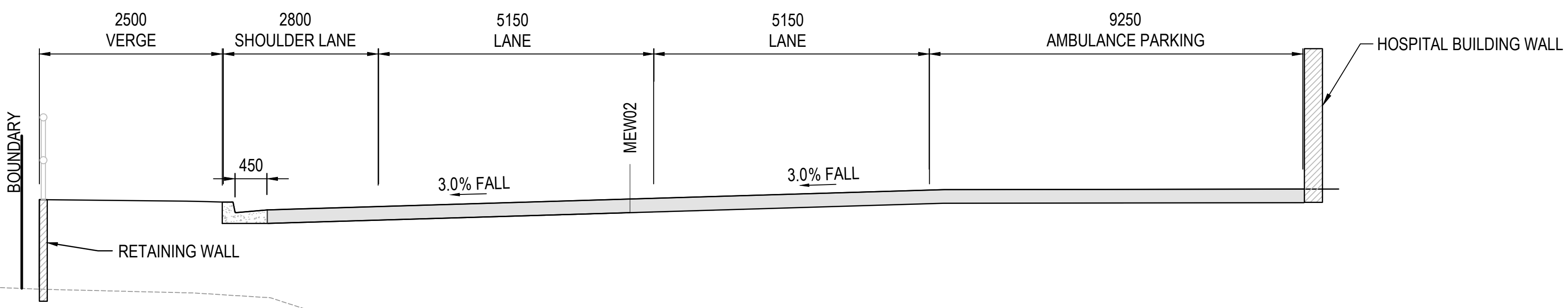
PROPOSED ROAD SECTION 4 SCALE 1:50 265001
