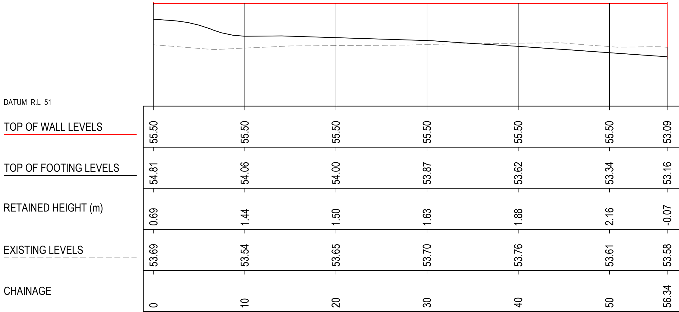
RETAINING WALL ELEVATION - MW08
