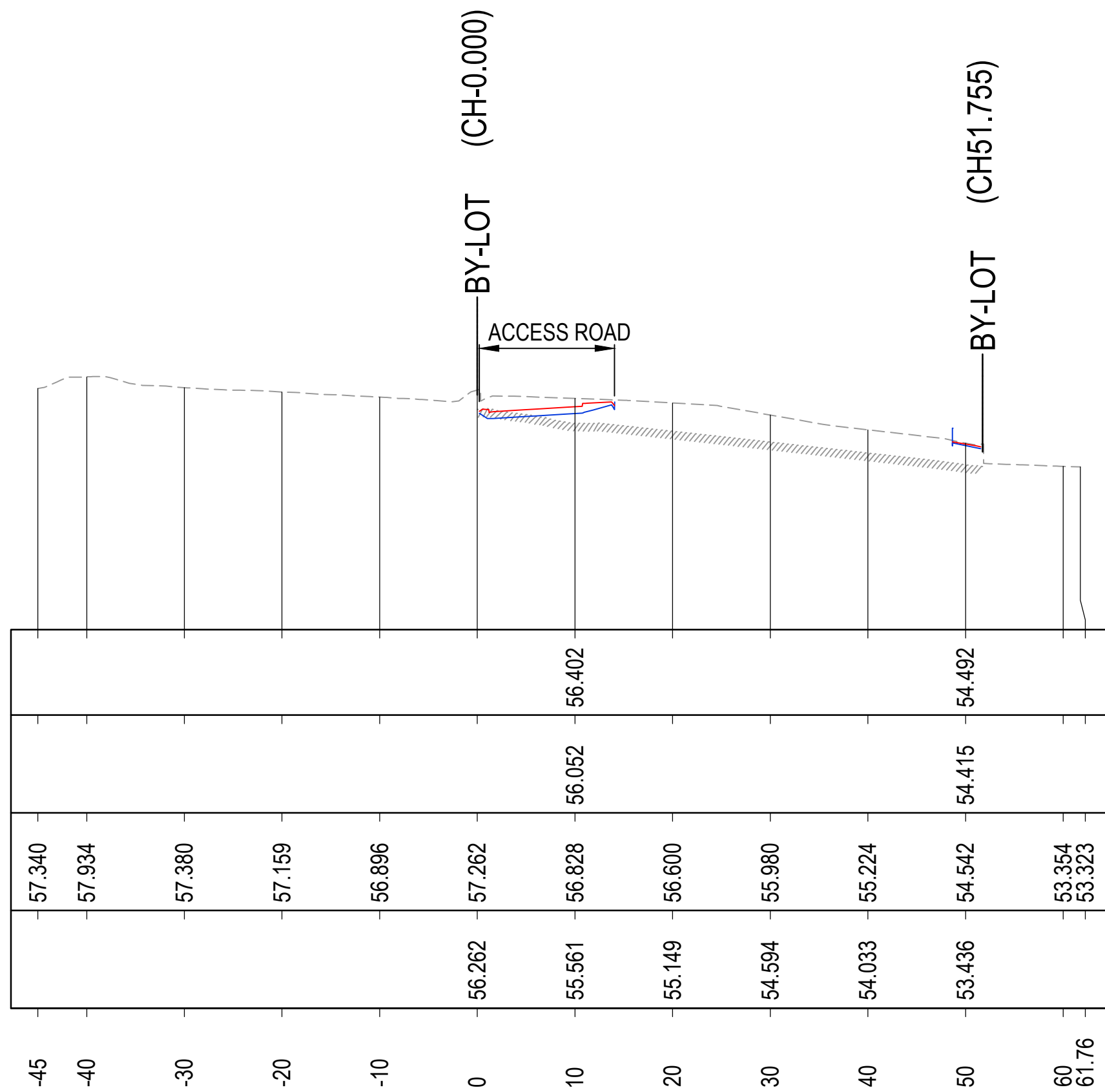
BULK EARTHWORKS SECTION - BE-B A1 Horizontal scale 1:500 A1 Vertical scale 1:250
