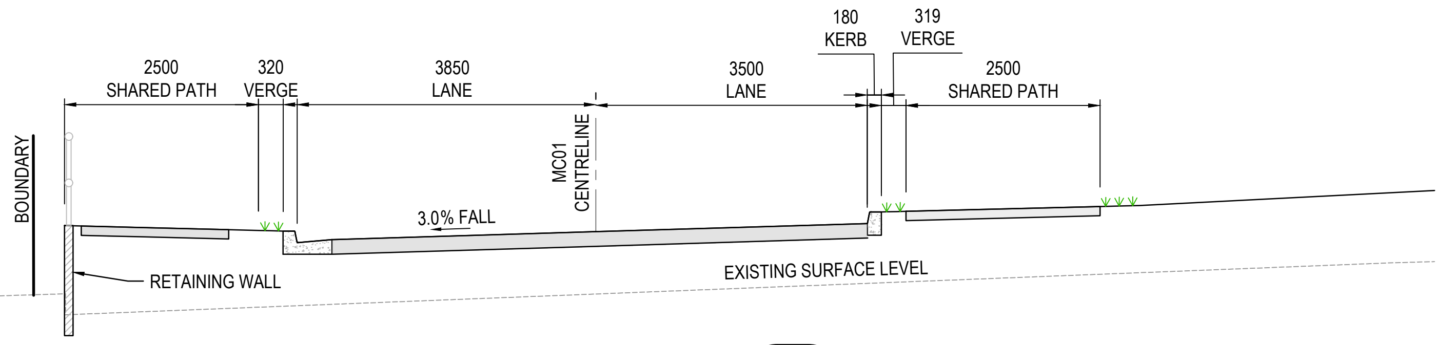
PROPOSED ROAD SECTION 3 SCALE 1:50 265001
