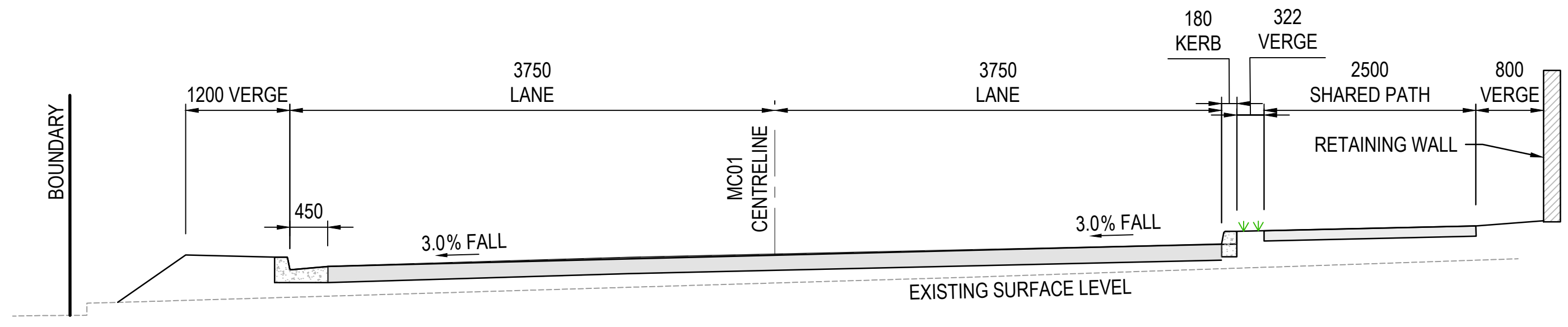
PROPOSED ROAD SECTION 2 SCALE 1:50 265001
