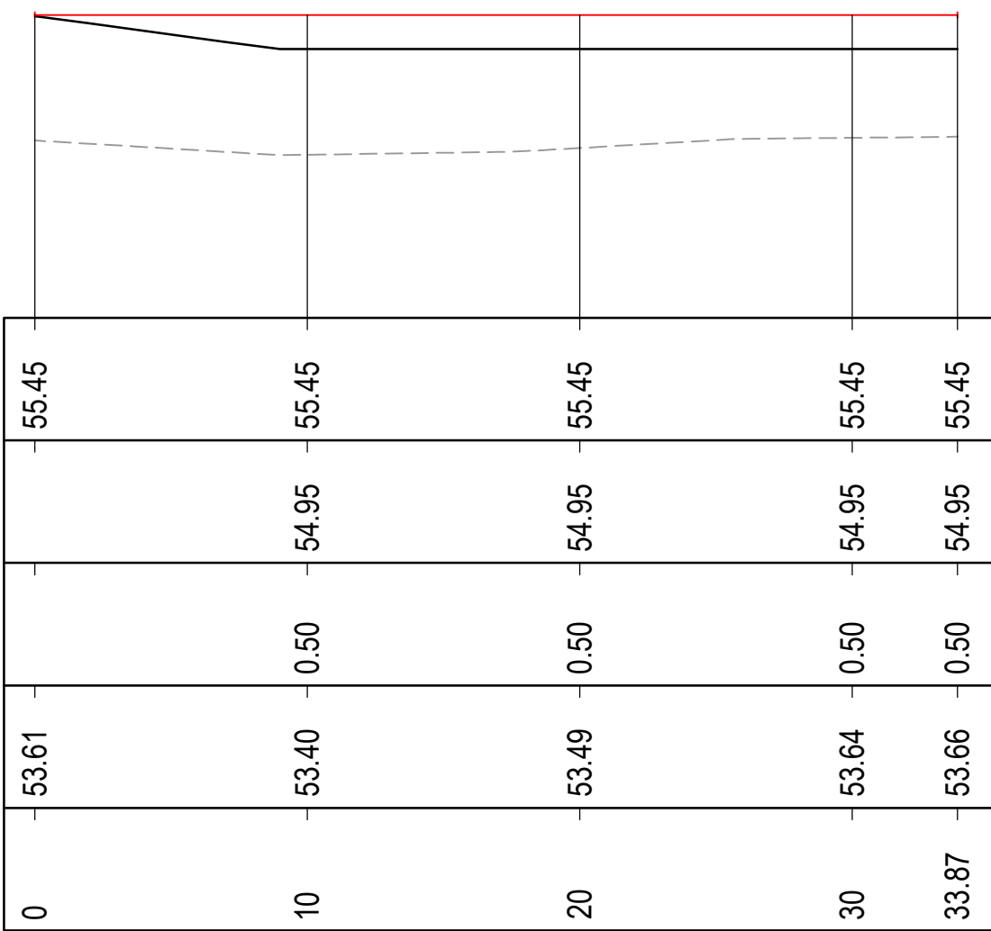
RETAINING WALL ELEVATION - MW11
