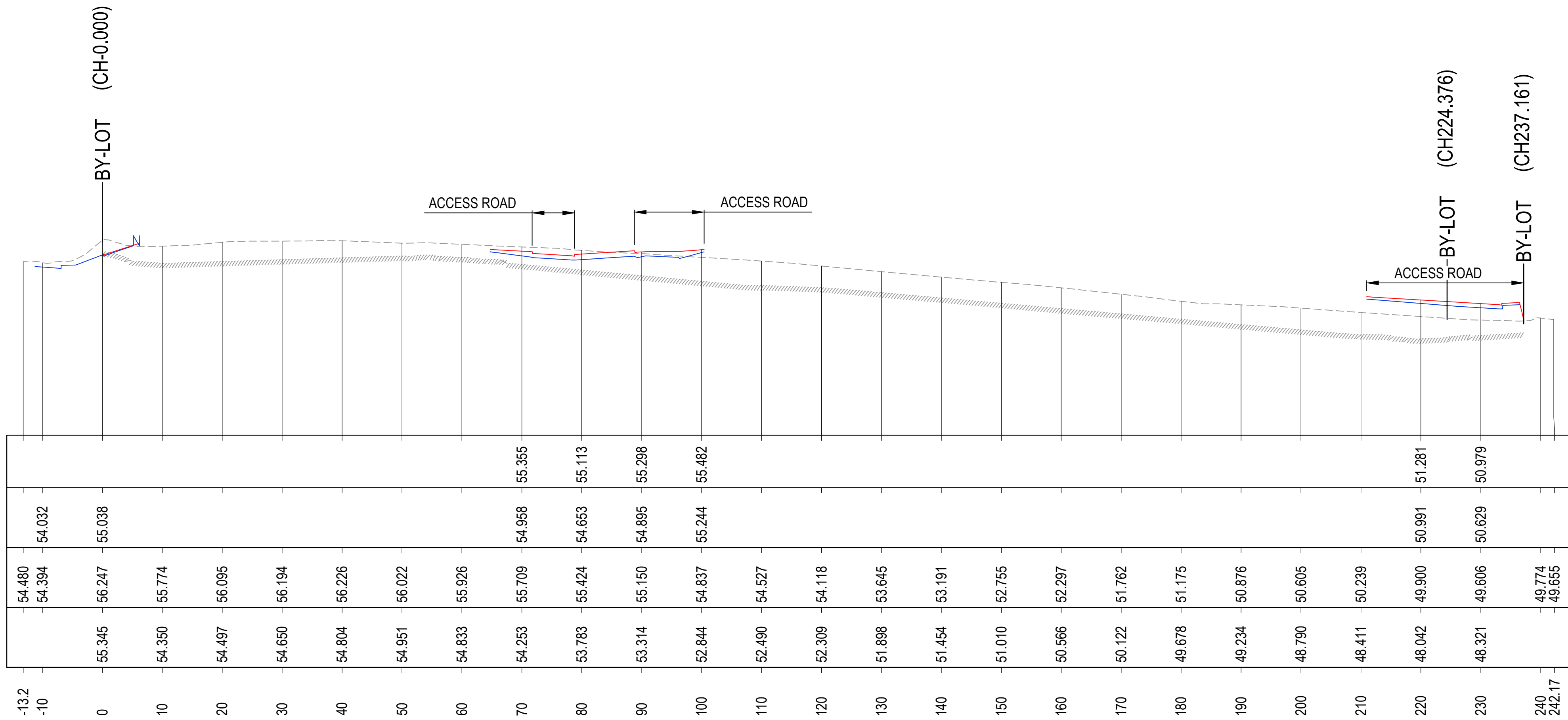
BULK EARTHWORKS SECTION - BE-A A1 Horizontal scale 1:500 A1 Vertical scale 1:250
