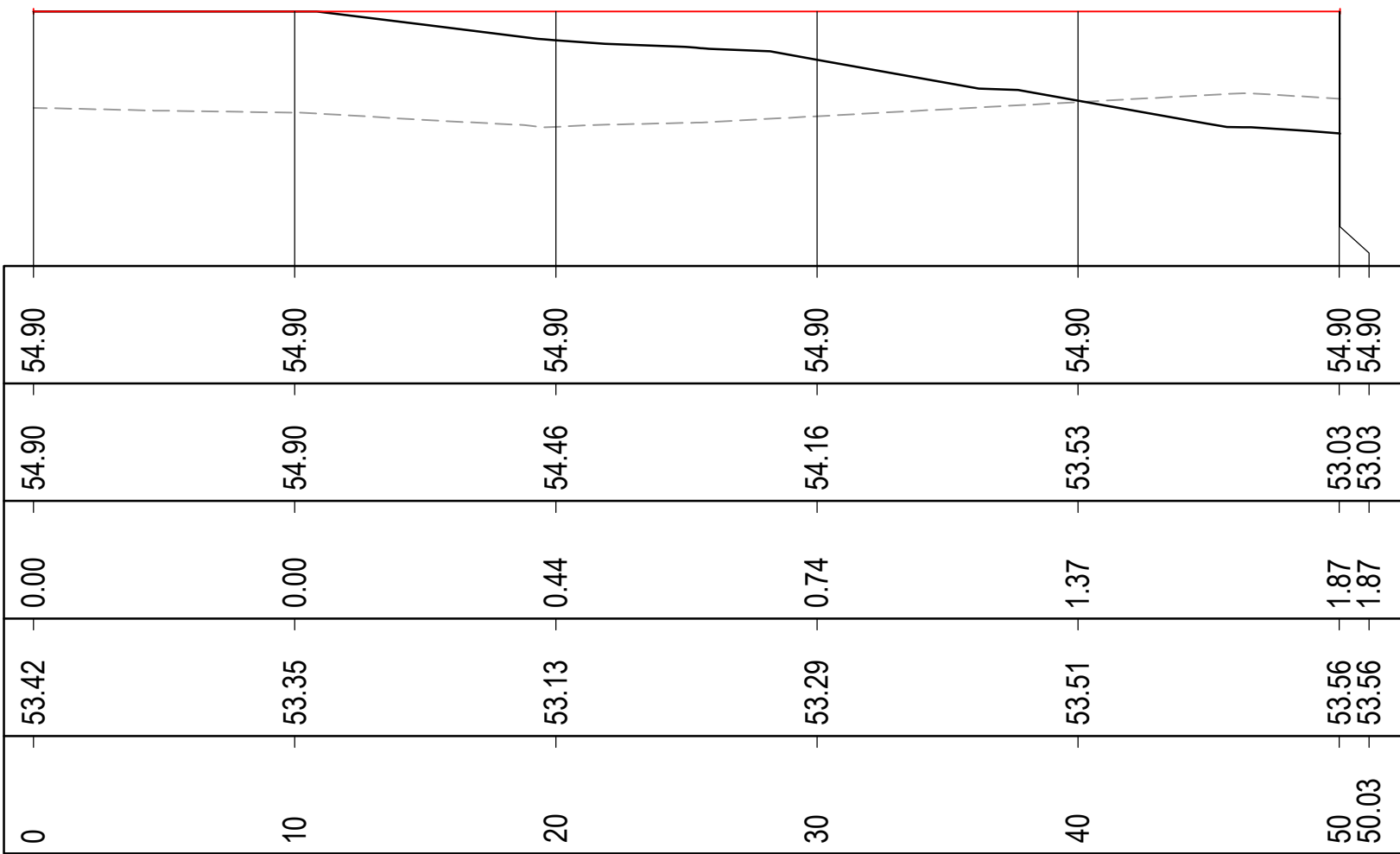
RETAINING WALL ELEVATION - MW09
