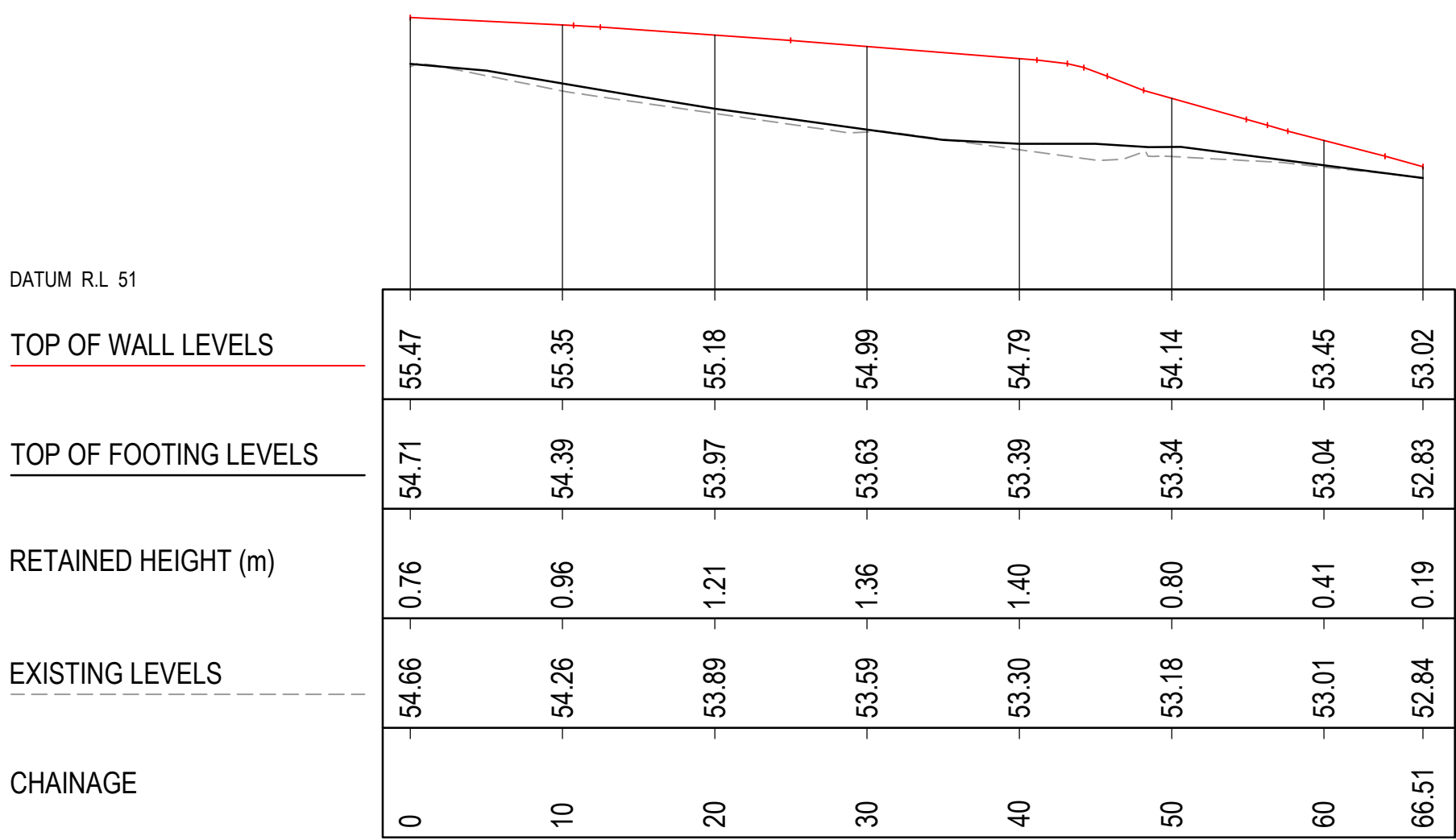
RETAINING WALL ELEVATION - MW04
