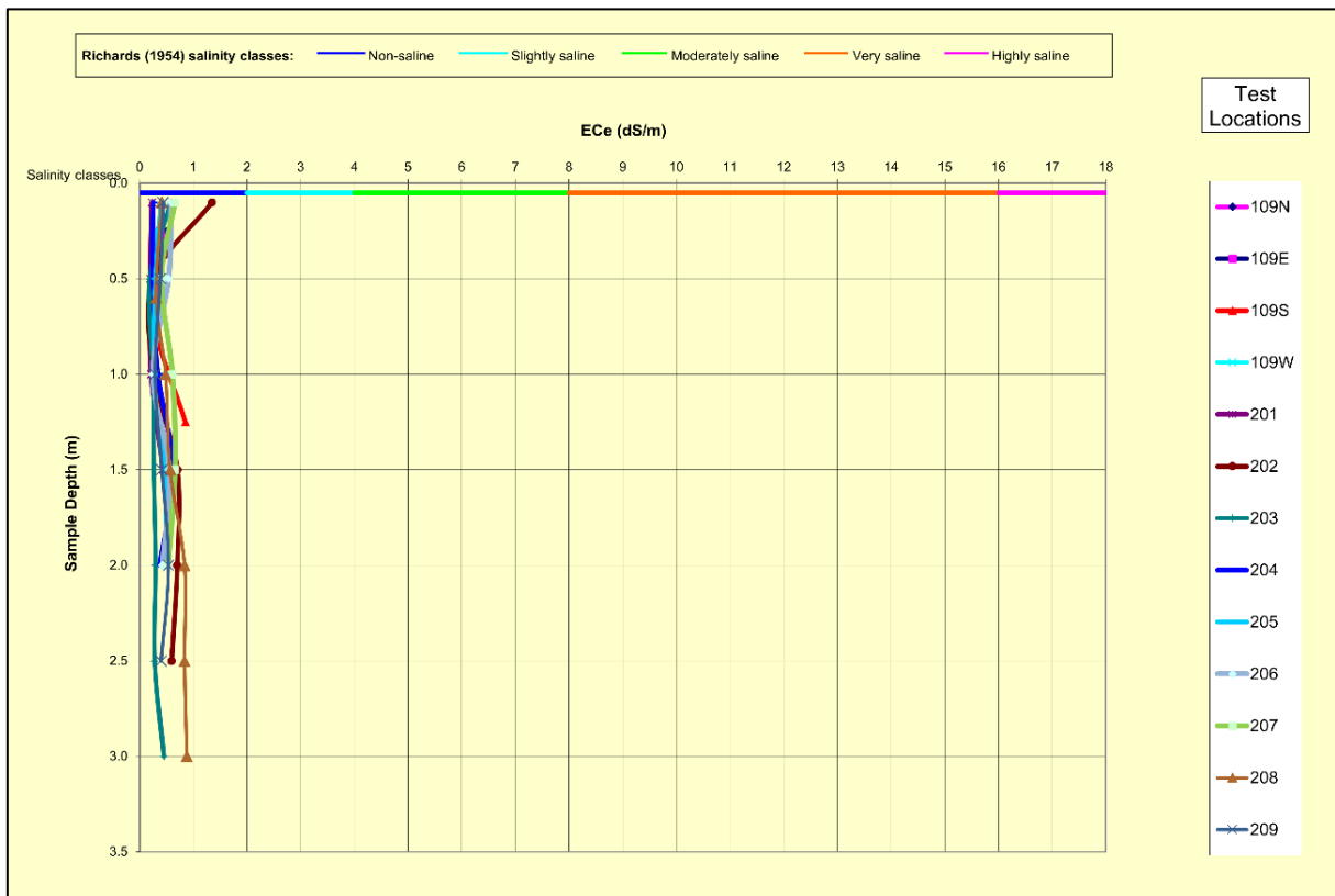
Figure 2: Vertical Soil Salinity Profiles and Salinity Classes
