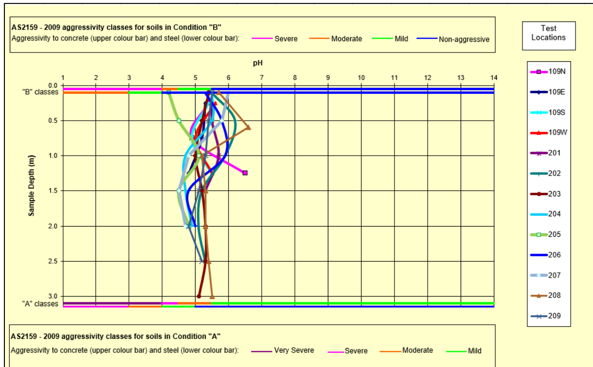
Figure 1: Vertical Soil pH Profiles and Aggressivity Classes
