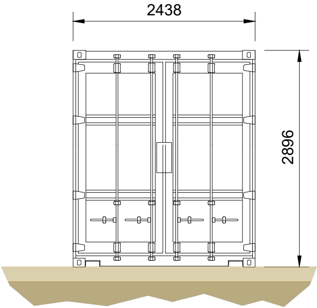
2 Elevation - front view M 1:50
