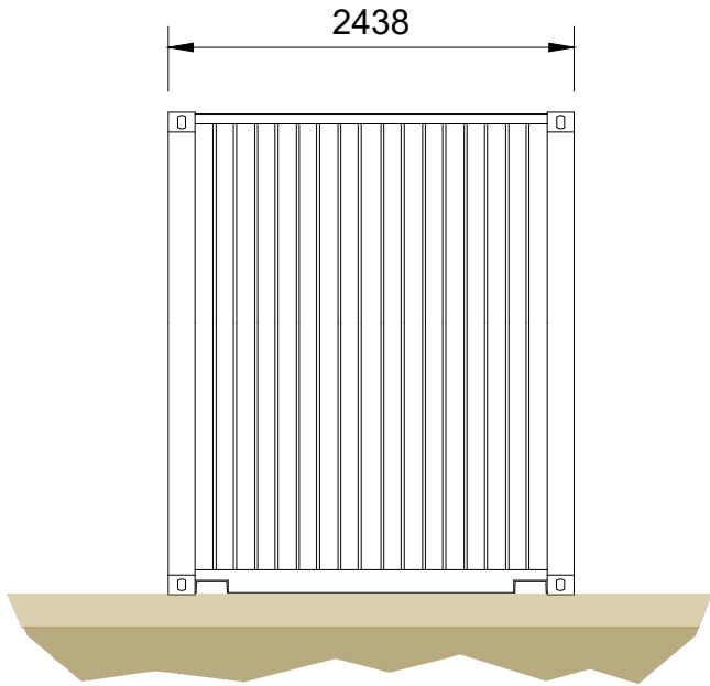
4 Elevation - back view M 1:50
