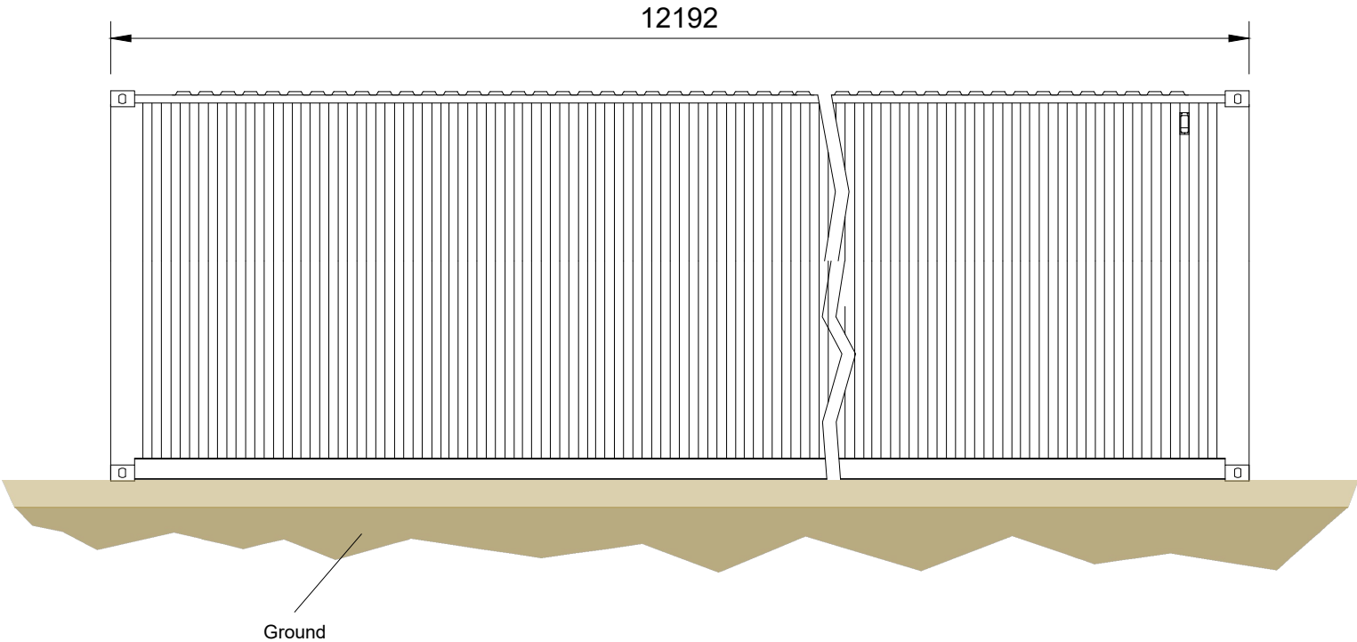
3 Elevation - side view M 1:50
