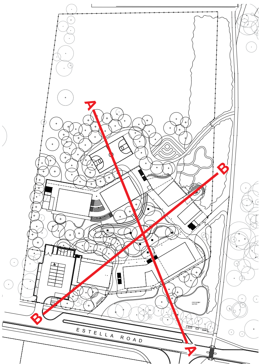
KEY PLAN
