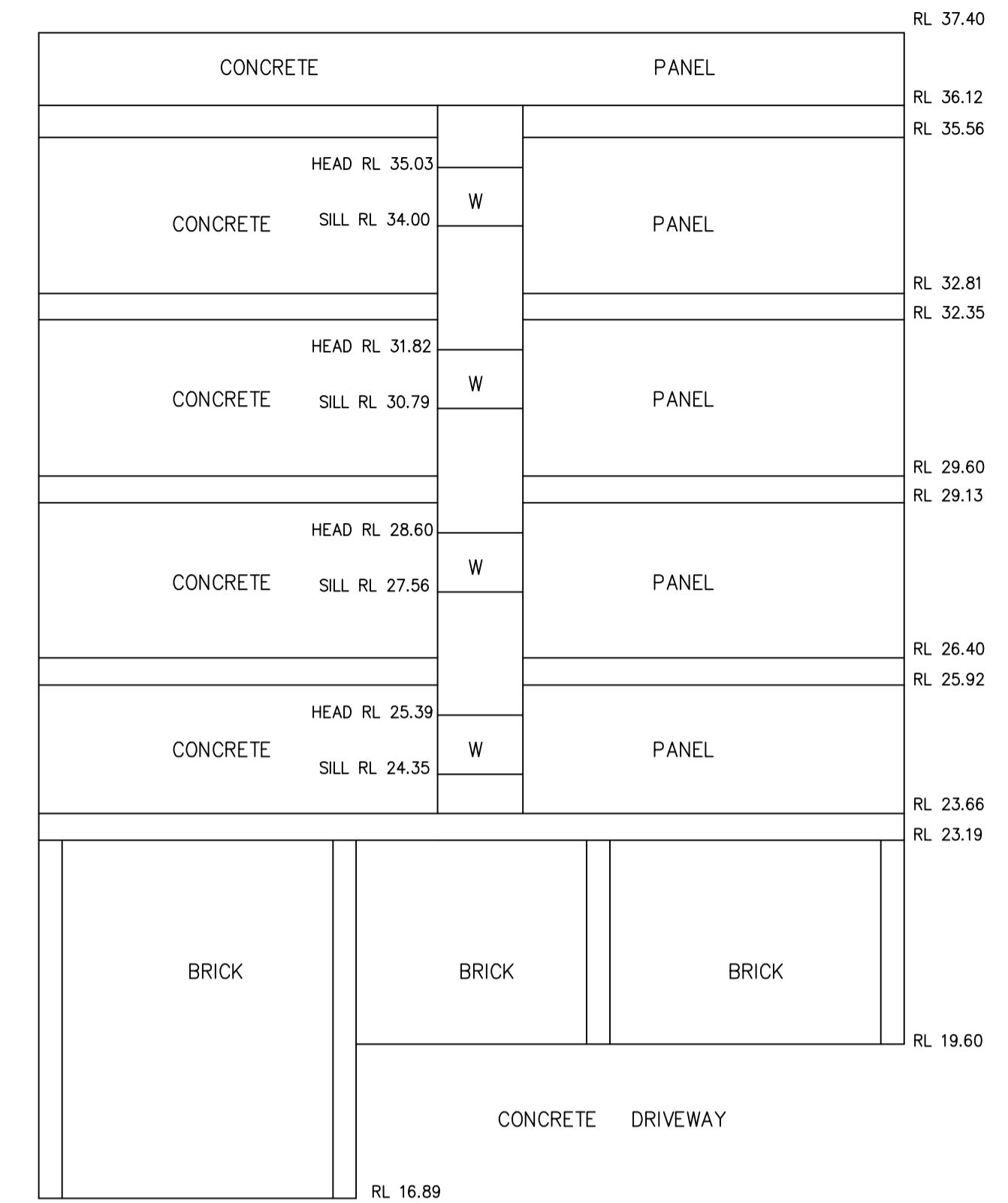
NORTHERN ELEVATION SPIRIT HOUSE SCALE 1 : 100
