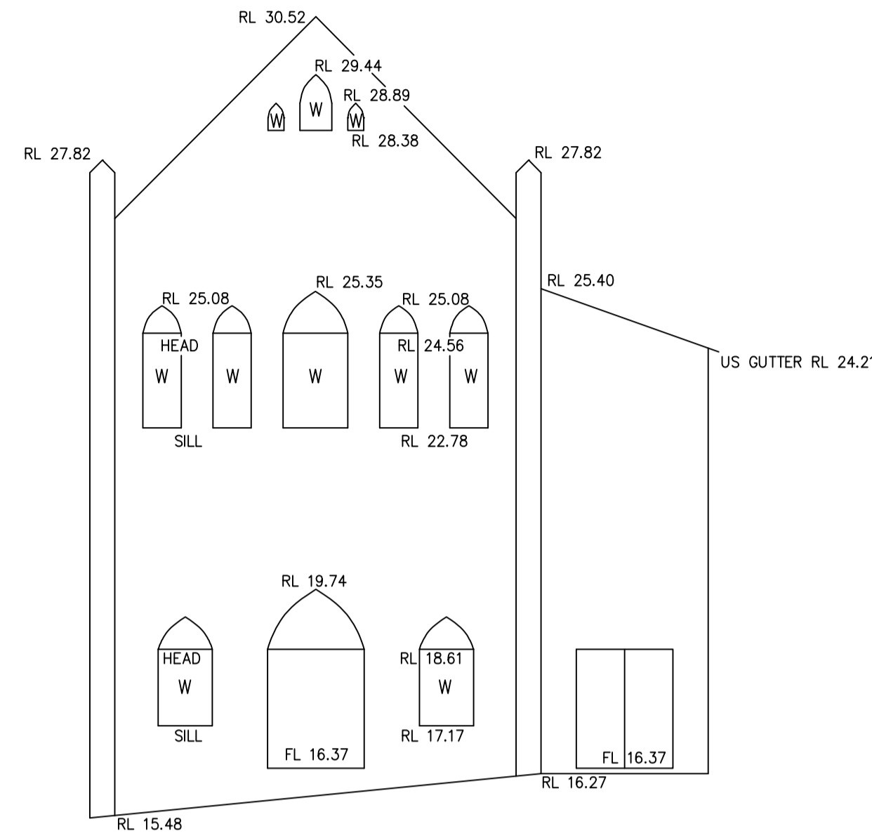
NORTHERN ELEVATION NATIONAL SCHOOL BUILDING SCALE 1 : 100
