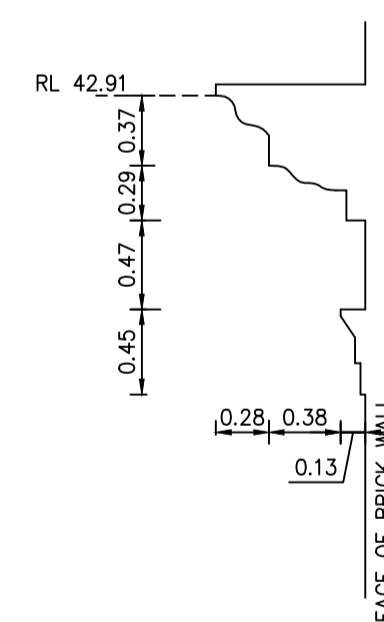
DIAGRAM 1 DETAIL OF EXTERNAL CORNICE ON EASTERN ELEVATION VERNON WING SCALE 1 : 25
