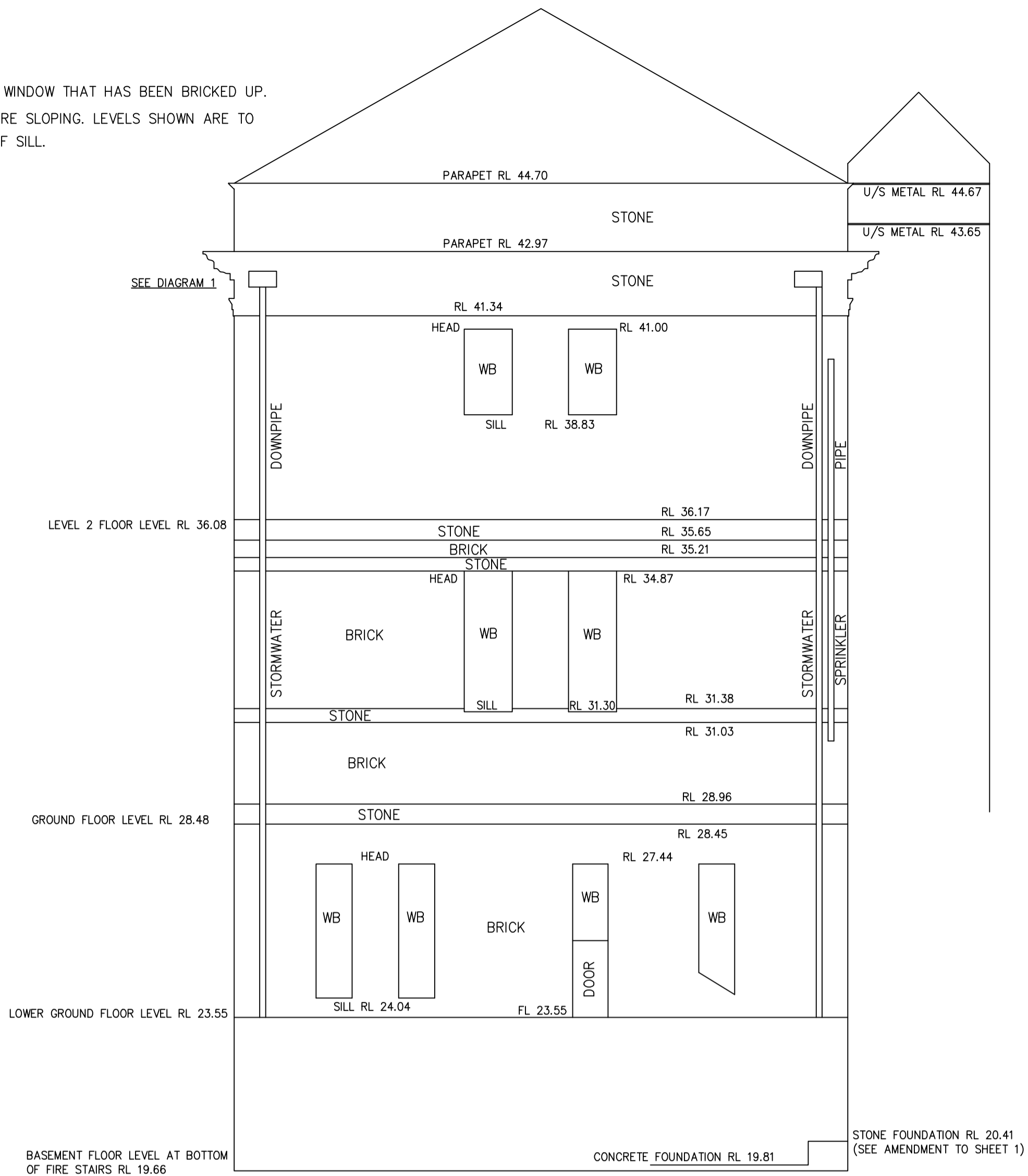
EASTERN ELEVATION VERNON WING SCALE 1 : 100
