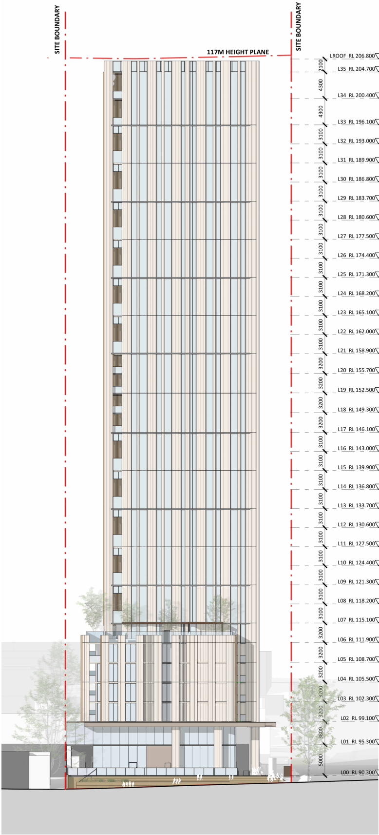
NORTH ELEVATION (1:600)
