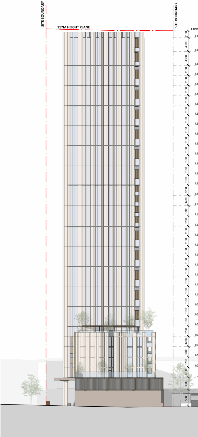
SOUTH ELEVATION (1:600)
