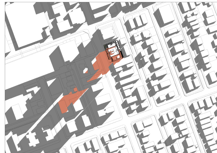
21 JUNE 0900 HRS
