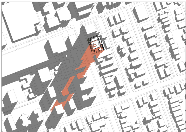
21 JUNE 1000 HRS
