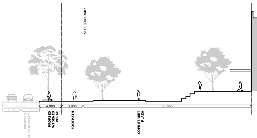
Figure 13 – Section B-B Cope Street Plaza
