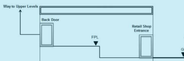
Figure 22 – Possible flood mitigation design
