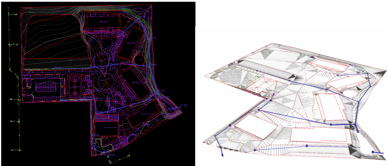
Figure 2: 12d model layout
