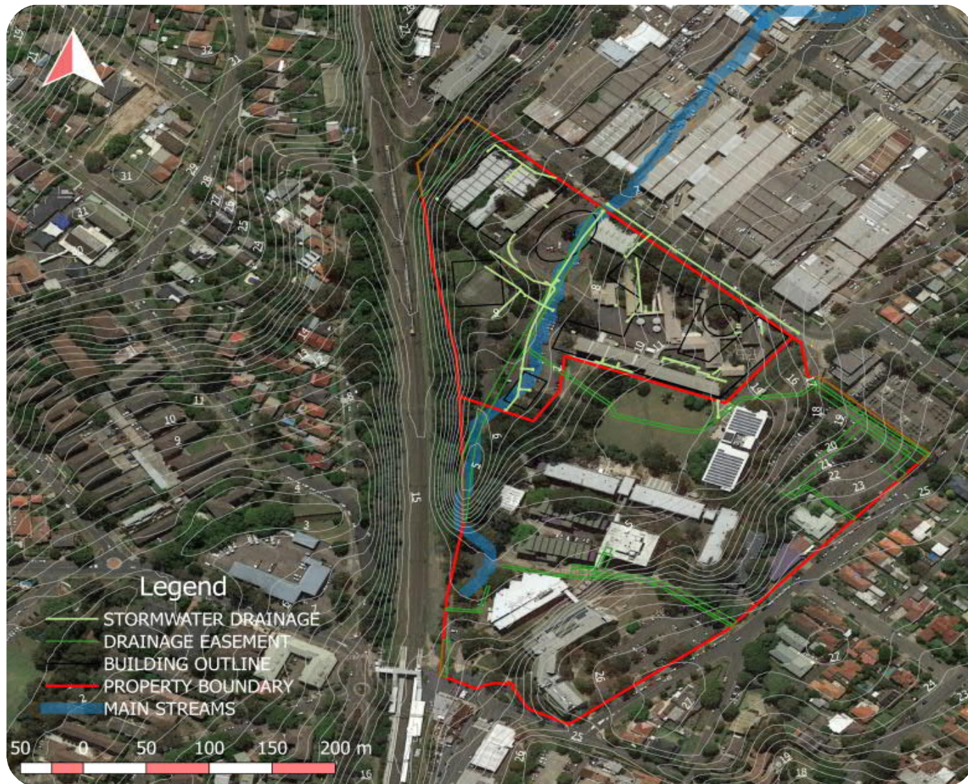
Figure 3. Existing site drainage
