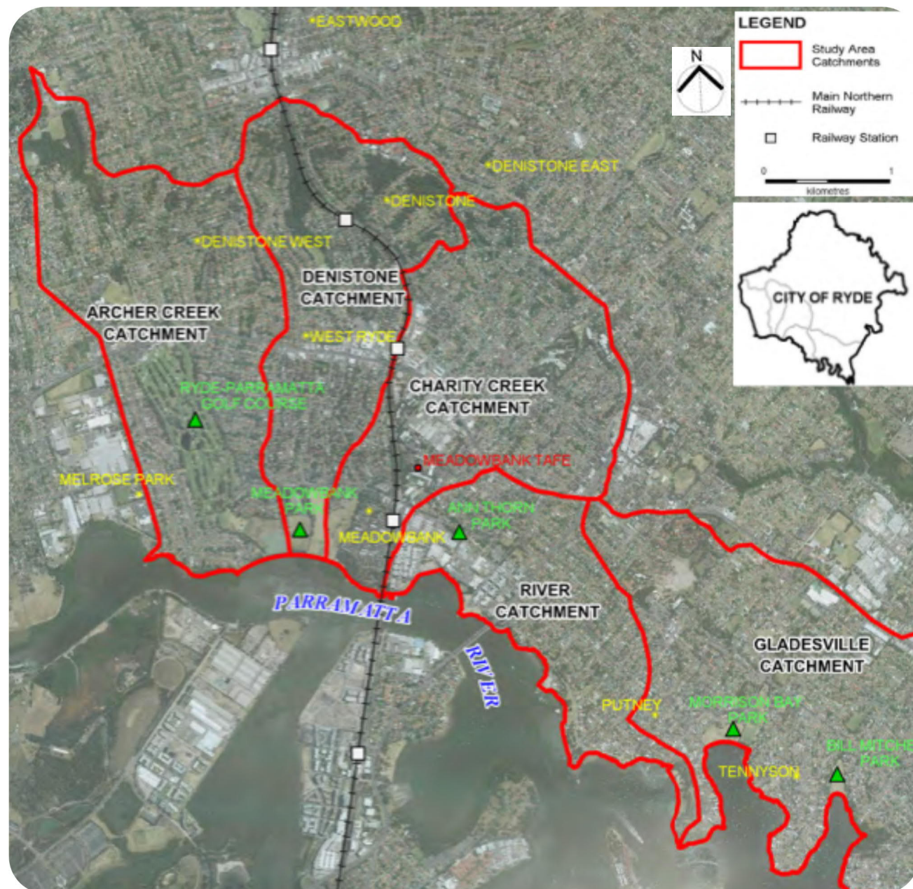
Figure 5. Charity Creek catchment (Source: City of Ryde Council)
