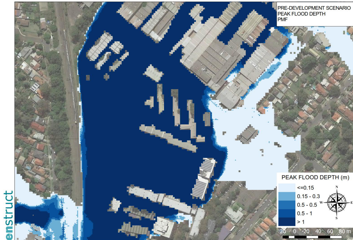
Figure 9. Overland flooding under existing conditions for PMF event
