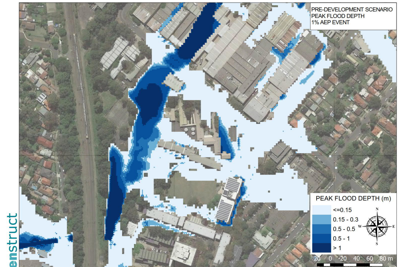
Figure 8. Overland flooding under existing conditions for 1% AEP event
