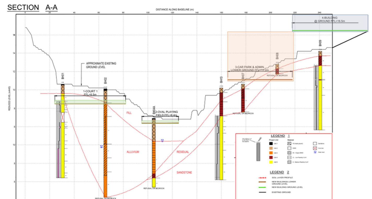
Figure 10. Interpreted geological model for site
