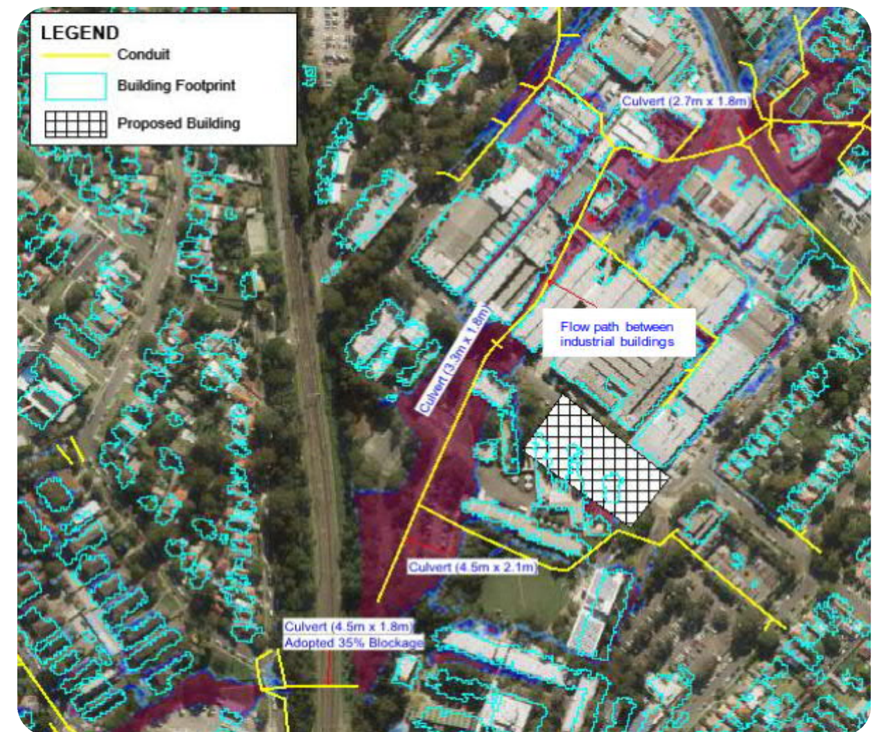
Figure 6. Key drainage structures (Source: ARUP)
