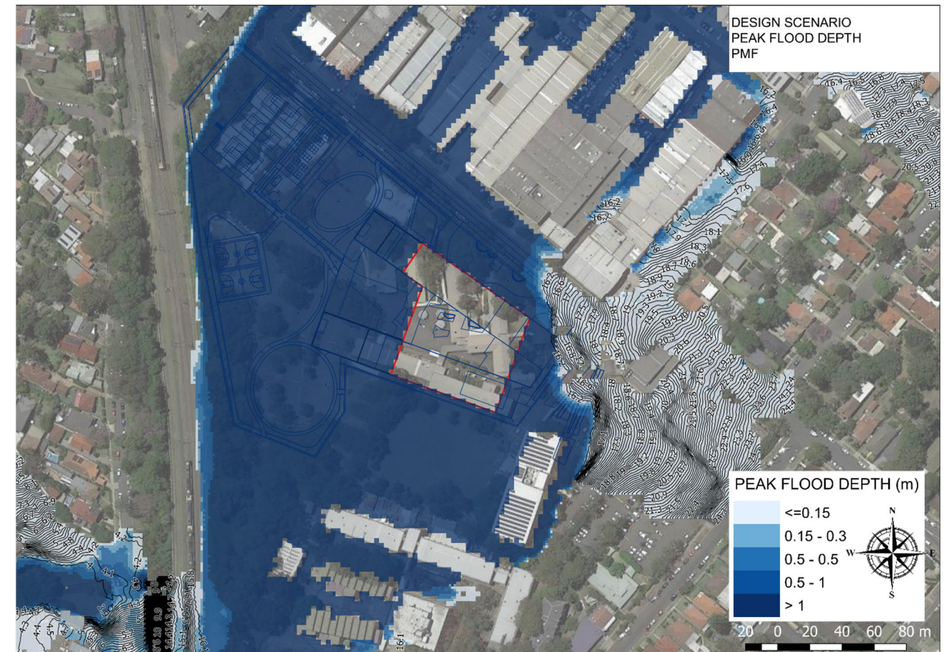
Figure 14. Overland flooding under post-development conditions for PMF event
