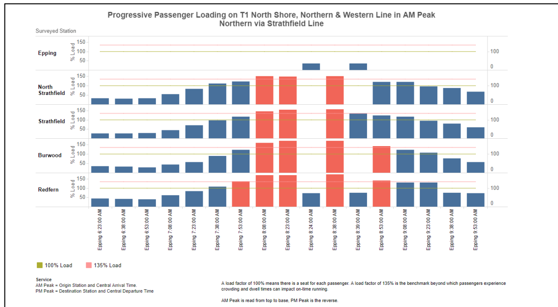
Figure 3.10: Train Loads Survey for T1 Line
