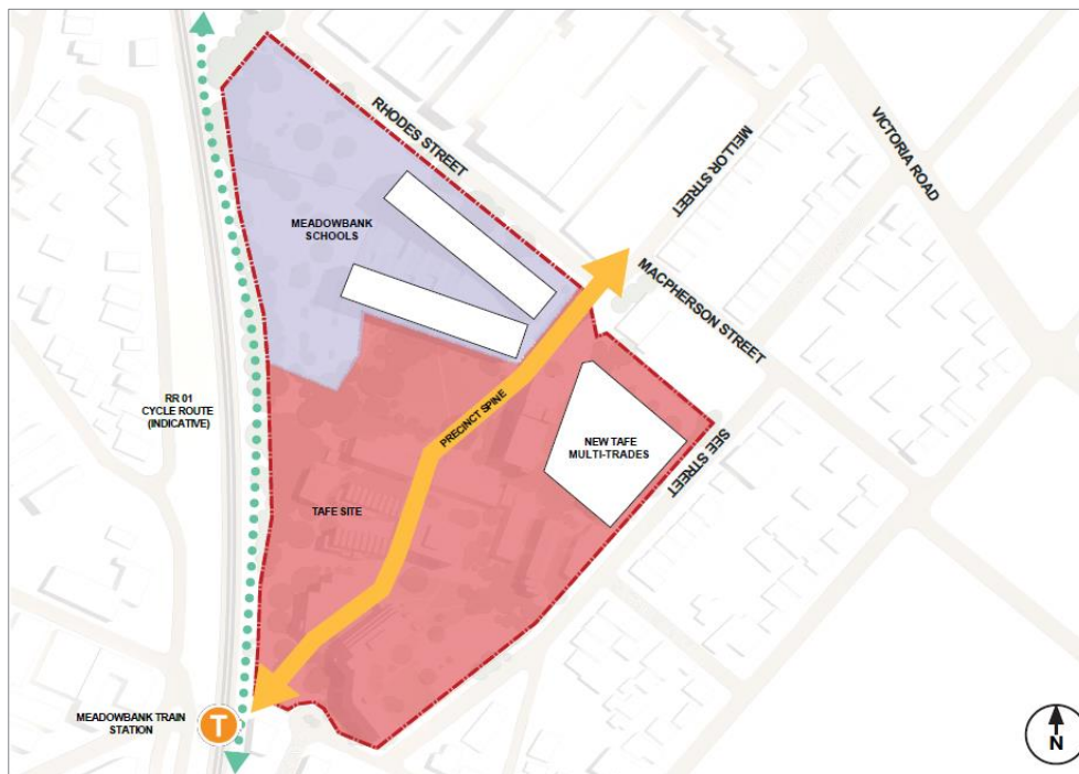
Figure 4.1: Indicative site layout plan
