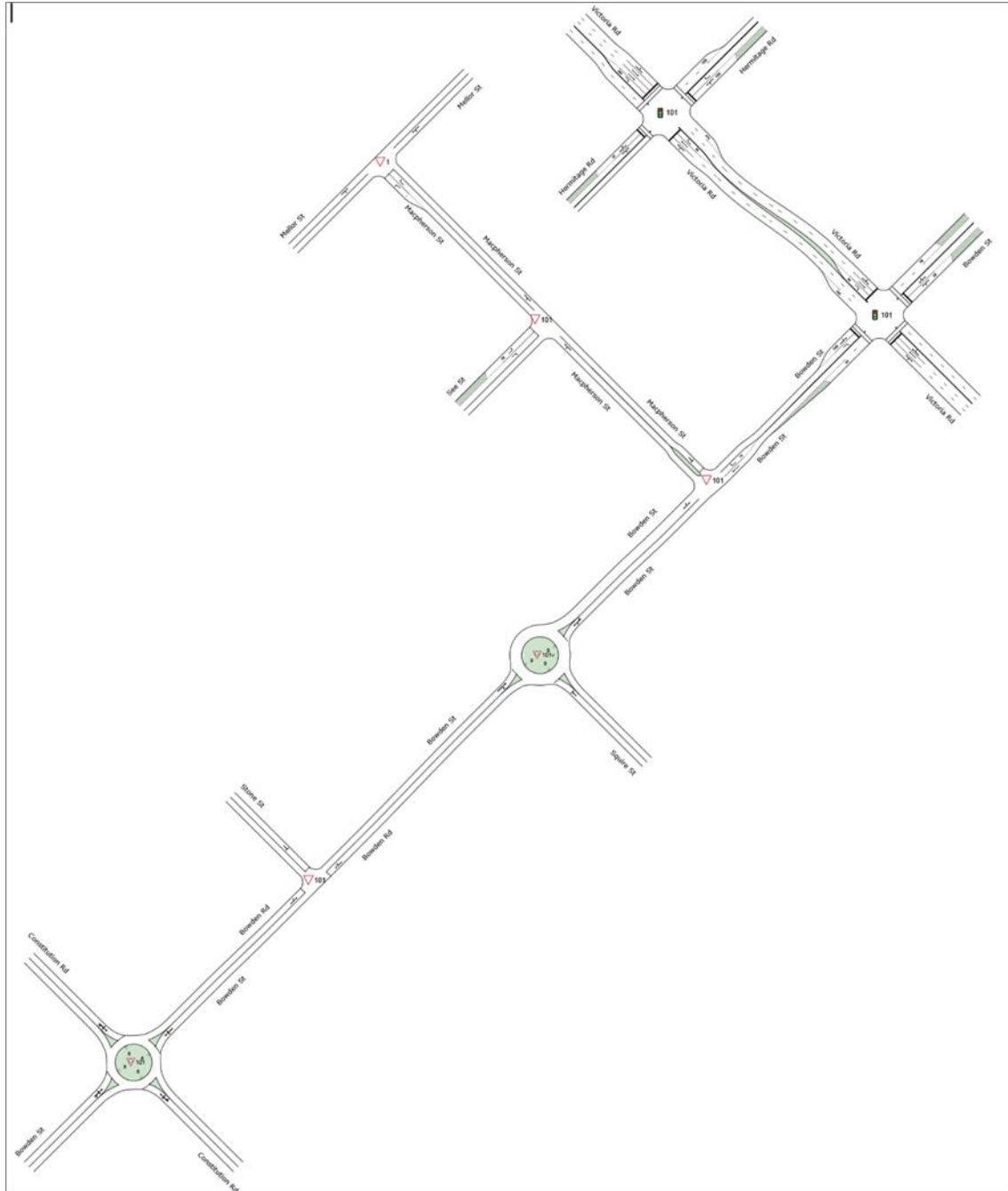
Figure 9.1: Existing intersection layouts - SIDRA Network
