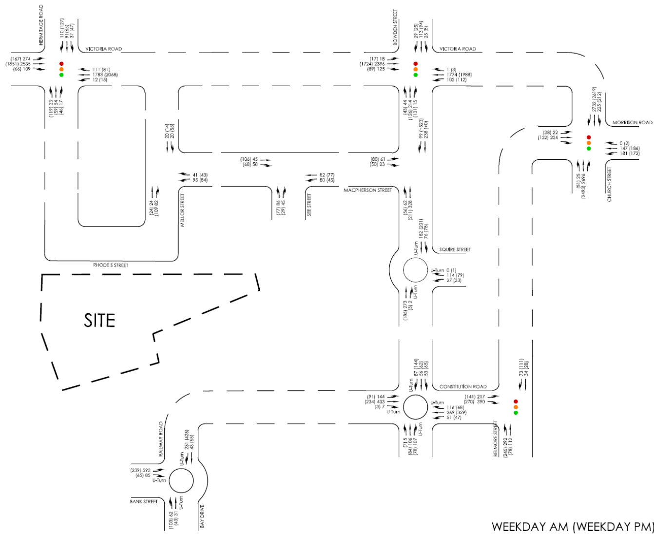
Figure 3.9: Existing AM/ PM school peak hour traffic volumes
