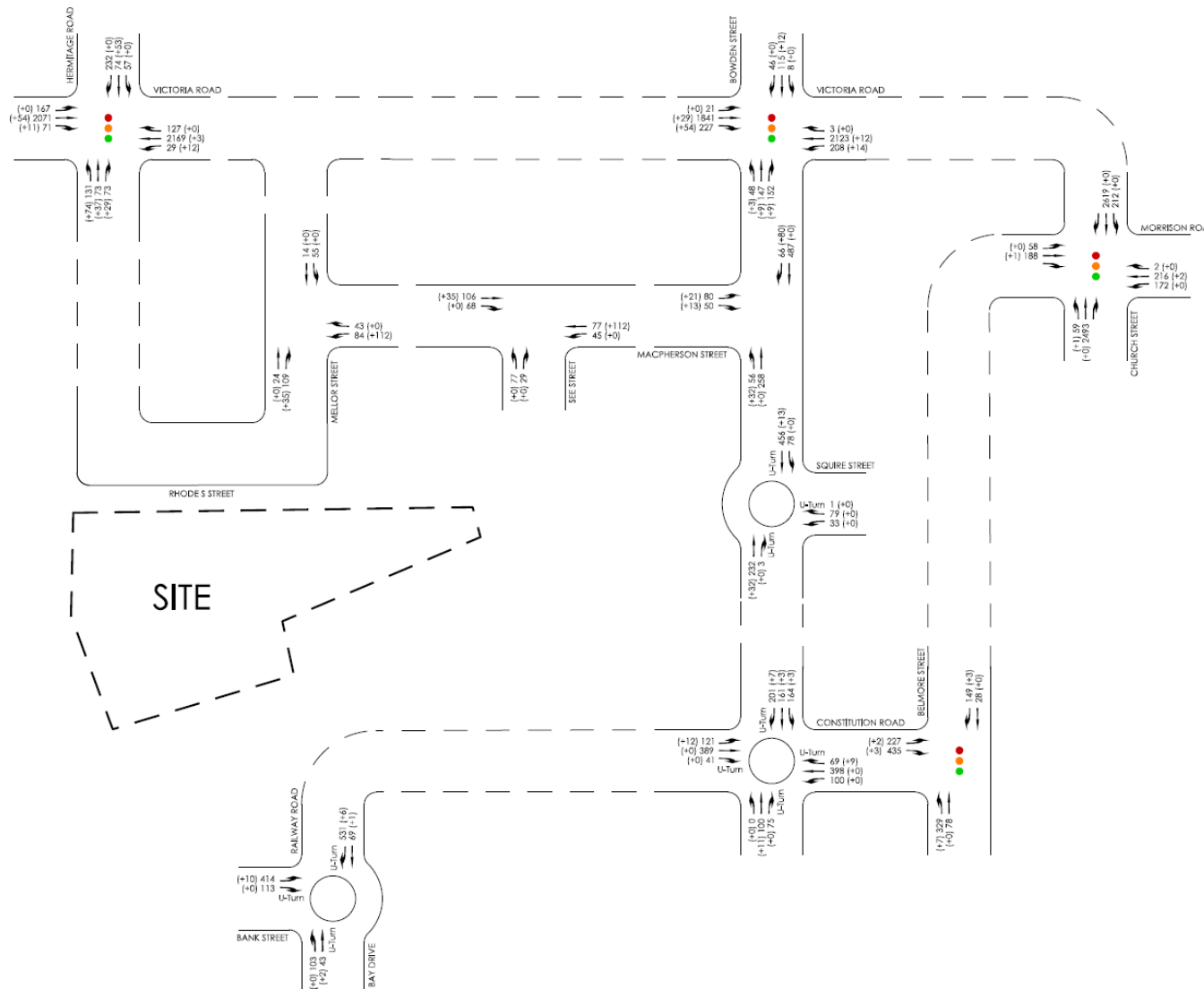
Figure 9.7: PM peak hour site generated traffic volumes – PM (+School)
