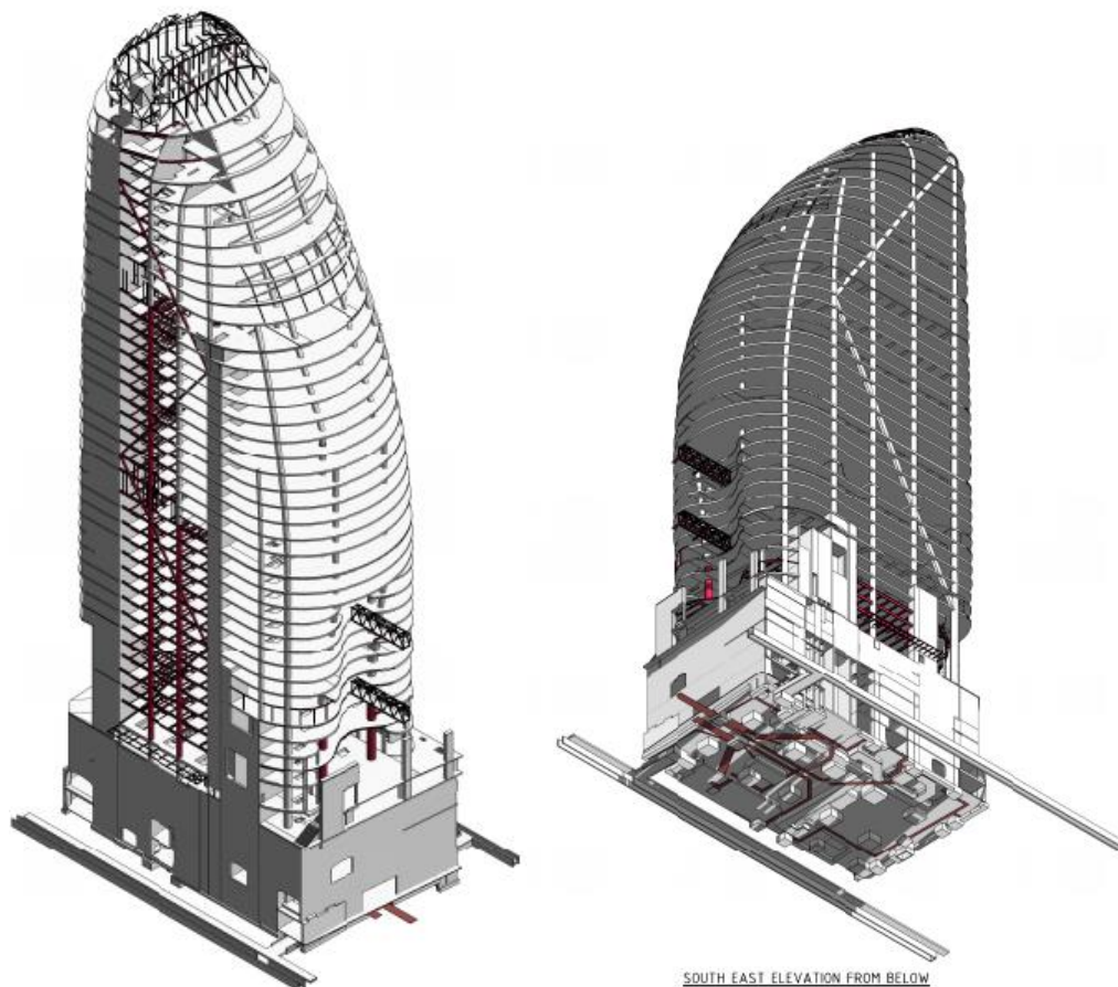
Figure 4: North Tunnel and station structure perspectives describing an integrated design from foundation level to rooftop including a view of the new tunnels adjacent the shaft and the foundation soffits.
