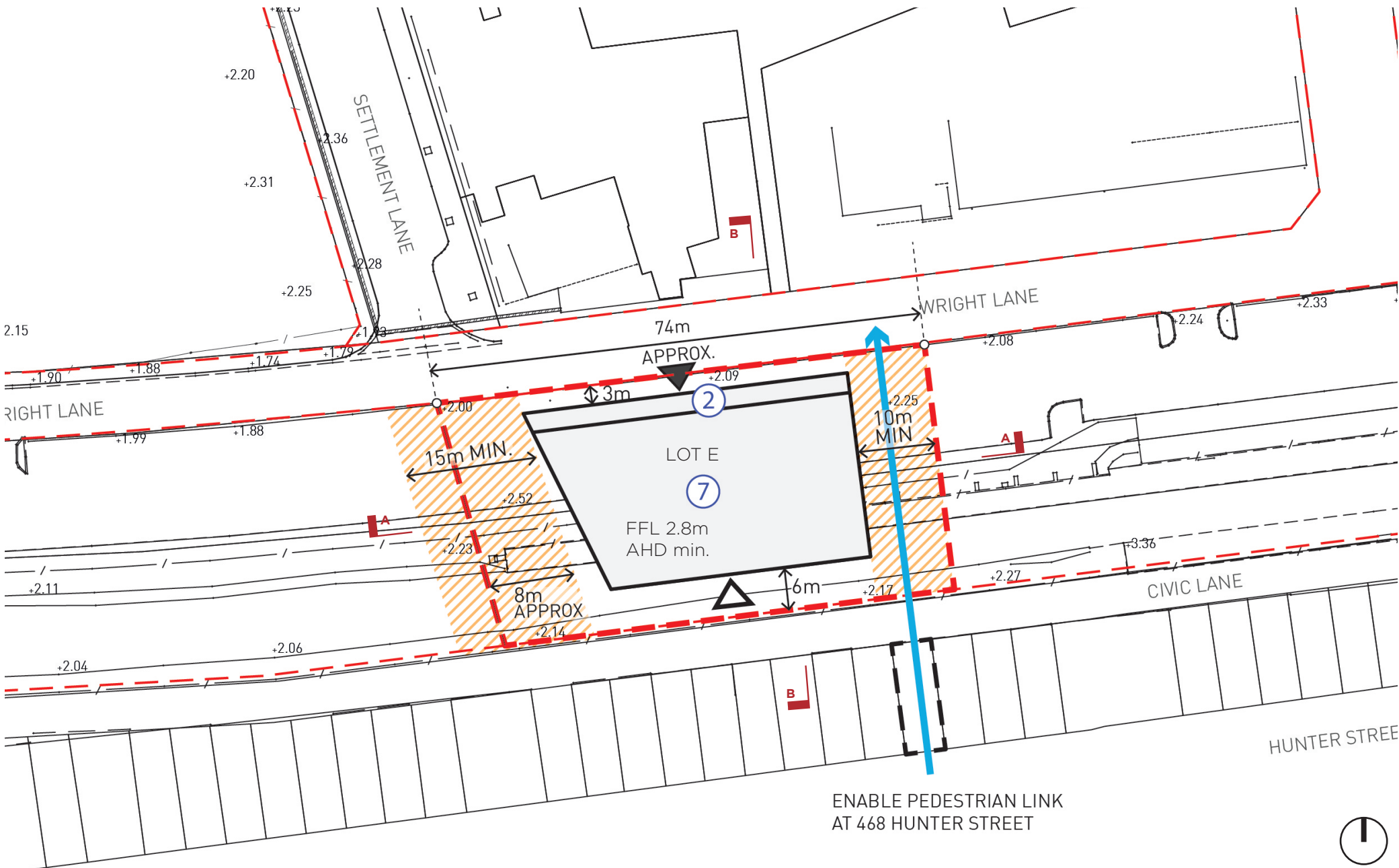
Figure 7.16 Lot E Detail Plan
