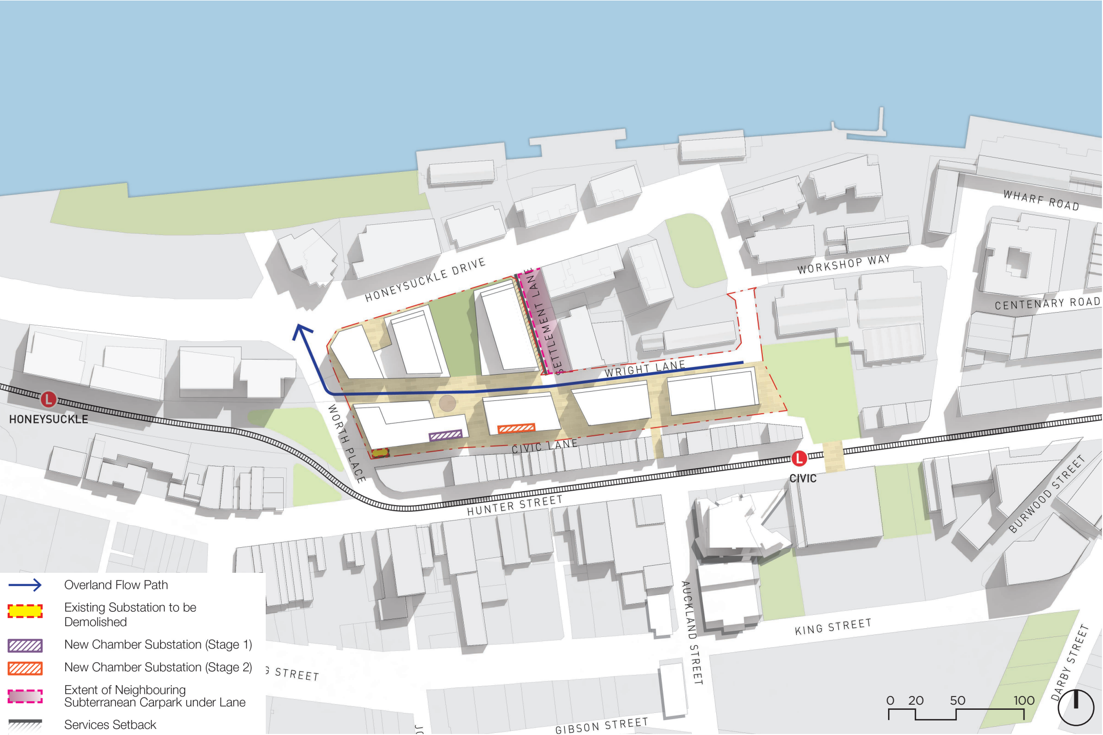
Figure 3.8 Site Infrastructure Diagram
