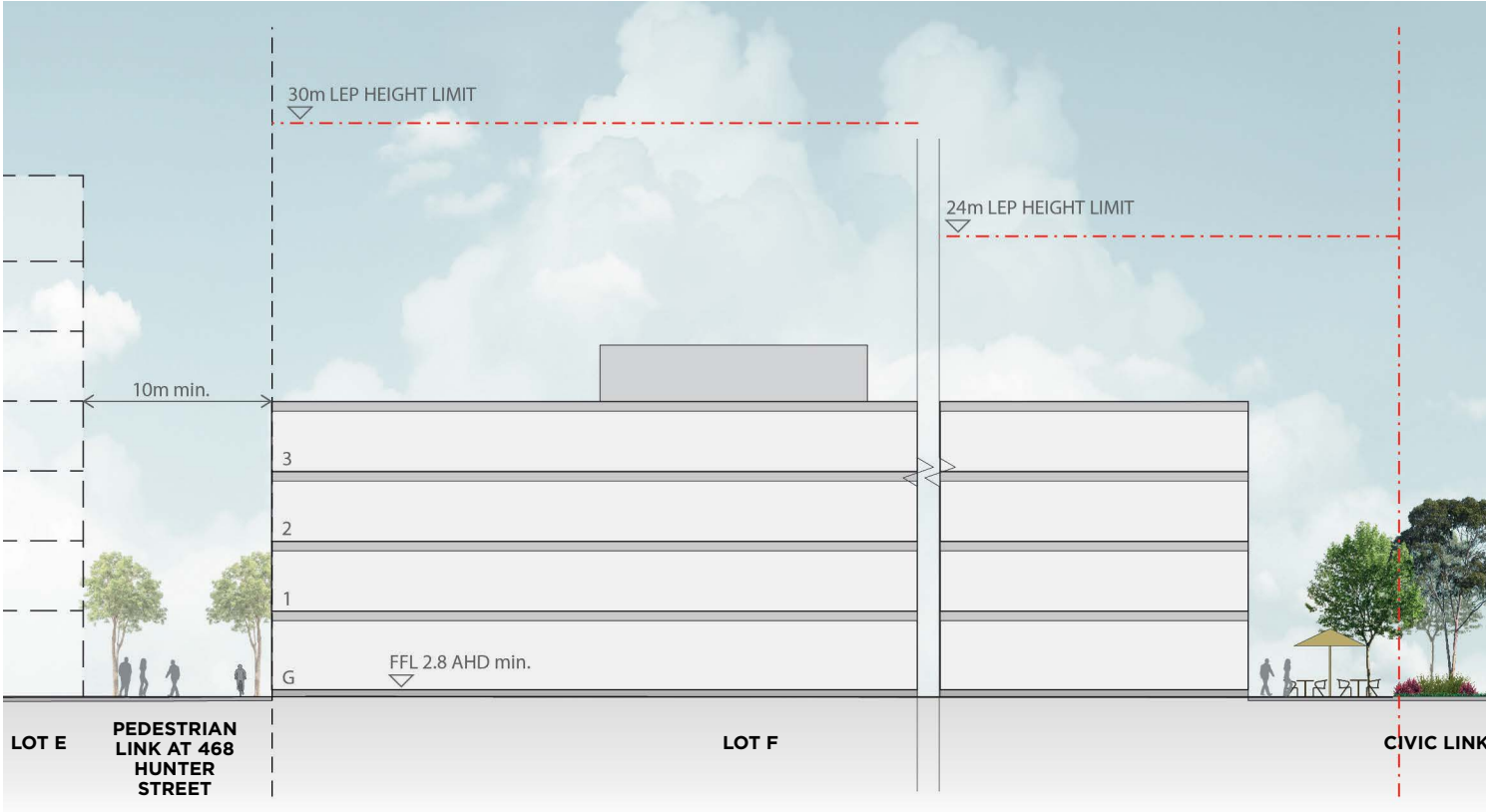
Section A Figure 7.20 Lot F Sections
