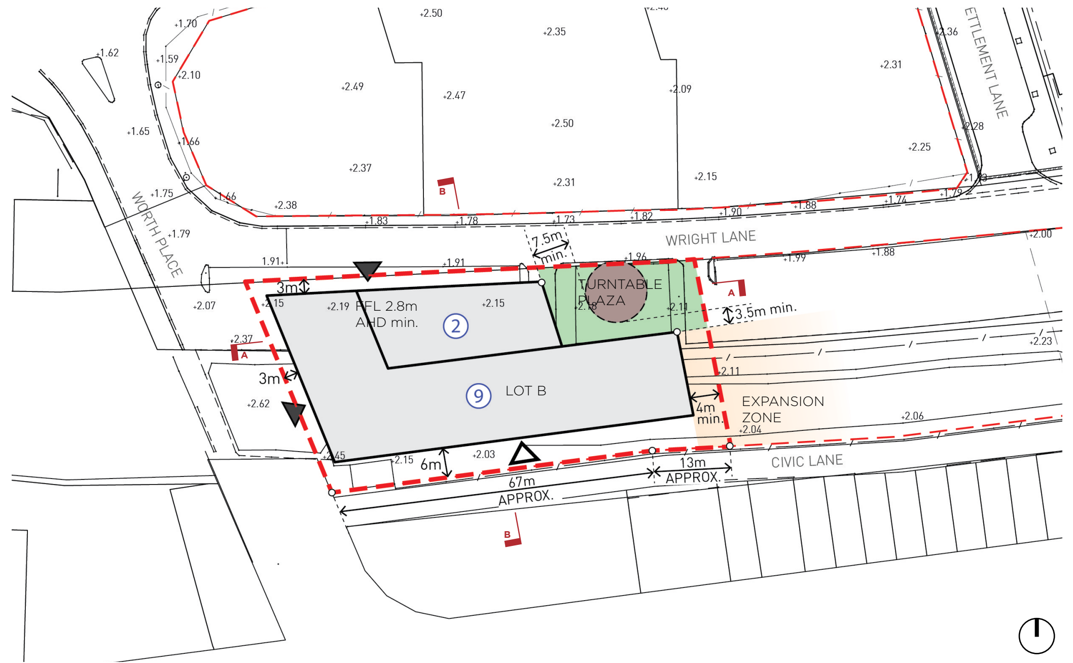
Figure 7.7 Lot B Detail Plan
