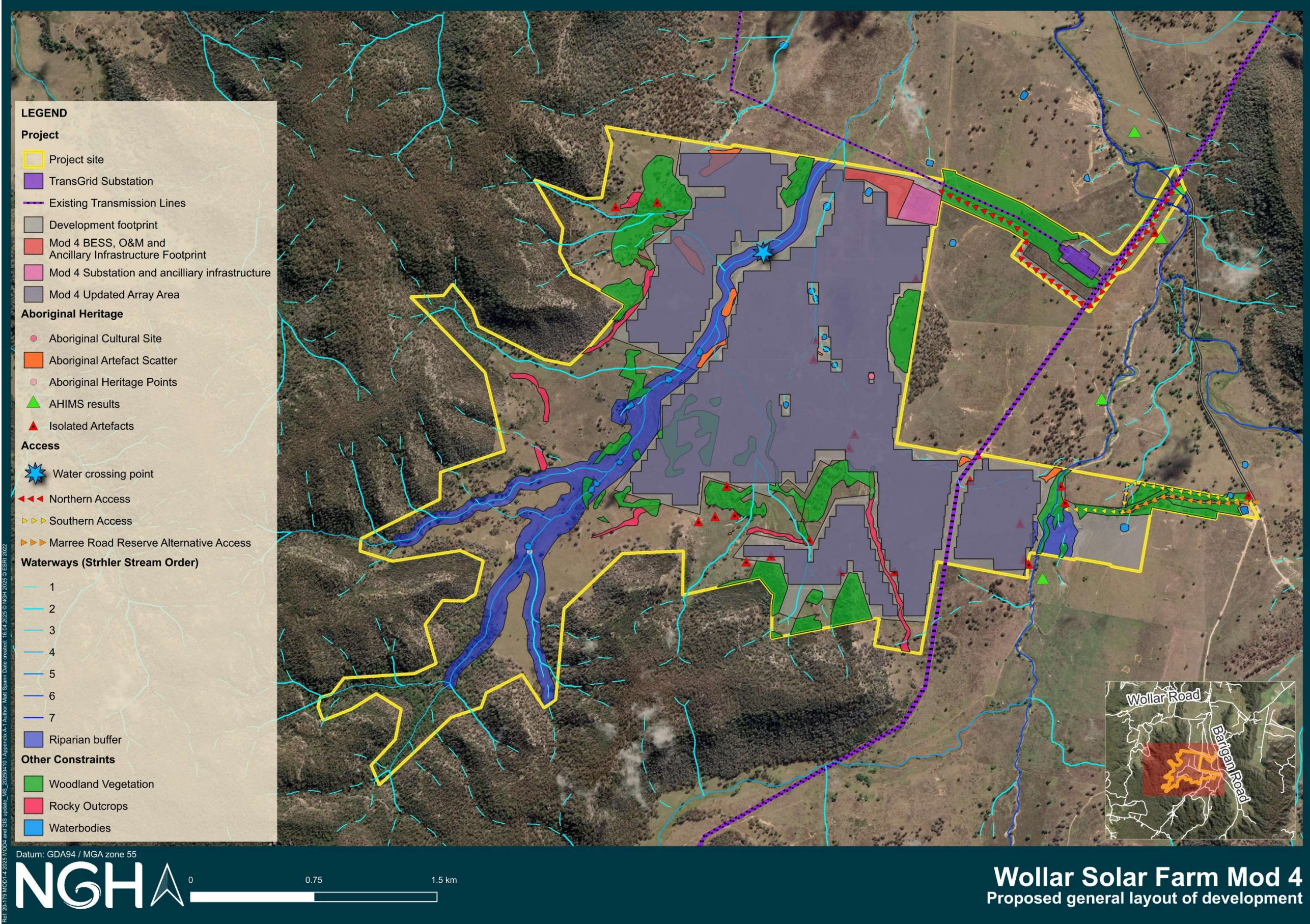
Figure A-11 Wollar Solar Farm proposed Development Footprint and Infrastructure layout
