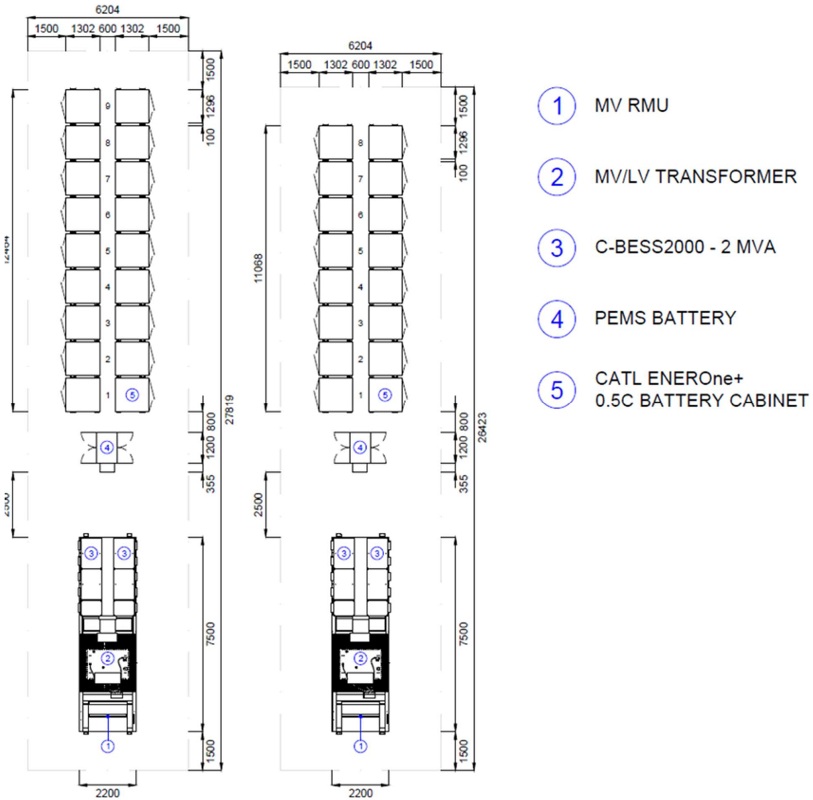
Figure A-13 Module layout for the Wollar BESS if using the modular setup
