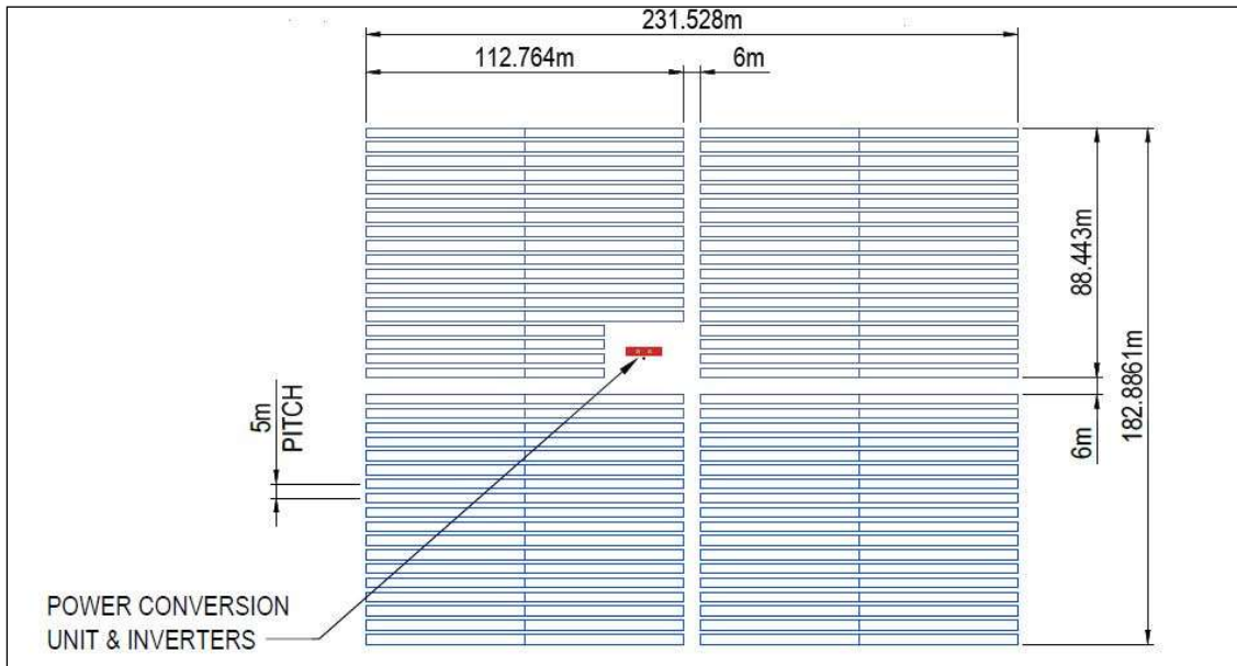
Figure A-5 Typical array block showing location of PCU.
