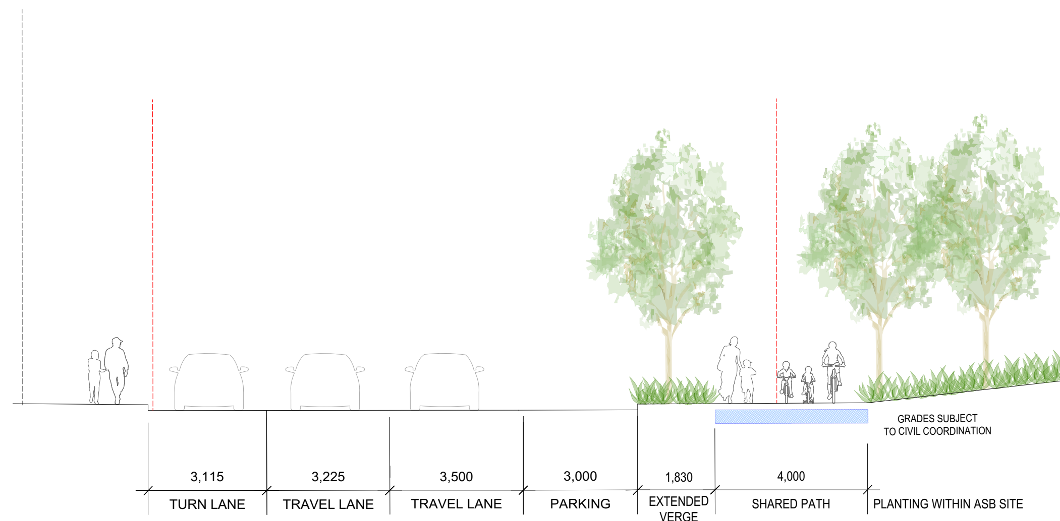
1 Botany St Section Scale 1:100
