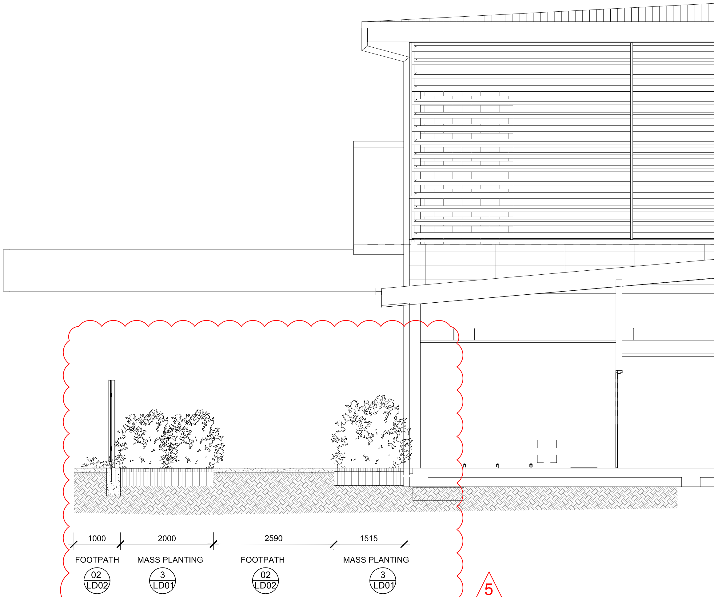
B-B MOTHER AND BABIES COURTYARD SECTION 1:250
