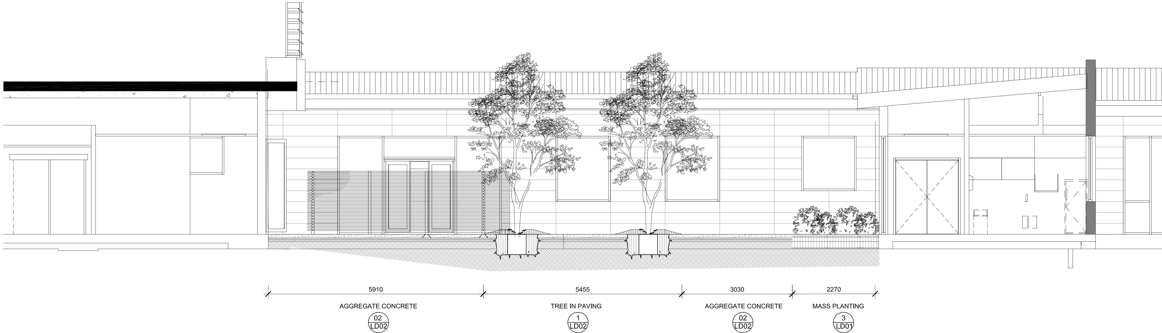
A-A CENTRAL COURTYARD SECTION 1:50
