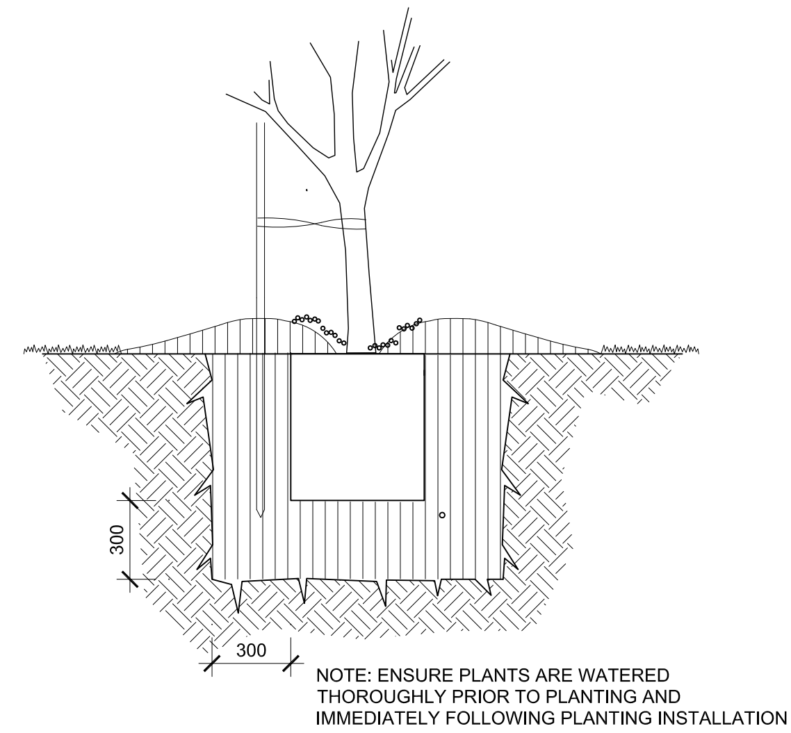
3 TREE IN GRASS TYPICAL SECTION 1:20
