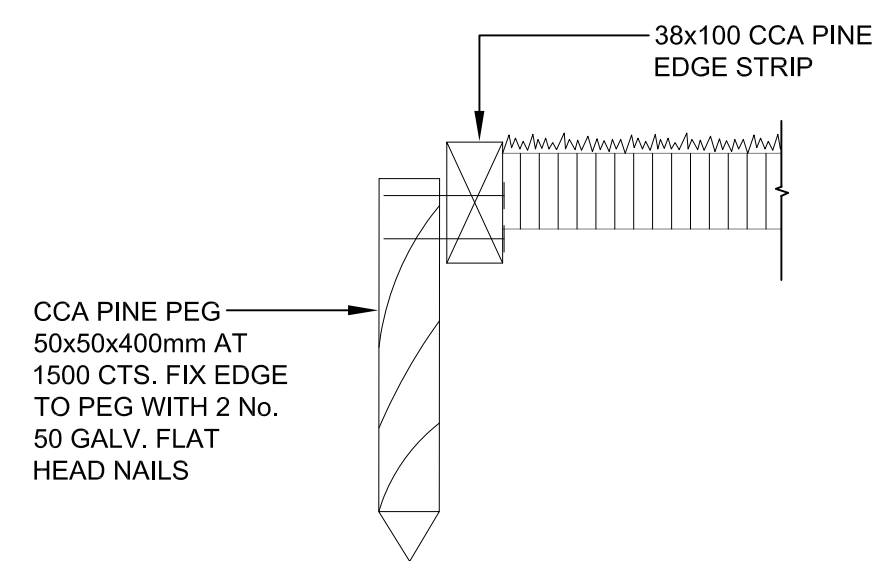
2A TIMBER EDGE TYPICAL DETAIL
