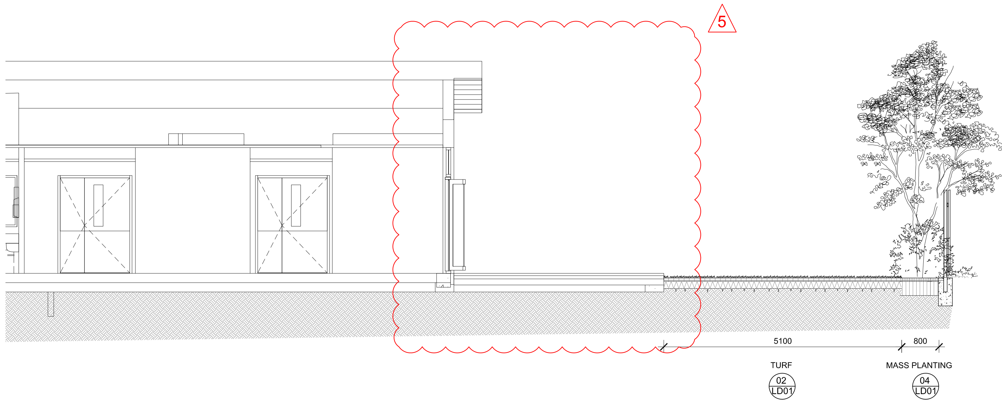
D-D NORTH EAST SECURE COURTYARD SECTION 1:250
