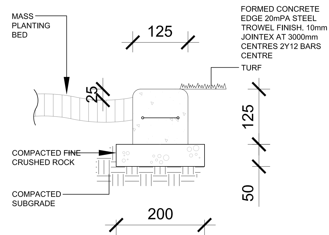
2B CONCRETE EDGE TYPICAL SECTION 1:5
