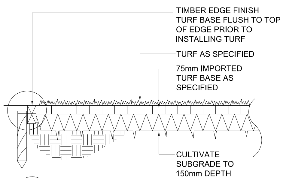
2 TURF TYPICAL SECTION 1:20
