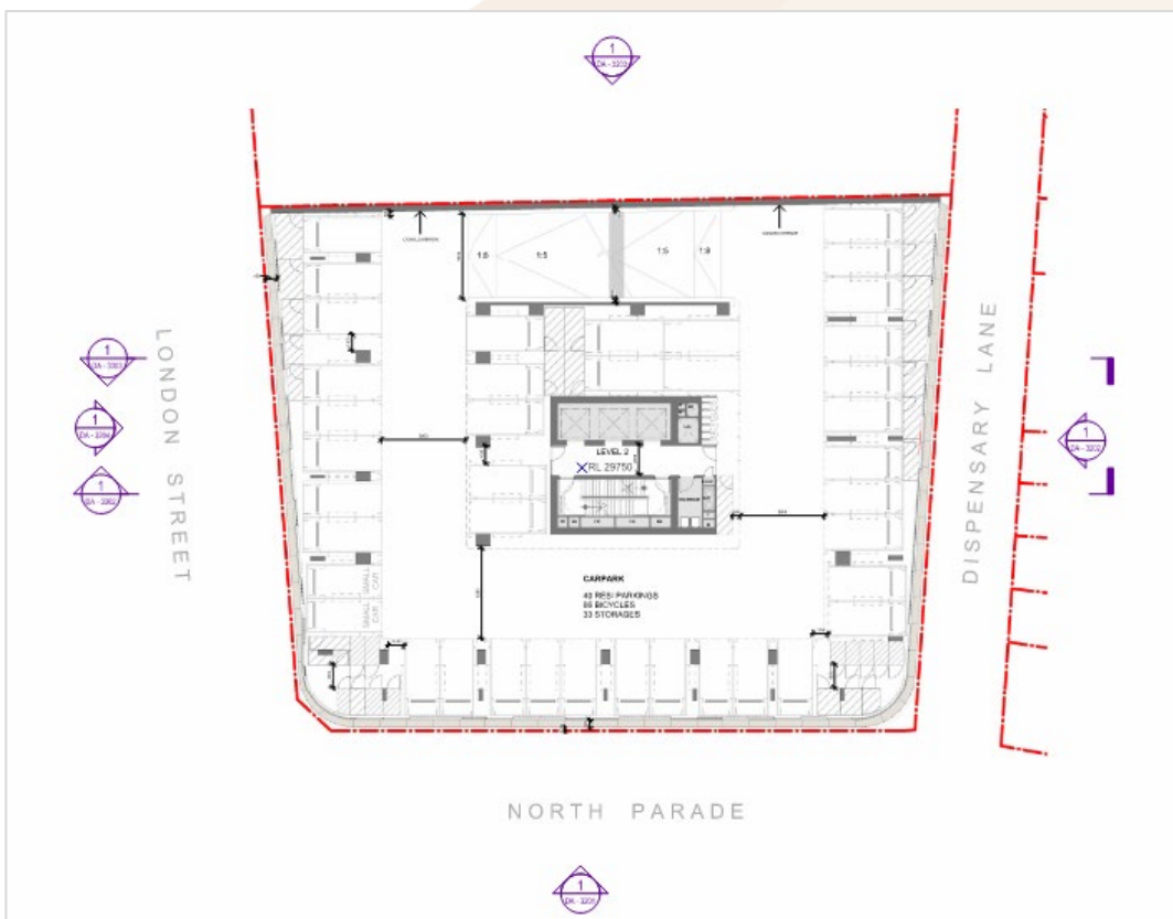
Figure 2.3 – Level 2 plan
