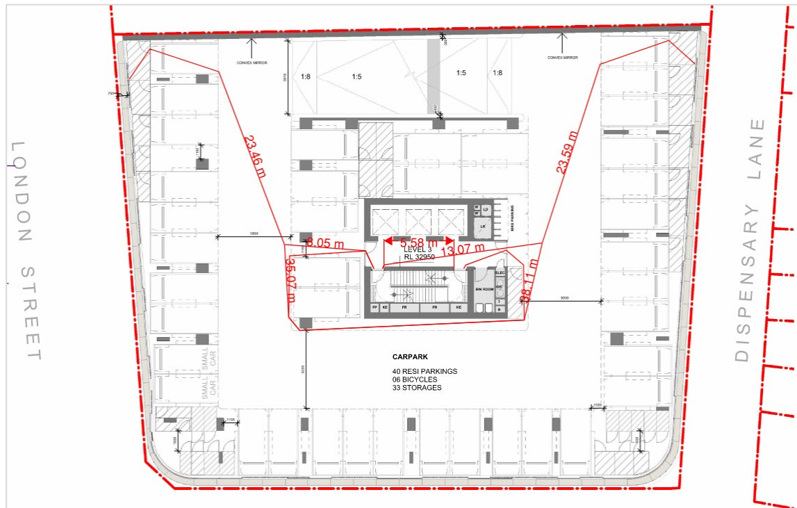
Figure 5.4 – Level 3 exit travel distances
