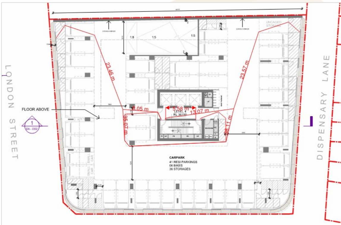
Figure 5.5 – Level 4 exit travel distances
