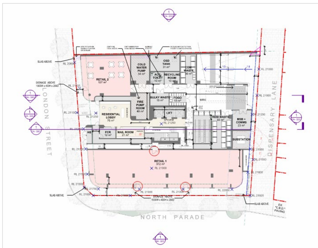
Figure 2.1 – Ground floor plan
