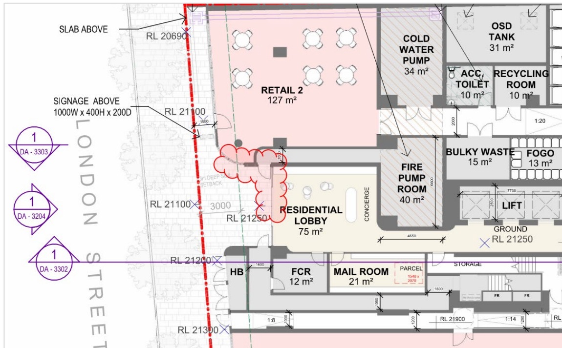
Figure 5.1 – Exposure between different fire compartments on ground floor
