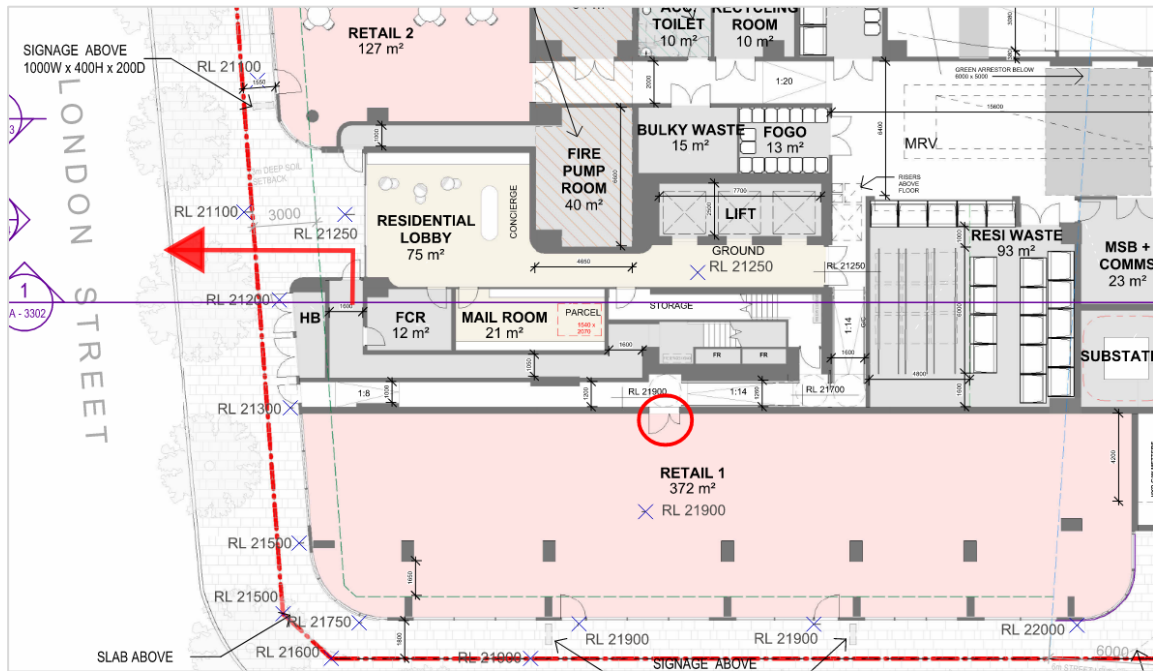
Figure 5.7 – Ground floor part plan
