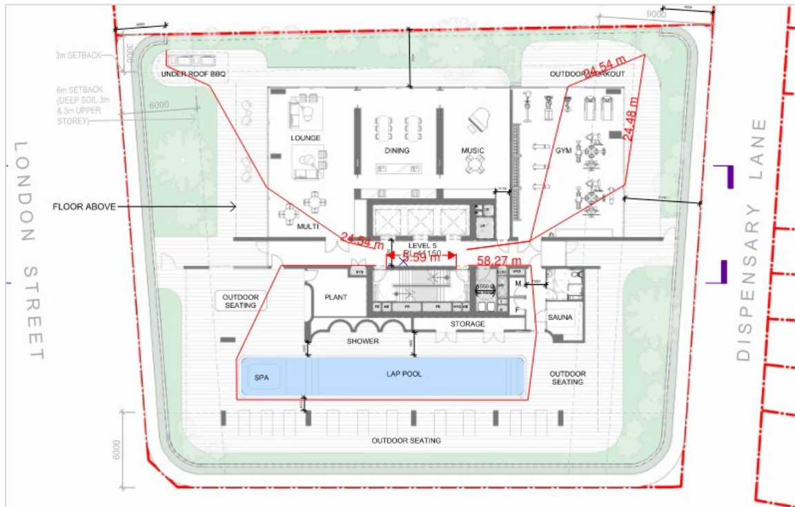
Figure 5.6 – Level 5 exit travel distances
