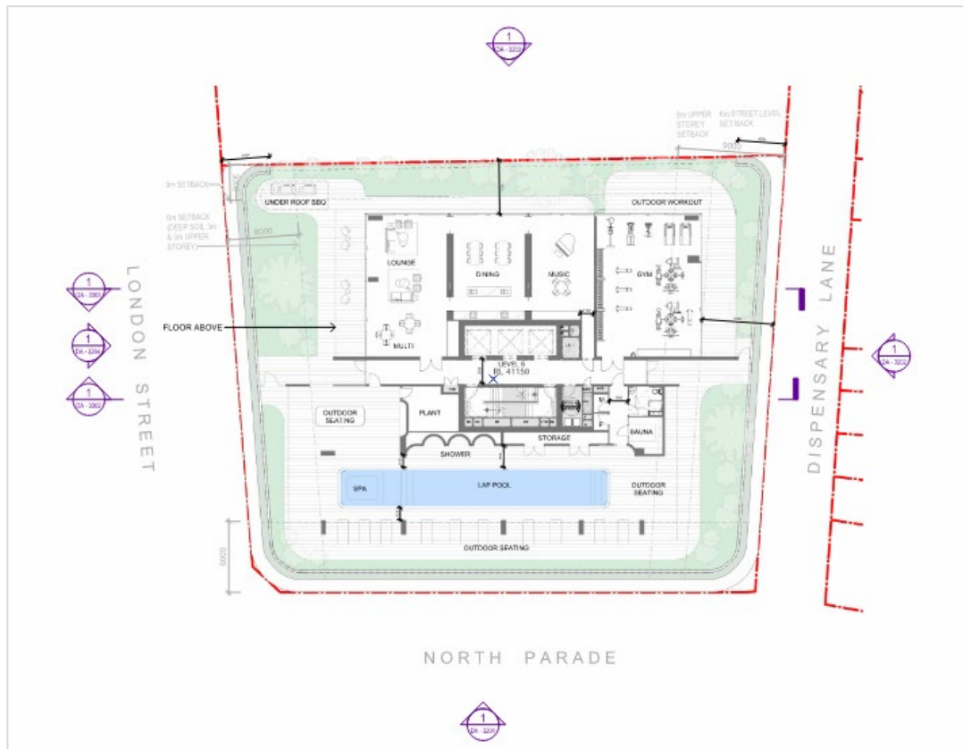
Figure 2.6 – Level 5 plan
