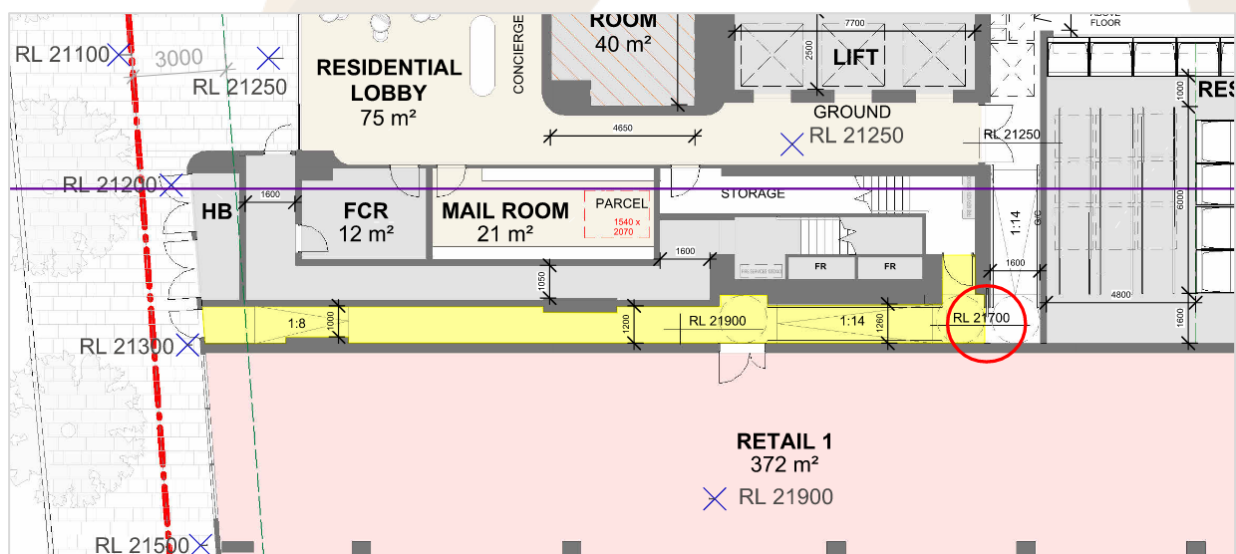
Figure 5.10 – Sliding door opening into fire isolated exit
