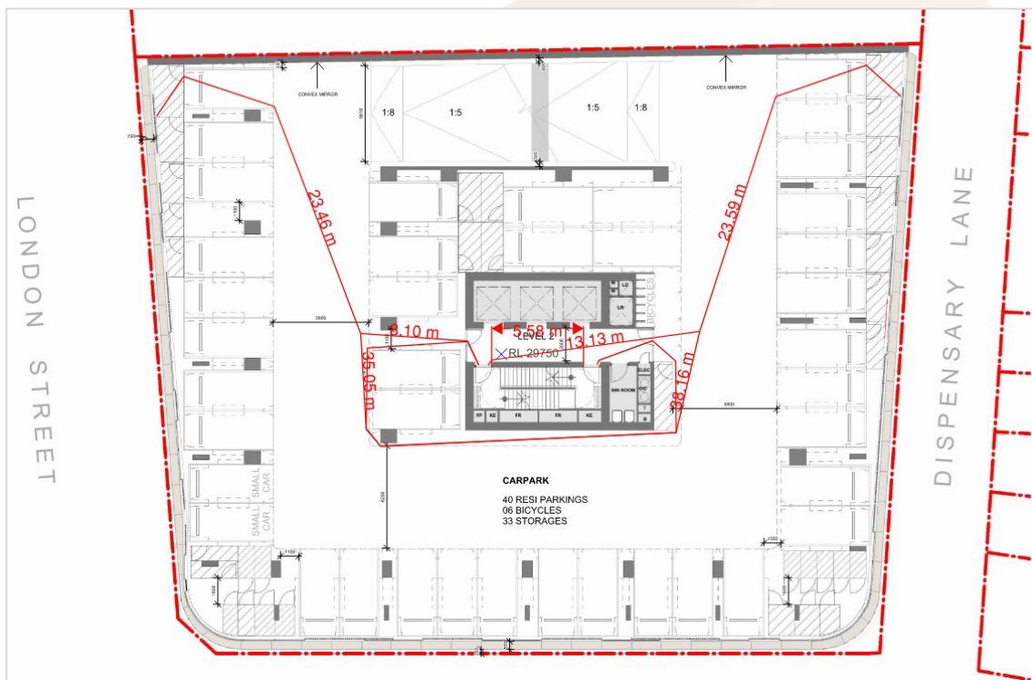
Figure 5.3 – Level 2 exit travel distances
