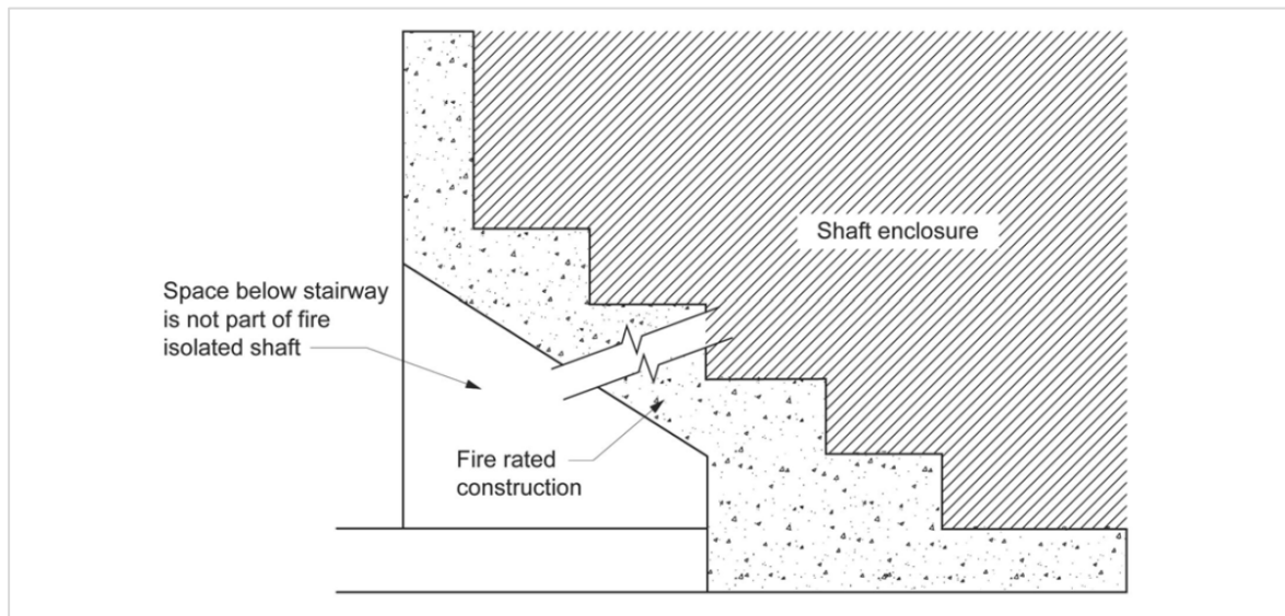
Figure 5.8 – Section showing enclosure of space below fire isolated stairway
