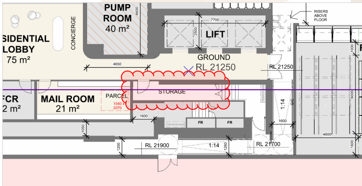
Figure 5.9 – Storage room below fire isolated stairway
