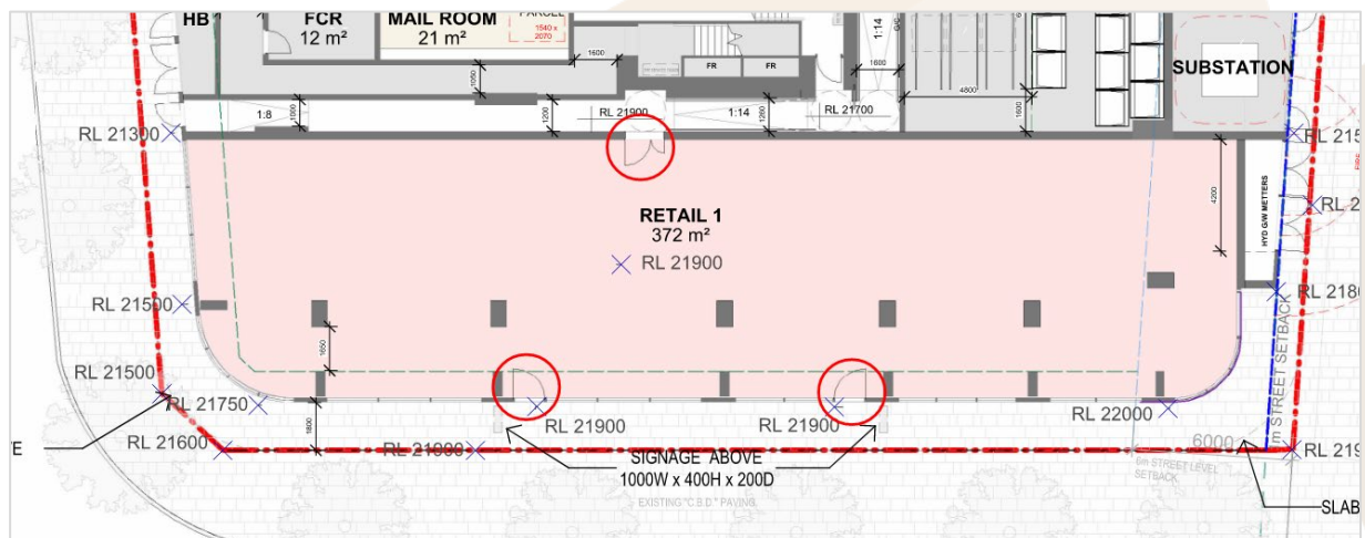
Figure 5.11 – Direction of swing to doors serving Retail 1
