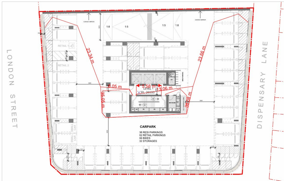
Figure 5.2 – Level 1 exit travel distances
