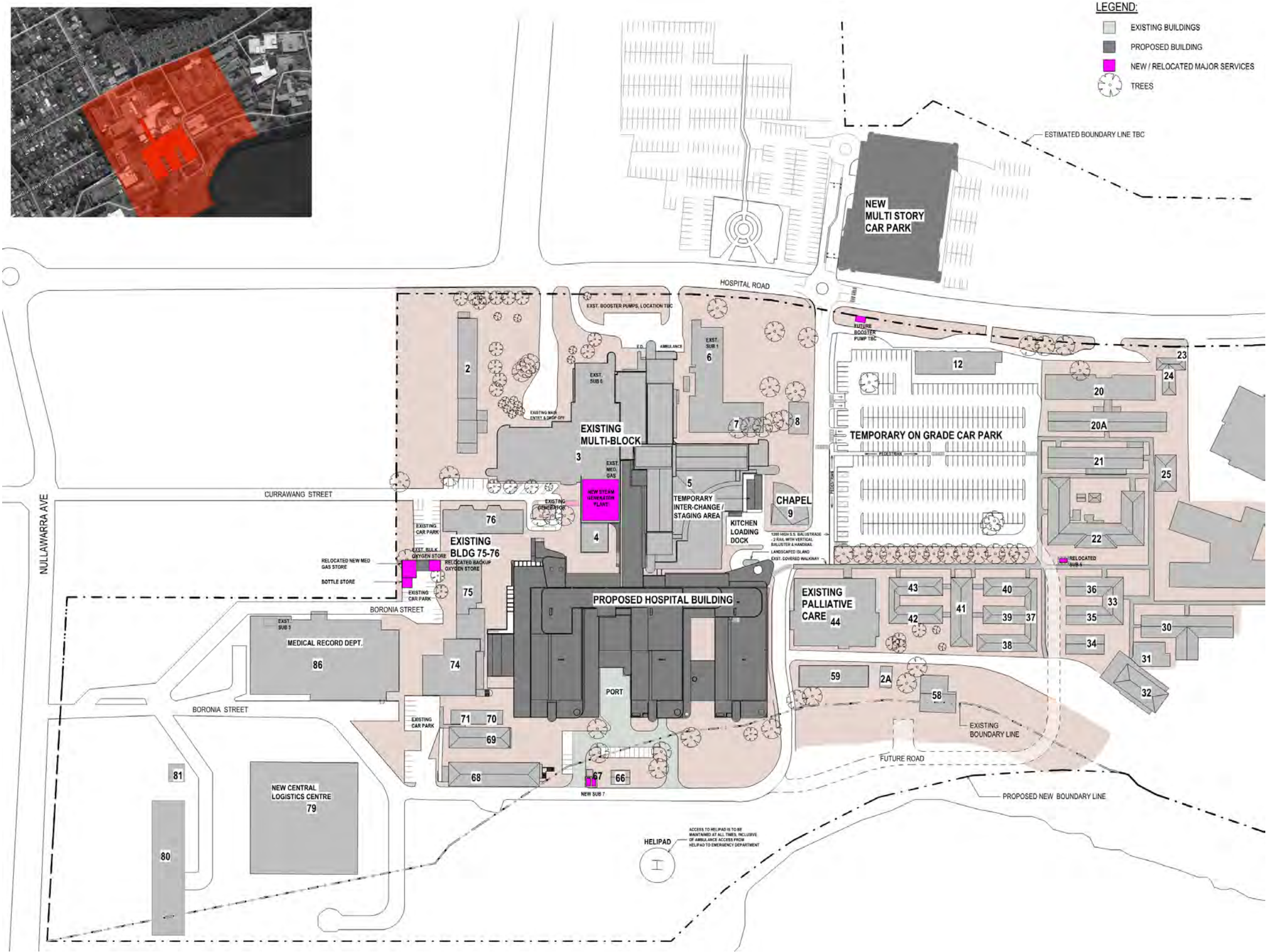
Figure 5 – Site Plan
