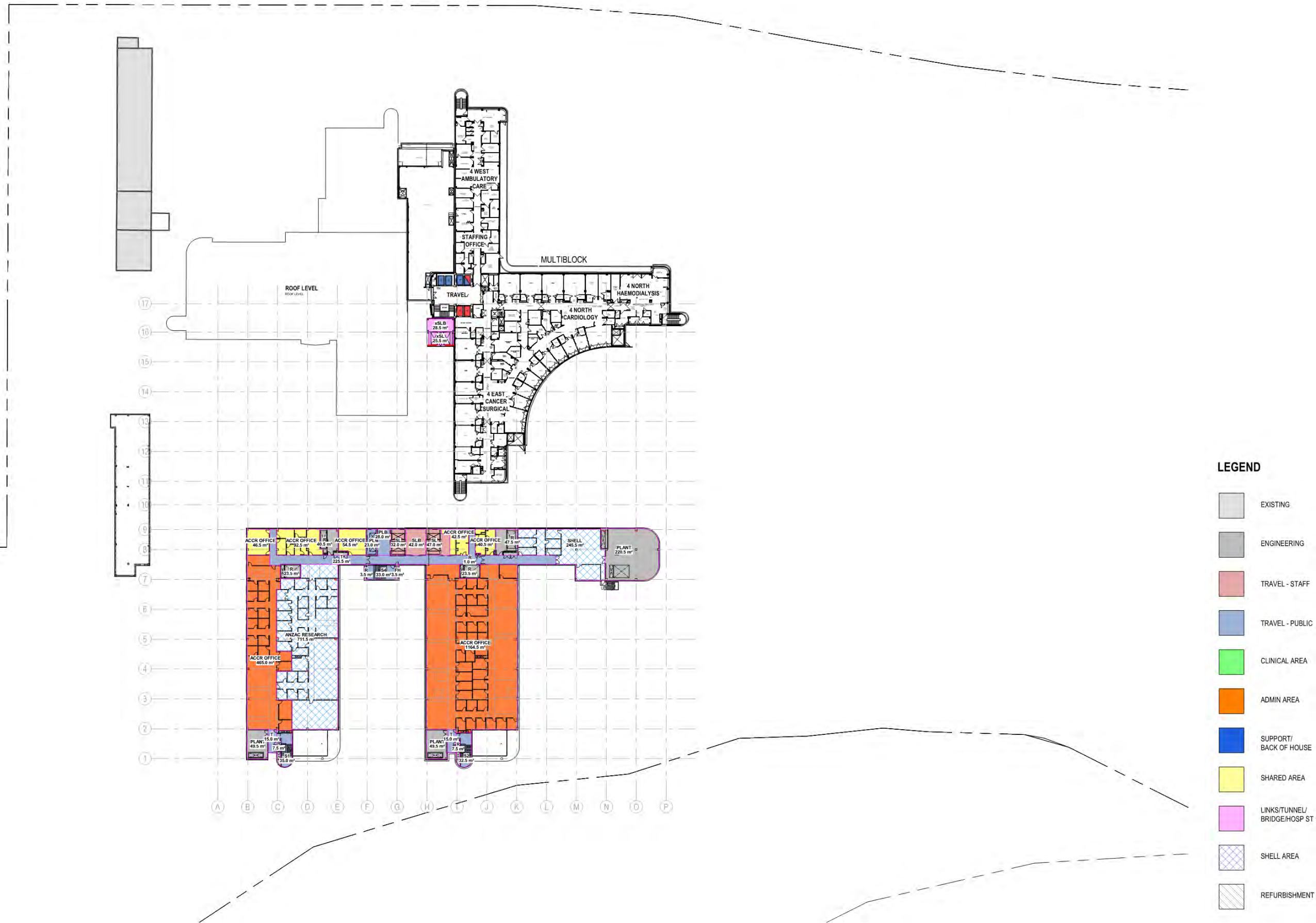
Figure 12 – Level 4 Plan
