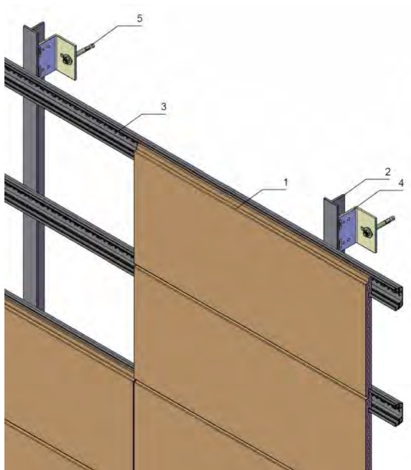
Figure 22 – Terracotta rainscreen façade system
