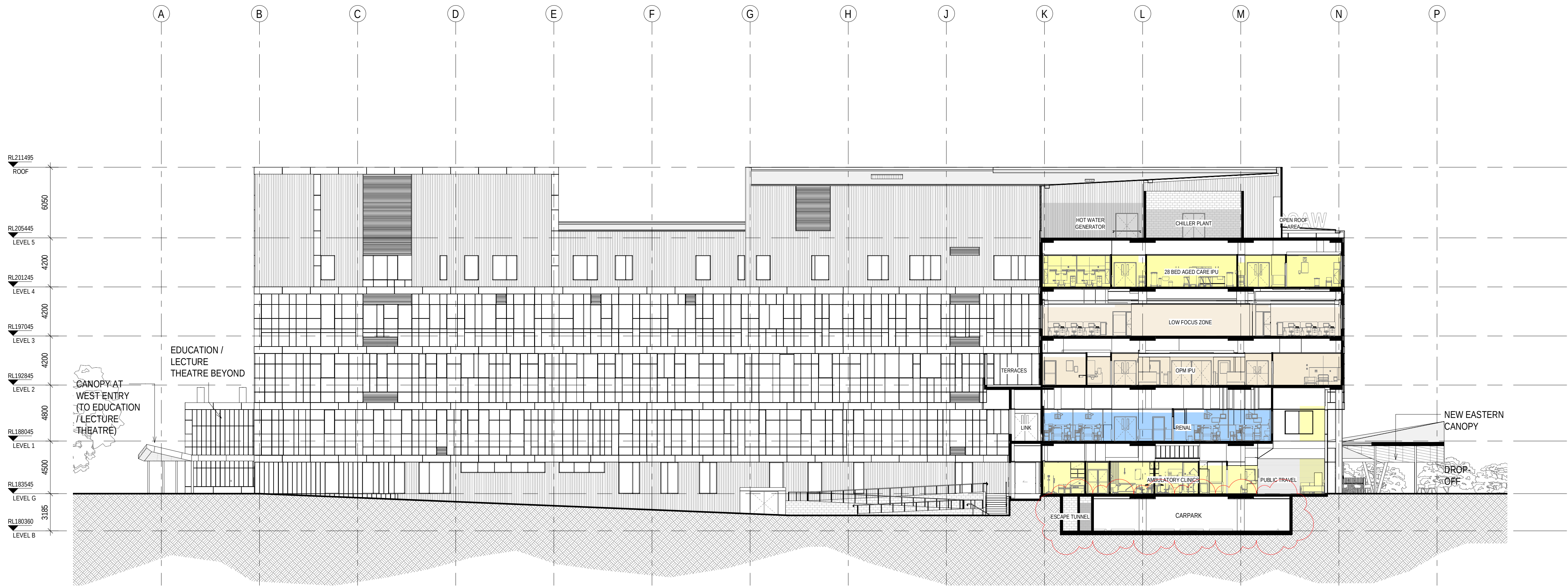
2 SECTION E-W LOOKING NORTH 1500 1:200
