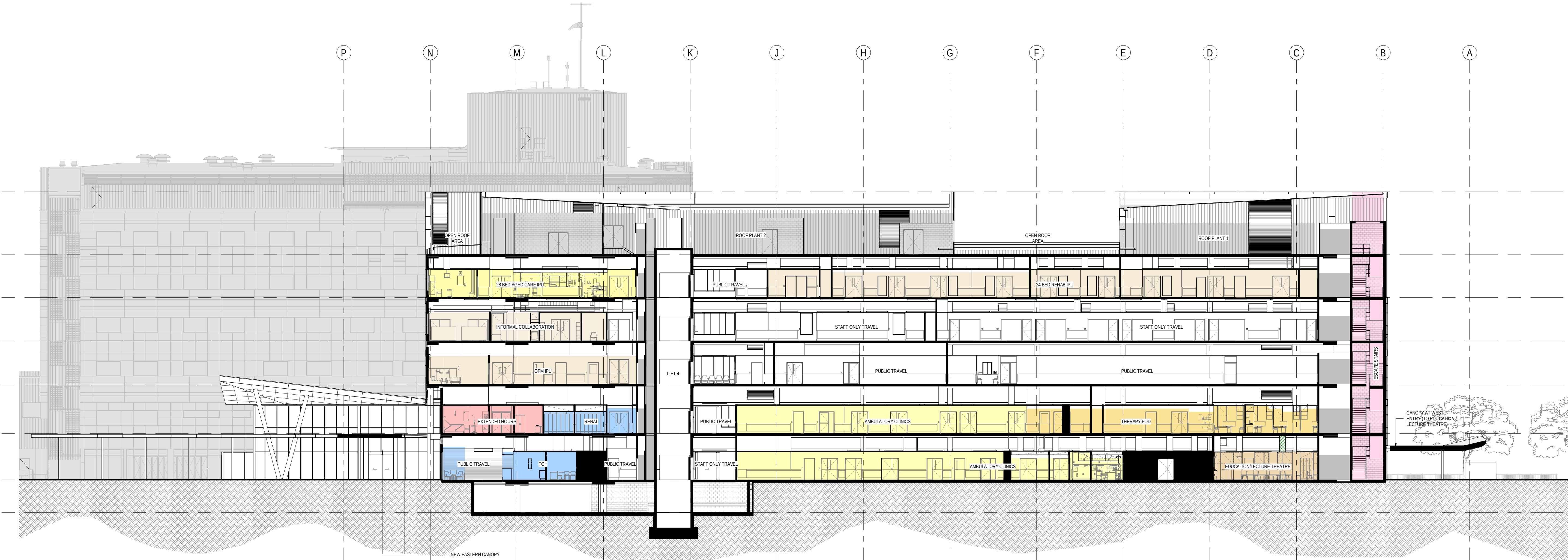
1 SECTION N-S LOOKING WEST 1500 1:200
