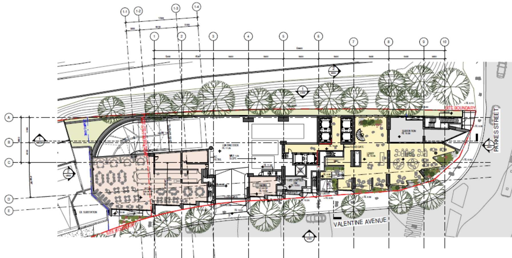
Figure 15: Proposed works – Ground Floor Plan (Source: Buchan Furtado Sullivan, December 2025, Rev C)
