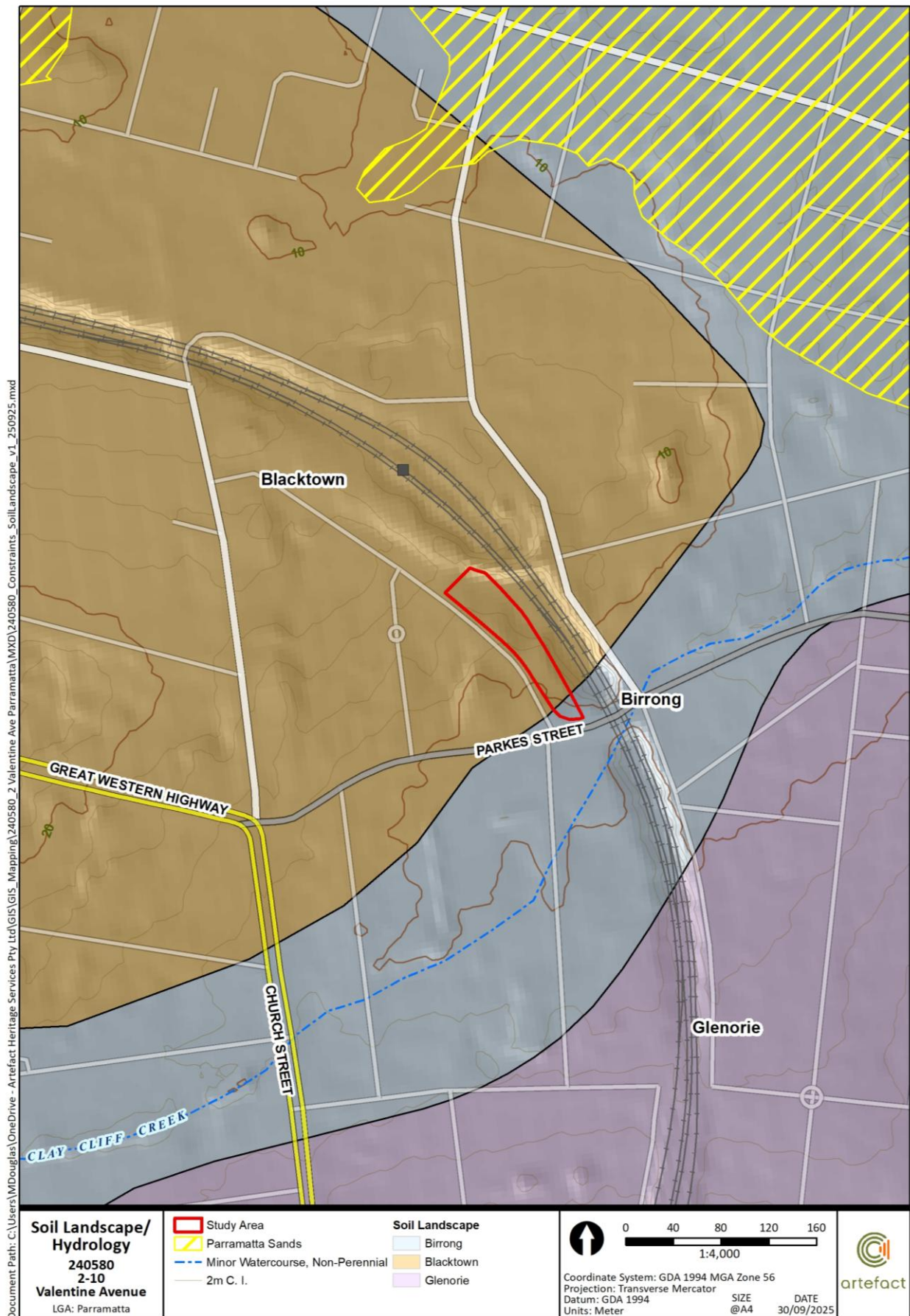
Figure 4: Soil landscape within and surrounding the study area
