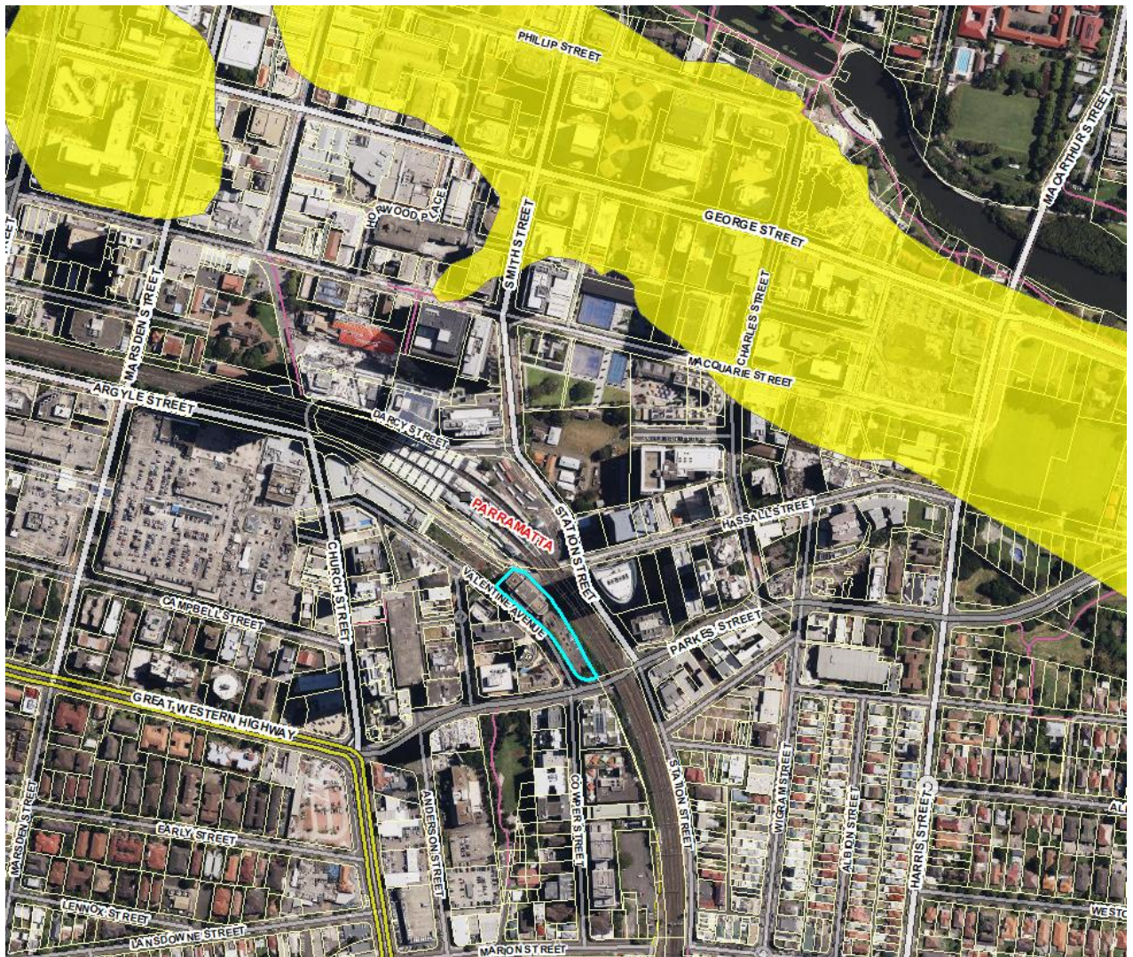
Figure 5: The study area (blue) in relation to the Parramatta Sand Body (shown in yellow)
