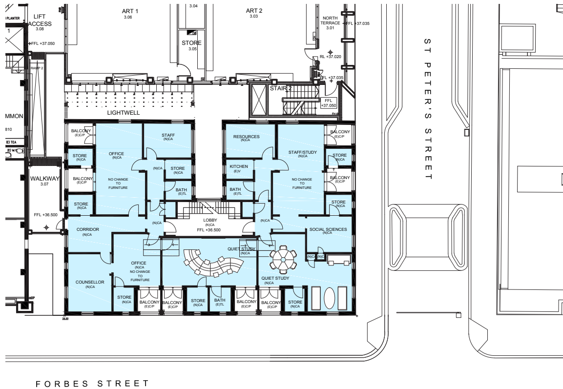
LEVEL 1
