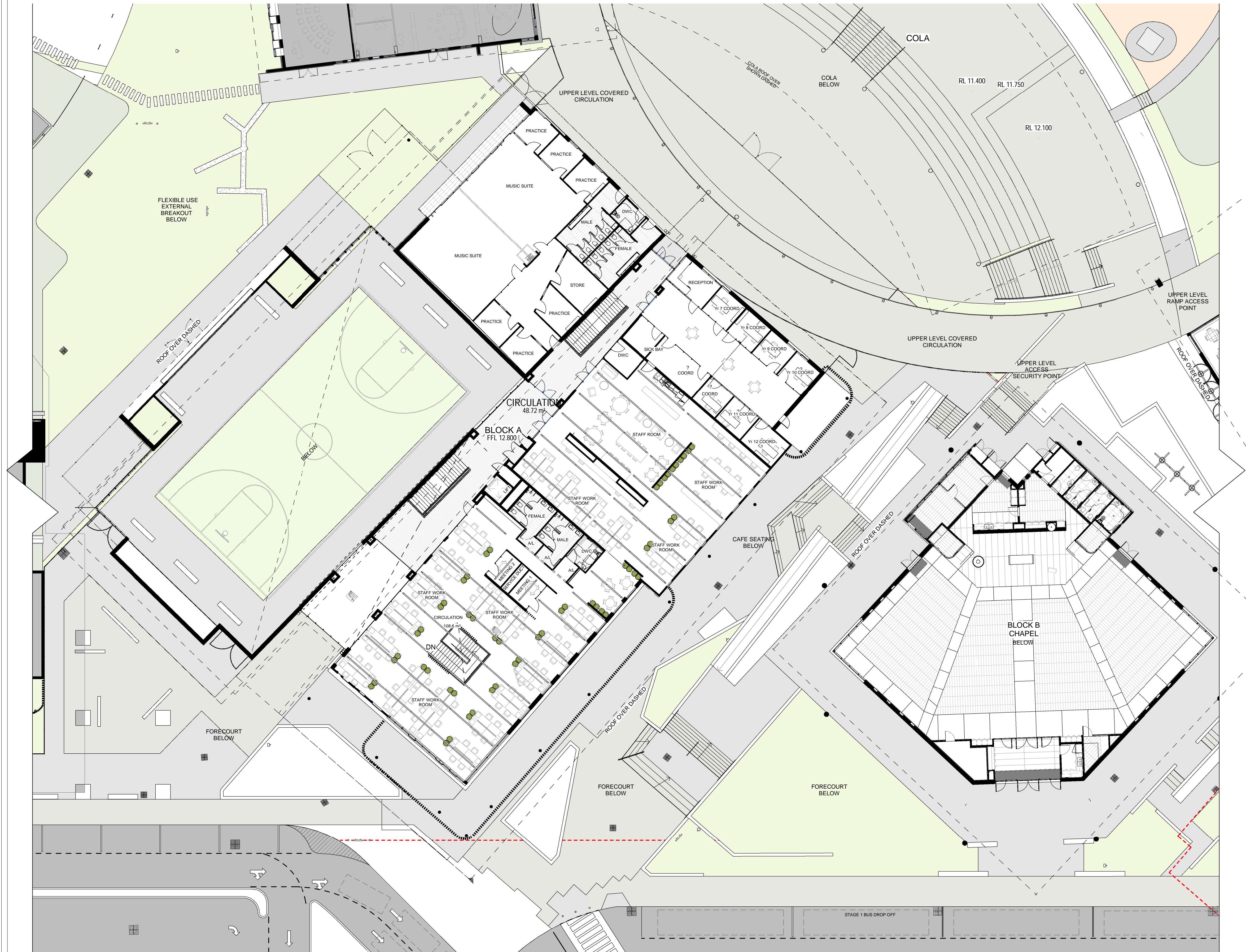
1 SITE FLOOR PLAN - LEVEL 1 - 02 04.0001 SCALE 1:200
