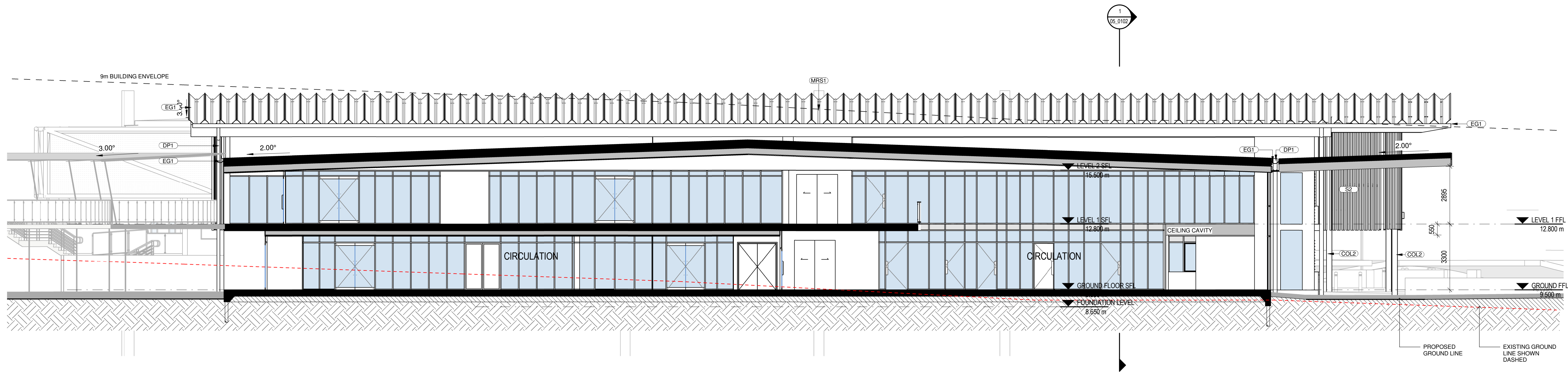
2 SECTION 4 03_0101 SCALE 1:100
