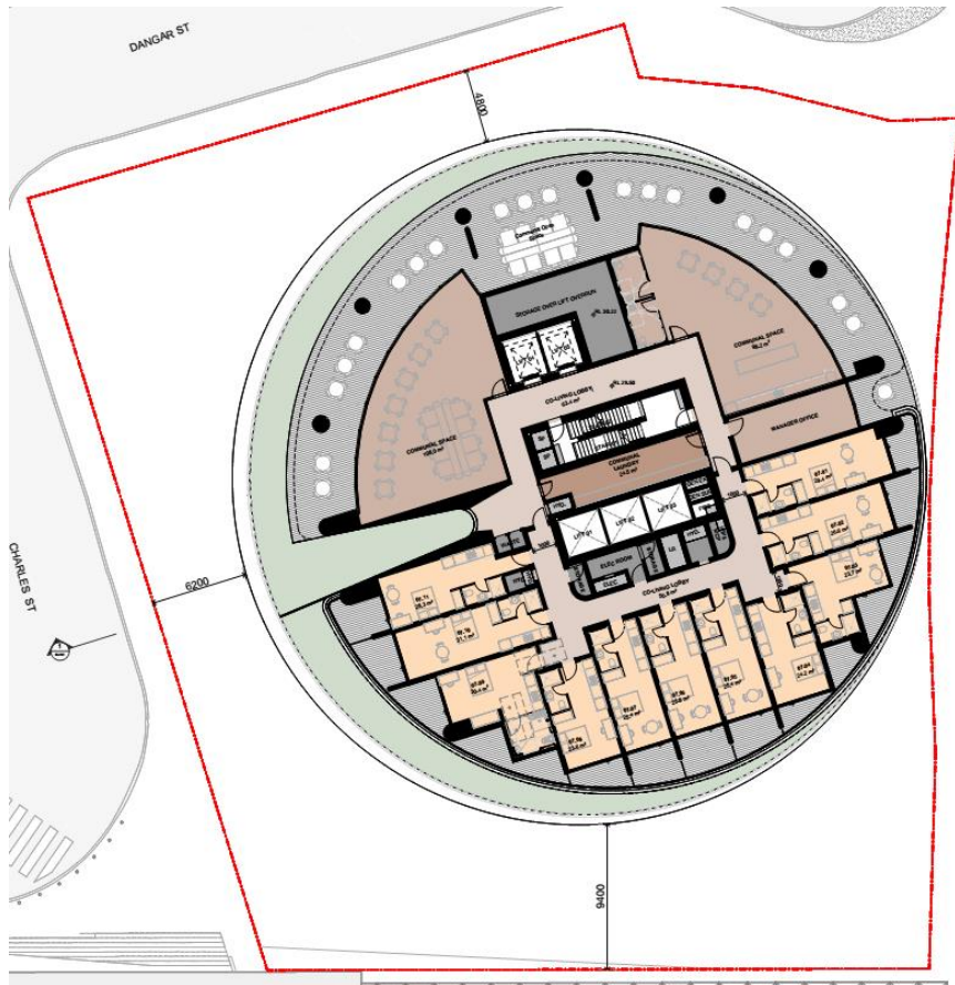
Level 07 co-living
