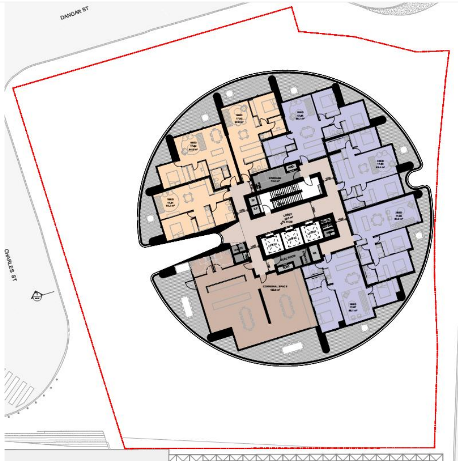
Level 17
