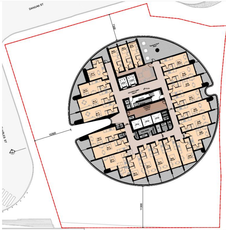
Level 08-11 co-living
