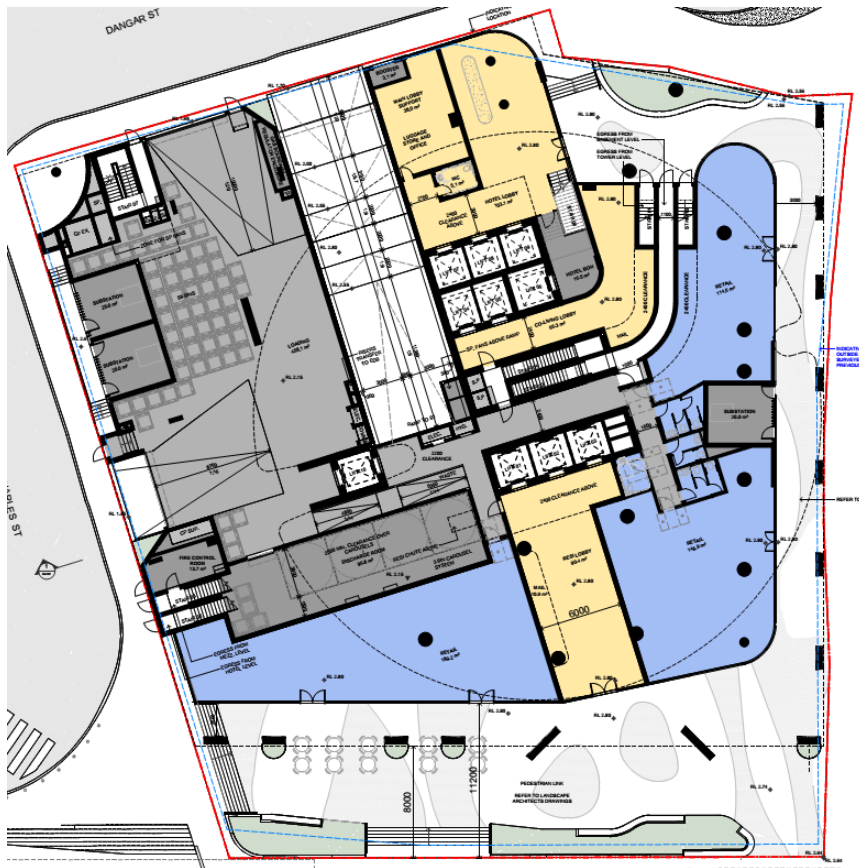
Level 00
