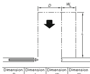
(b) Latch-side approach
