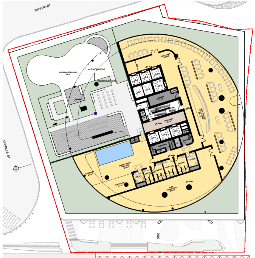
Level 06
