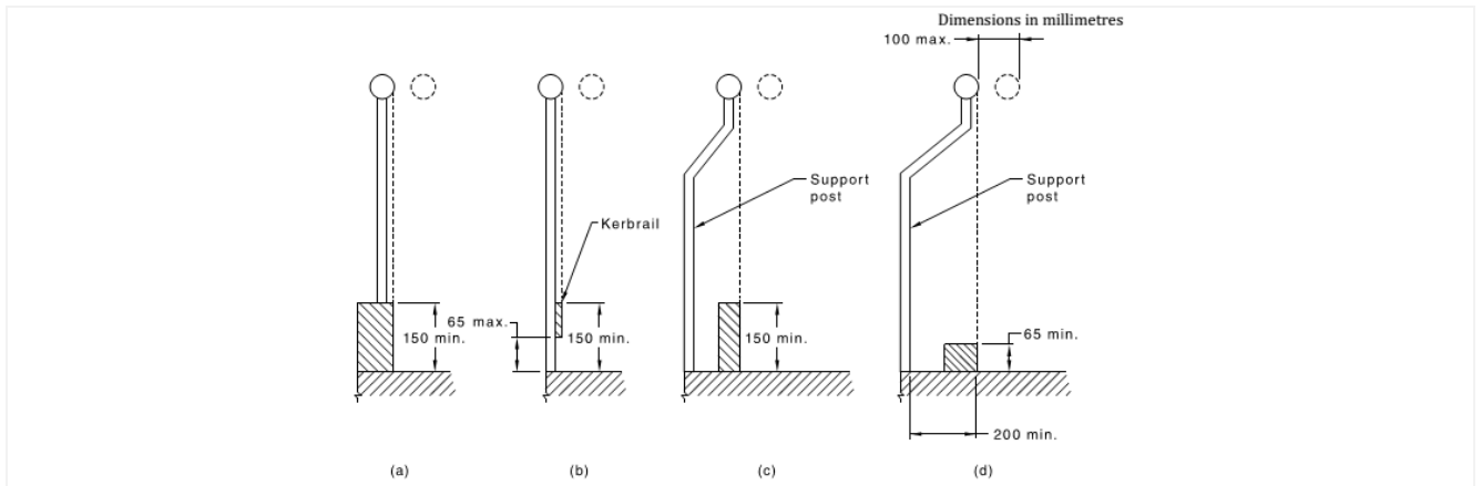
Selection showing the location of the kerb or kerb rail in relation to the handrail with vertical support
