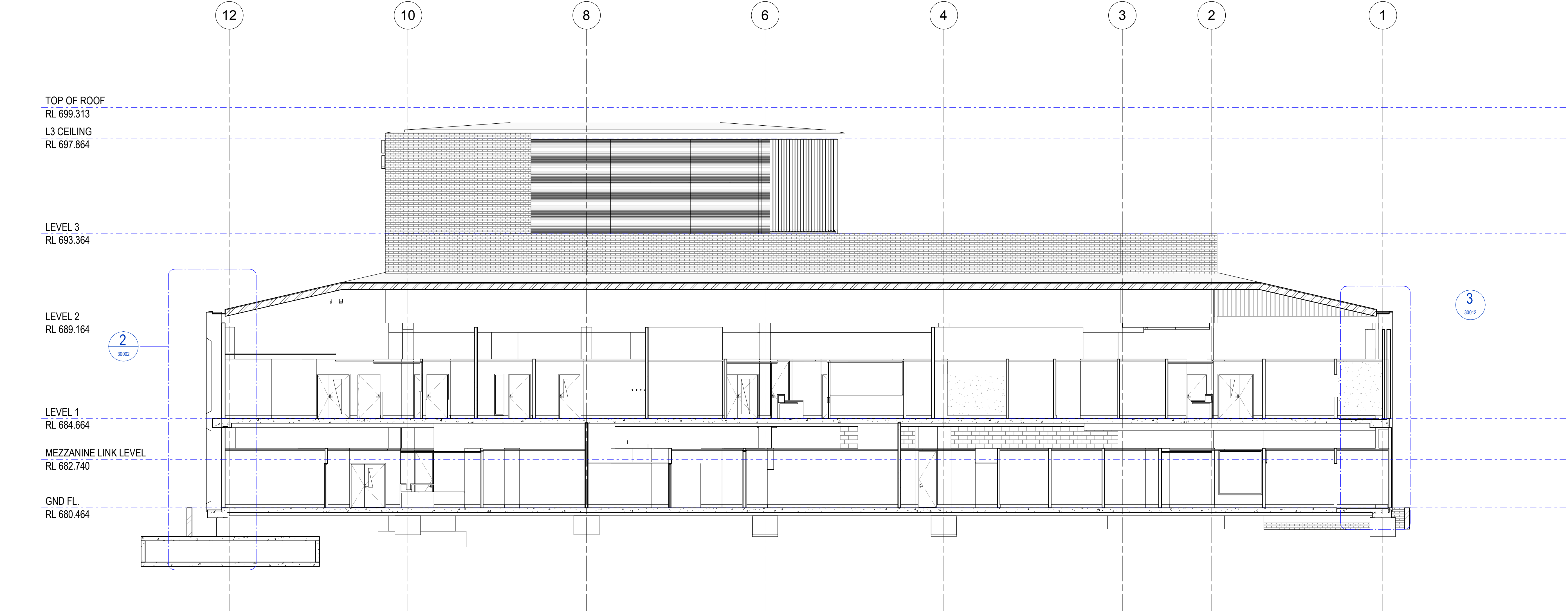
F SECTION F BETWEEN GRIDS B & C 1:100
