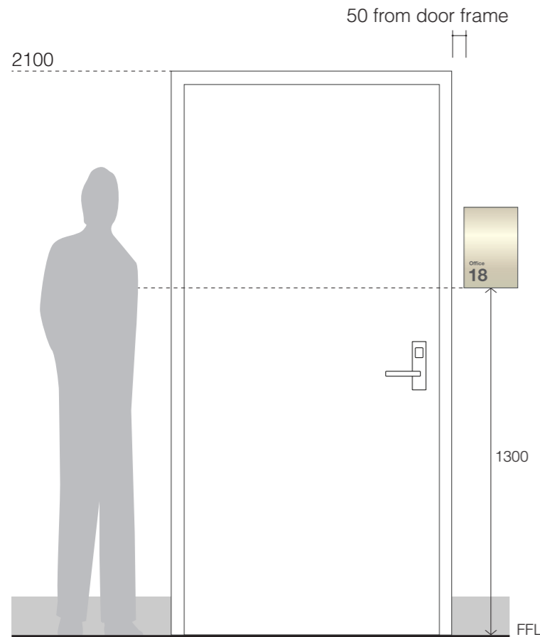
ROOM SIGNAGE Scale 1:20
