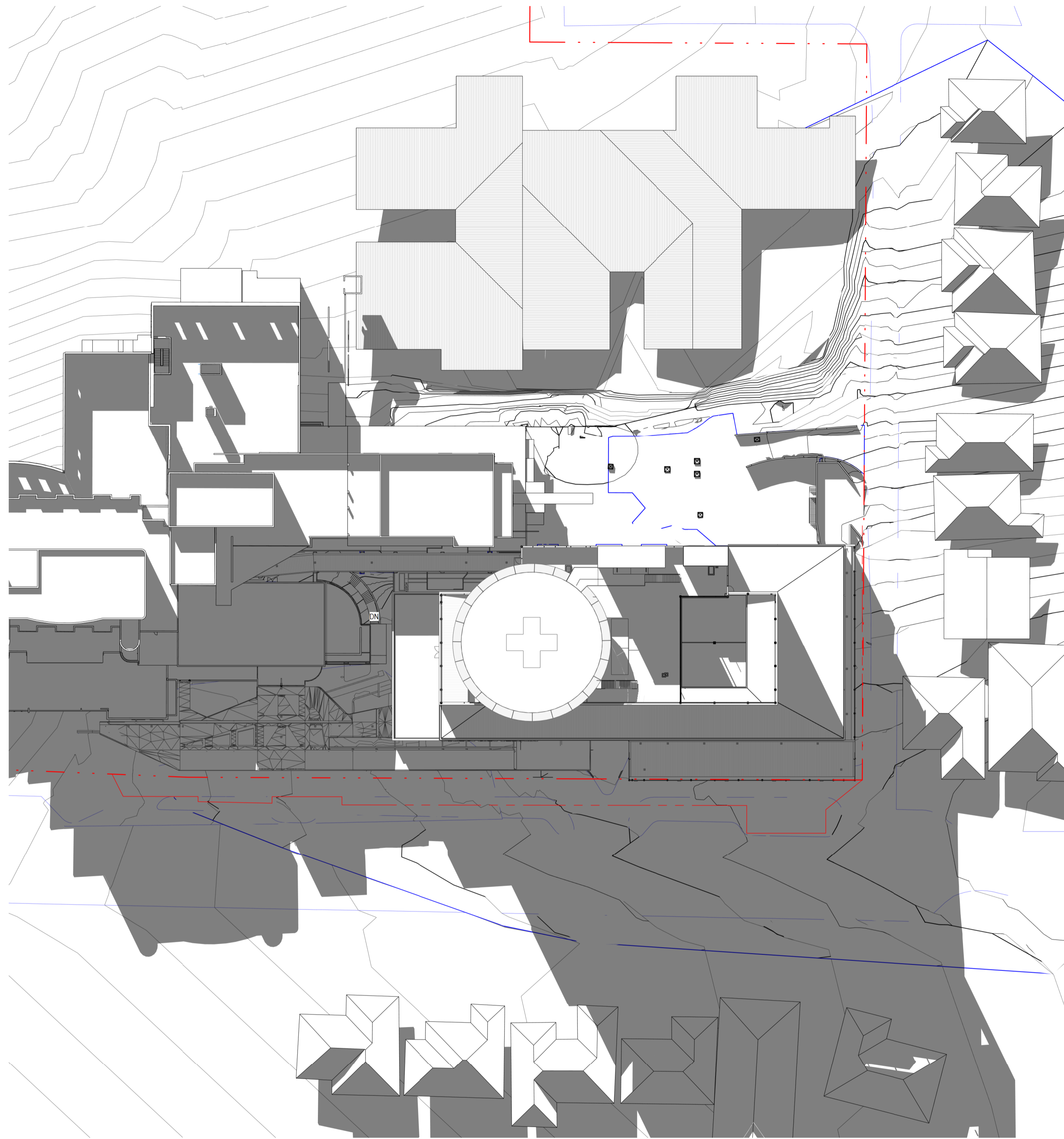
1 Sun Diagram Existing 3pm Mid Winter A30001 1 : 500
