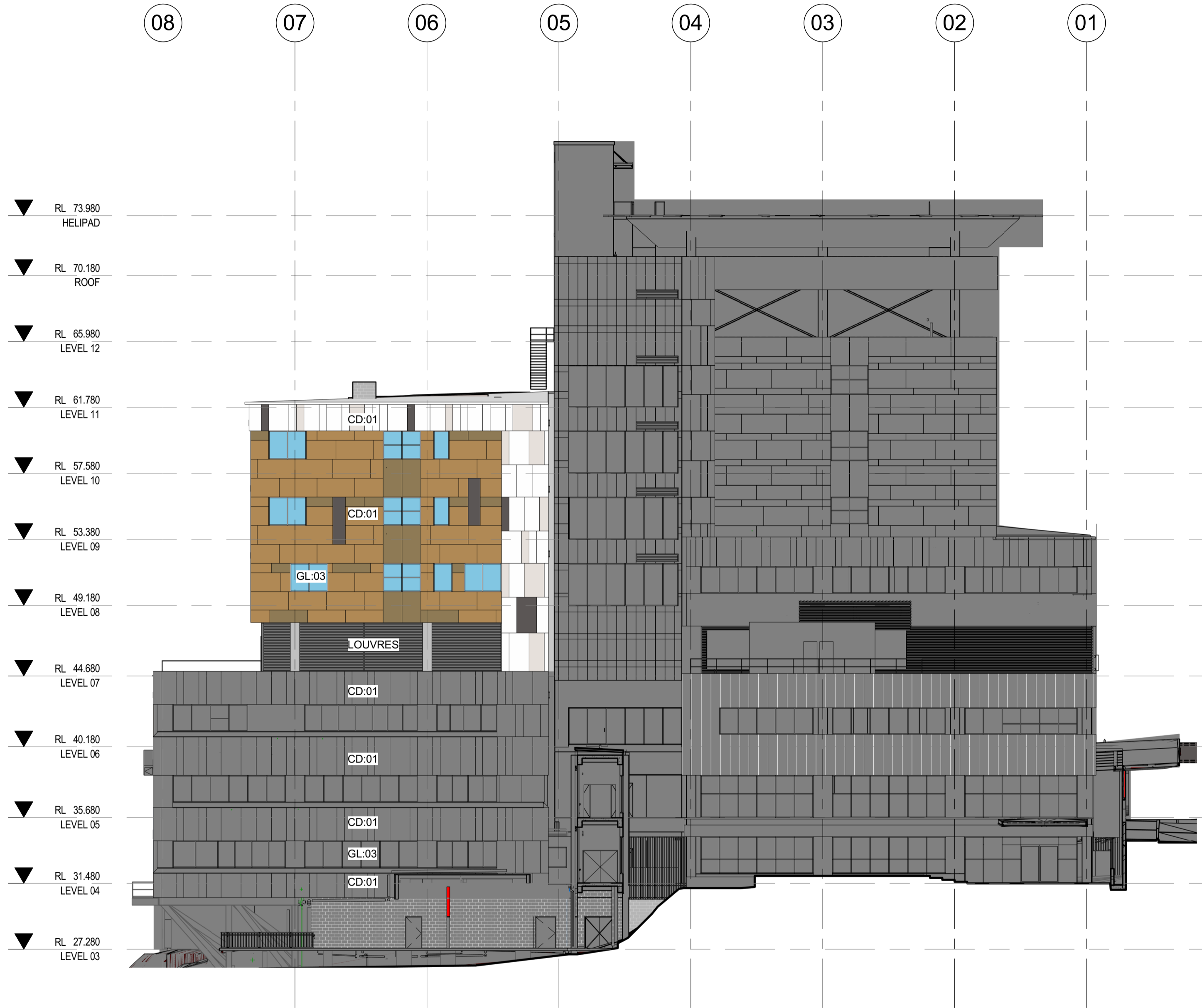
1 Building Elevation - West NTX SSDA 1:200
