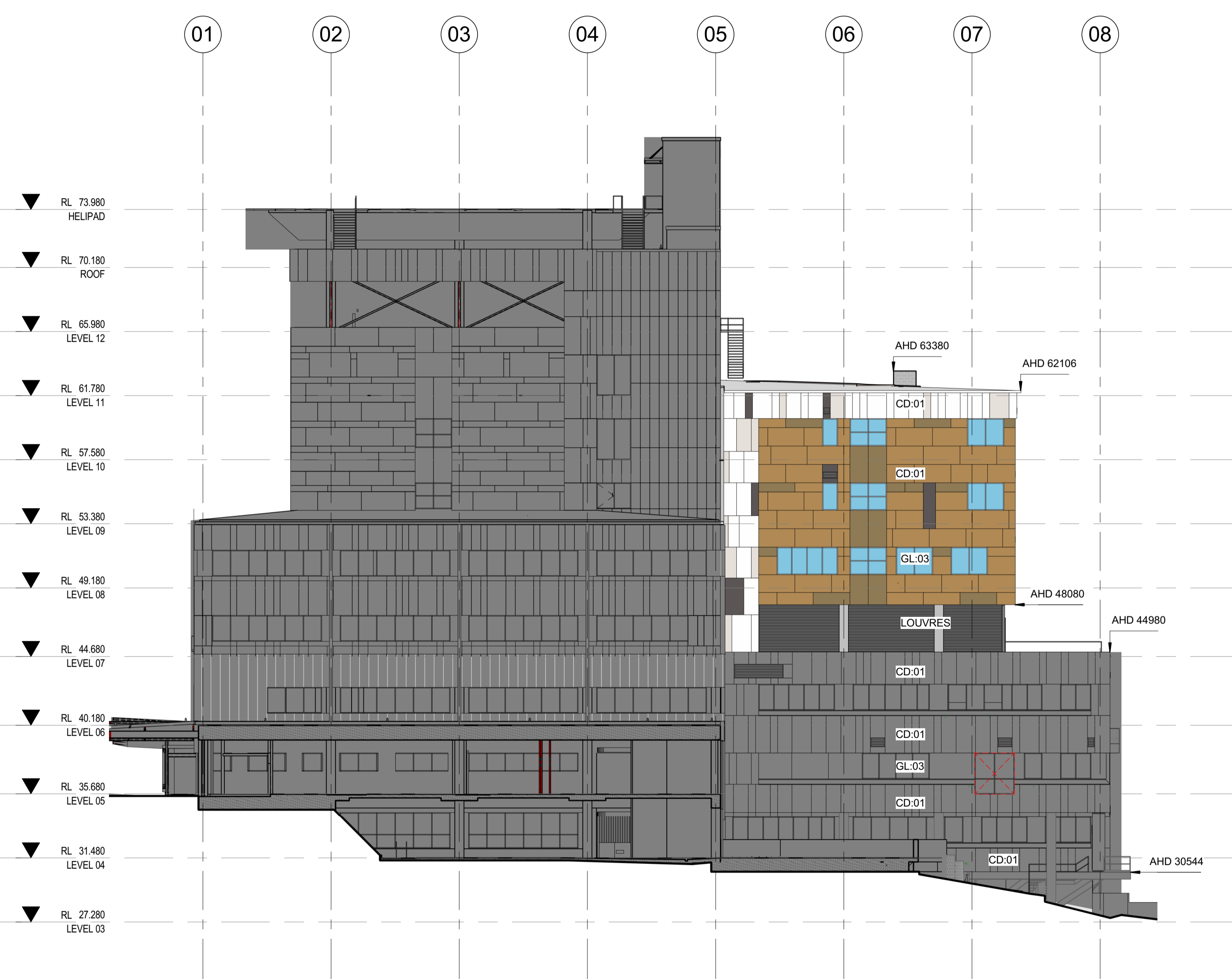
2 Building Elevation - East NTX SSDA 1:200
