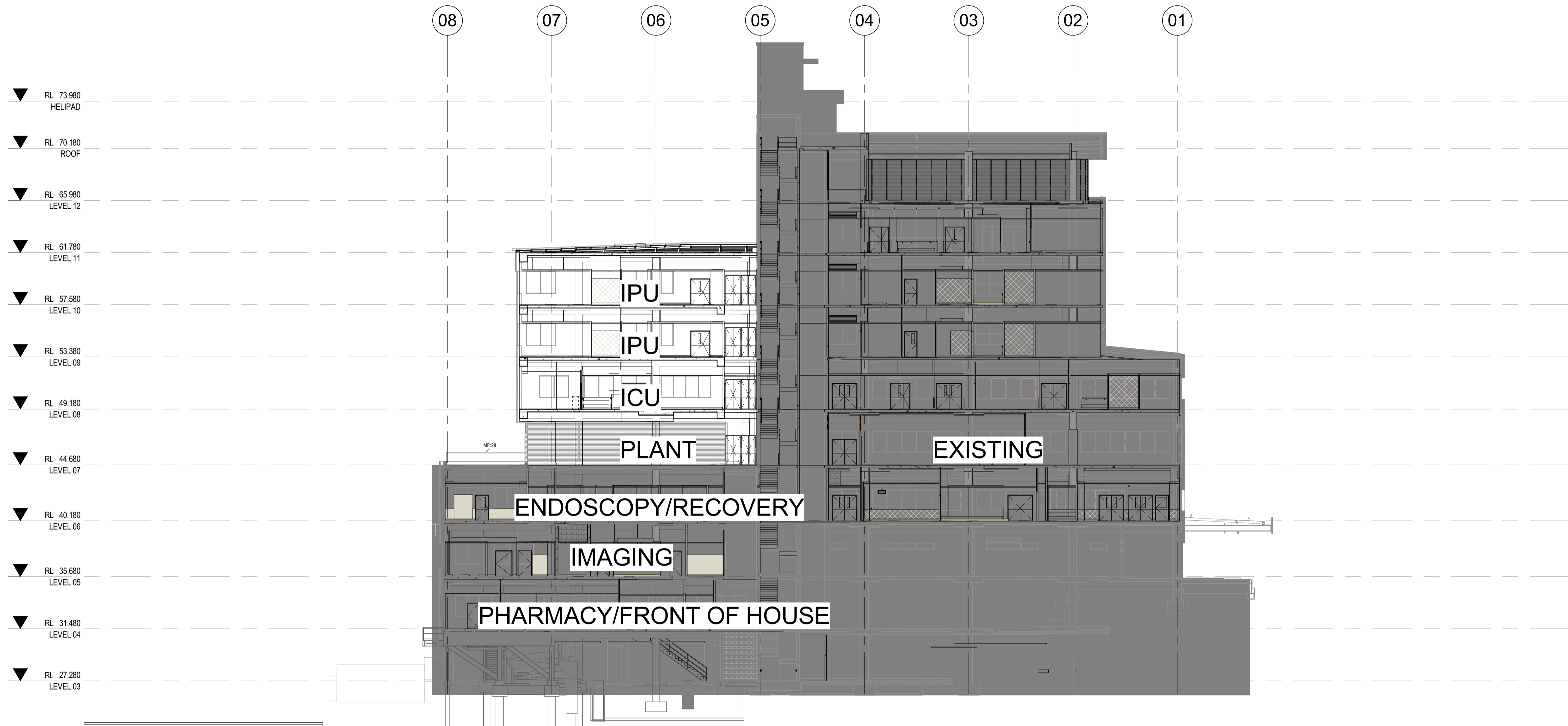
1 Overall Building Section N-S NTX SSDA A22073 1 : 200
