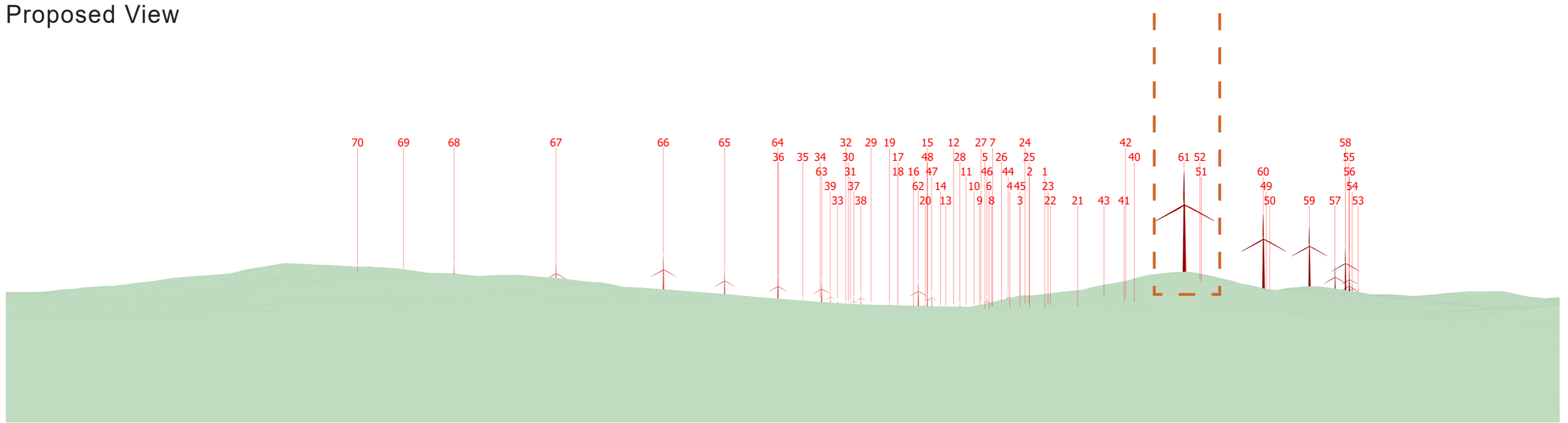
Proposed Wireframe
