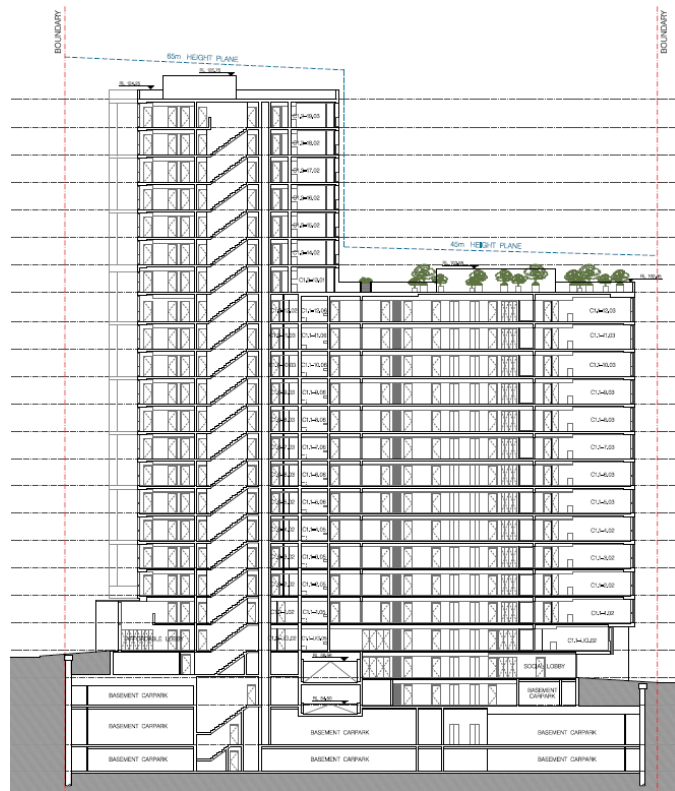
Figure 5 – Tower 1 Section and height plane controls
