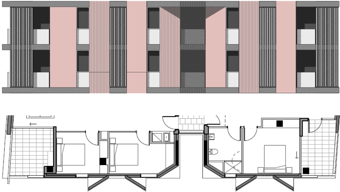
Figure 27 – South-West façade detail
