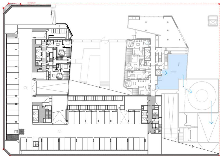
Figure 13.2 – Basement Level 1 plan showing waste strategy
