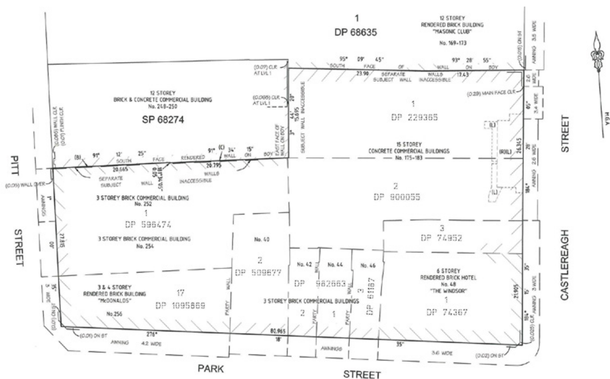
Figure 21 – Site survey
