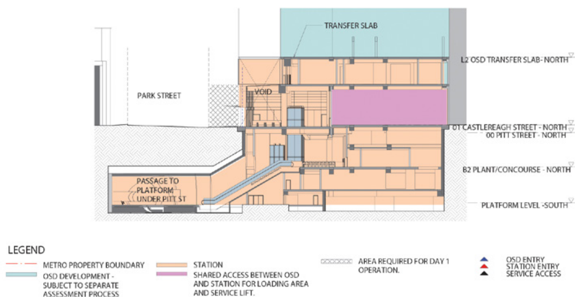
Figure 52 – Indicative interface set out under the CSSI PIR for Pitt Street North (North-South Section)
