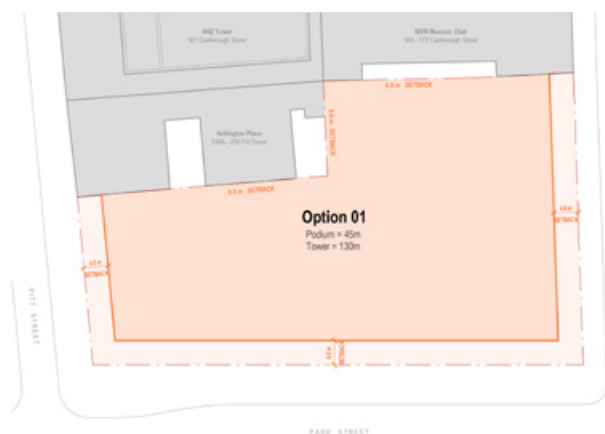
Figure 10 – Plan of Envelope Option 1
