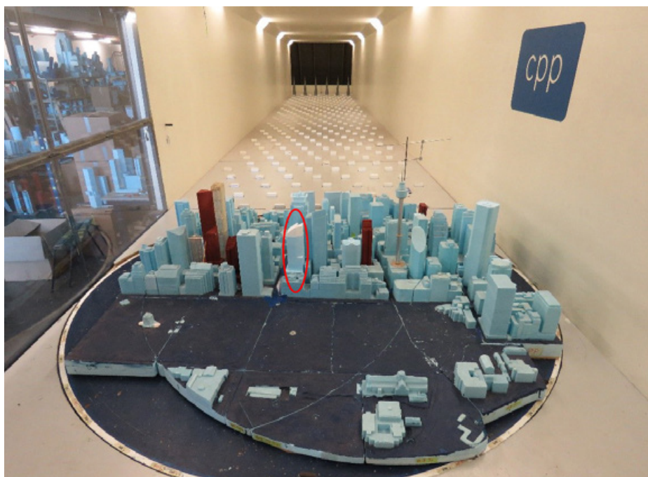
Figure 87 – Wind tunnel testing models used to determine the proposed wind impact (site in red circle)
