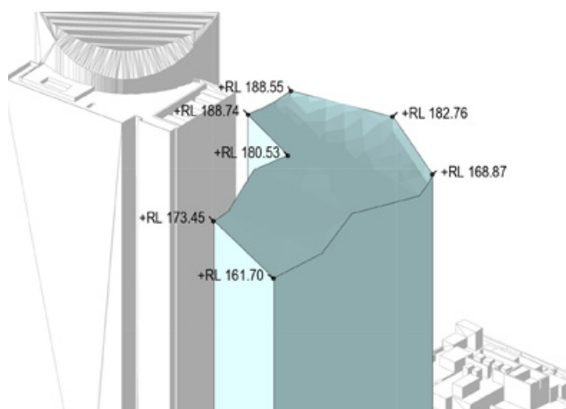
Figure 18 – Tapered envelope design at the highest extent of Option 4
